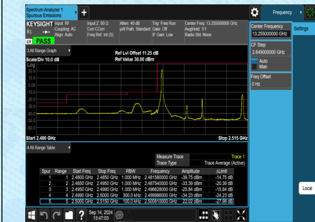
Band7-15MHz-QPSK-20825-1RB#0-PASS
