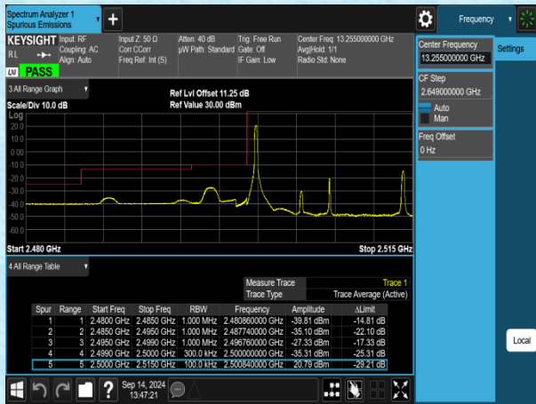
Band7-15MHz-16QAM-20825-1RB#0-PASS
