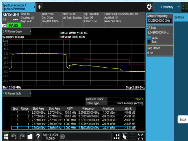
Band7-20MHz-QPSK-21350-100RB#0-PASS
