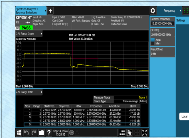
Band7-10MHz-QPSK-21400-50RB#0-PASS
