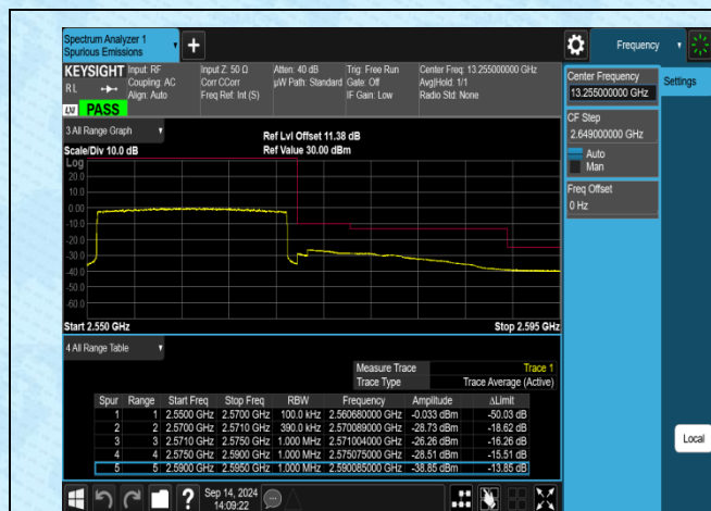
Band7-20MHz-16QAM-21350-100RB#0-PASS
