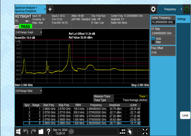
Band7-10MHz-16QAM-21400-1RB#49-PASS
