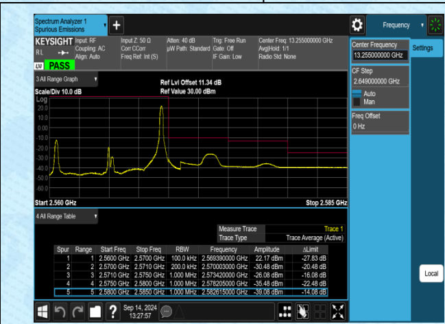
Band7-10MHz-QPSK-21400-1RB#49-PASS
