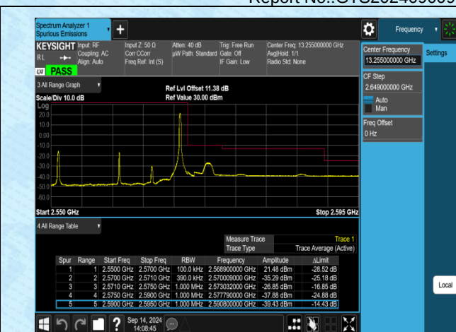
Band7-20MHz-16QAM-21350-1RB#99-PASS
