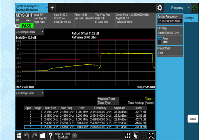
Band7-15MHz-QPSK-20825-75RB#0-PASS
