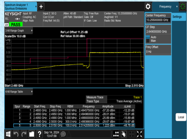
Band7-15MHz-16QAM-20825-75RB#0-PASS
