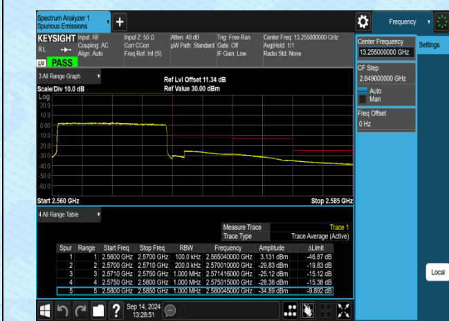
Band7-10MHz-16QAM-21400-50RB#0-PASS
