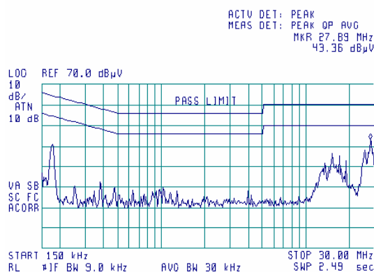
Plot 9.1.6 Conducted emission measurements
