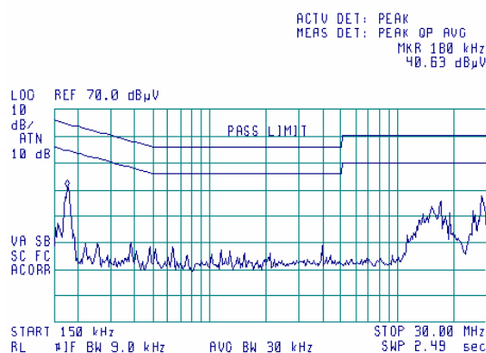
Plot 9.1.4 Conducted emission measurements
