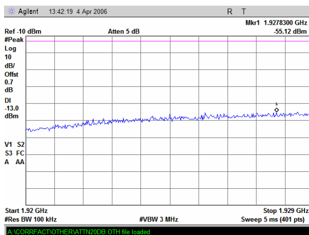
Plot 8.3.36 Spurious emission measurements in 1.920 – 1.929 GHz range, PCS 1900, TDMA modulation
