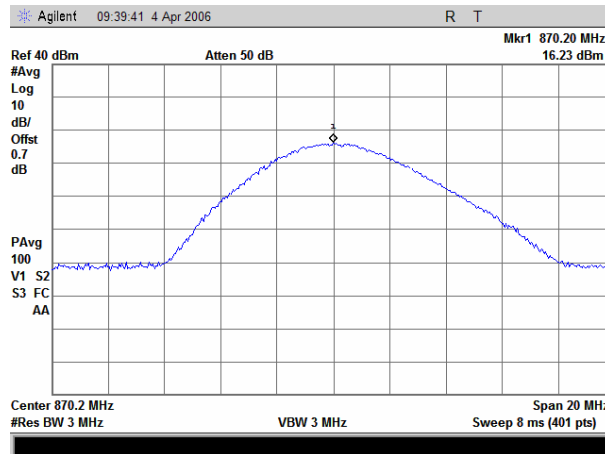
Plot 7.1.11 RF output power measurements at low frequency carrier, Cell 800, CDMA modulation
