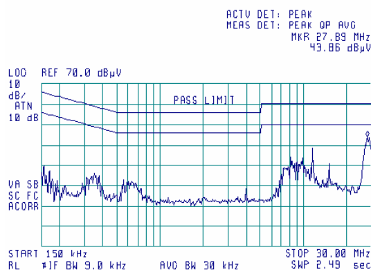
Plot 9.1.12 Conducted emission measurements
