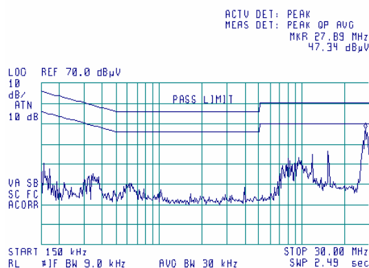
Plot 9.1.8 Conducted emission measurements
