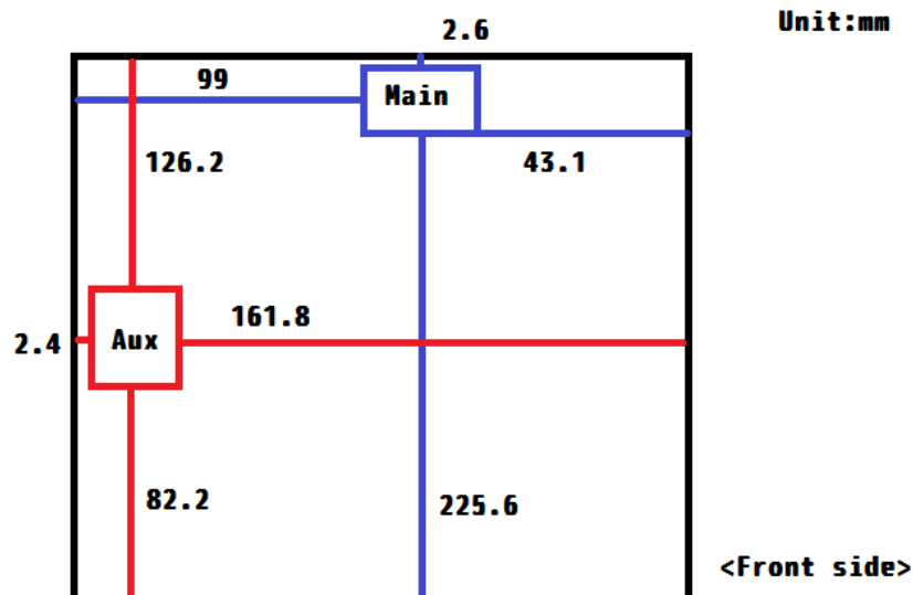
Fig.10 Antenna position of EUT
