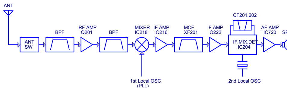
Fig.3 Receiver Section Configuration
