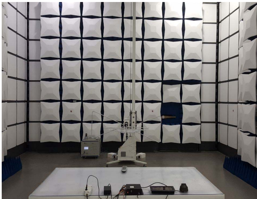
Radiated Emission
