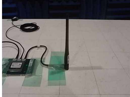
Sub Antenna
