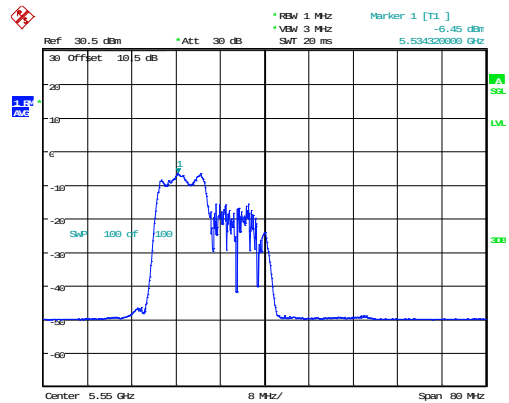
802.11ax40_5550MHz_RU_106/53
