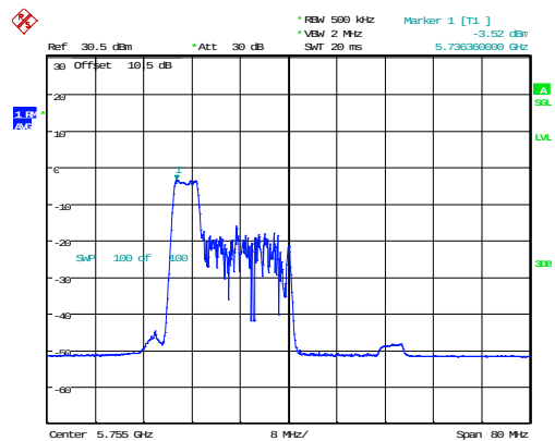
802.11ax40_5755MHz_RU_52/37
