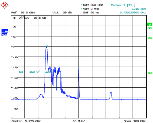
802.11ax80_5775MHz_RU_26/0
