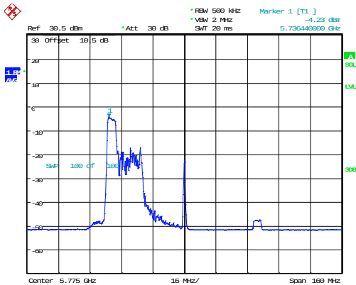
802.11ax80_5775MHz_RU_52/37
