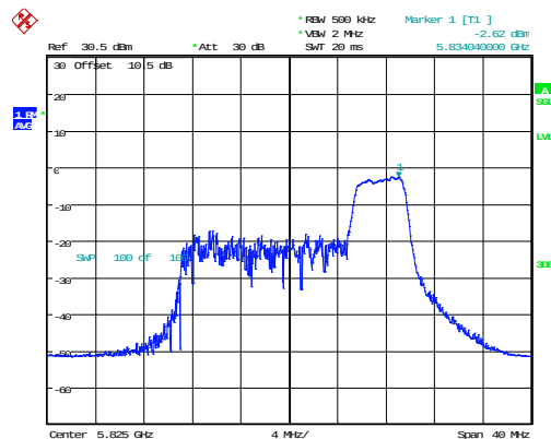
802.11ax20_5825MHz_RU_52/40
