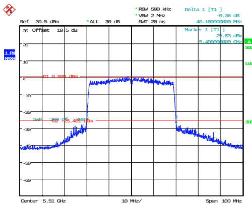
802.11ax40_5510MHz_RU_Full
