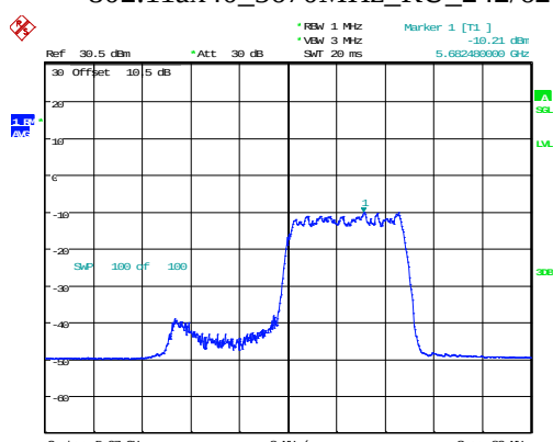
802.11ax40_5670MHz_RU_242/62
