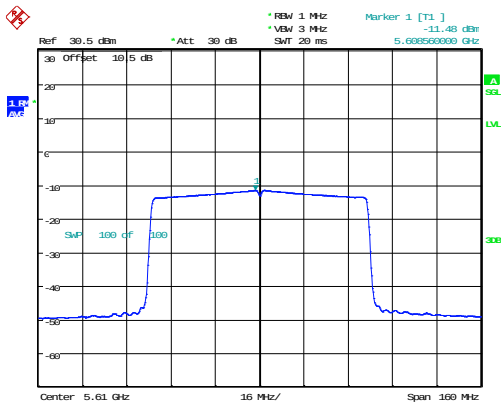
802.11ax80_5610MHz_RU_Full
