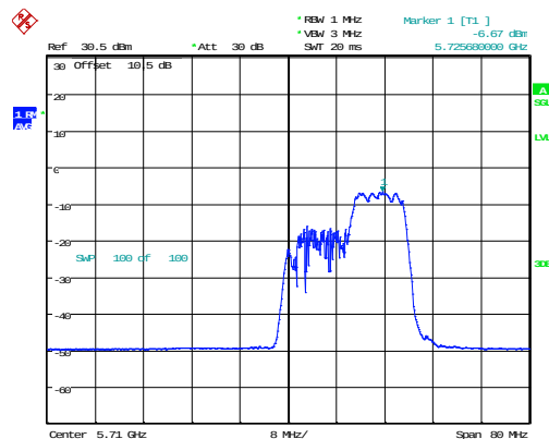
802.11ax40_5710MHz_RU_106/56
