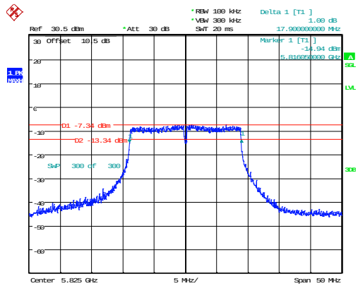
802.11n20_5825MHz
