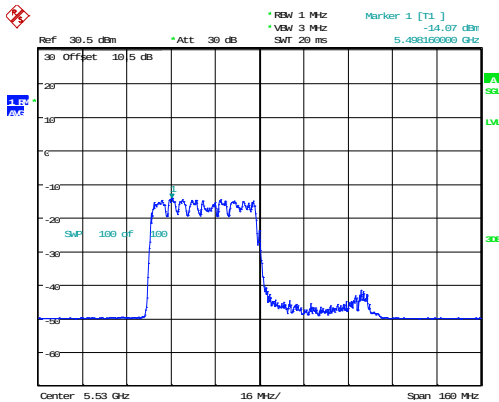
802.11ax80_5530MHz_RU_484/65
