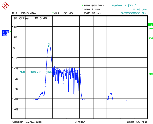
802.11ax40_5755MHz_RU_26/0
