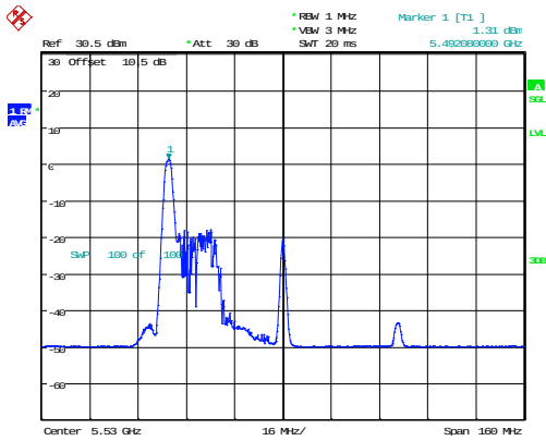
802.11ax80_5530MHz_RU_26/0
