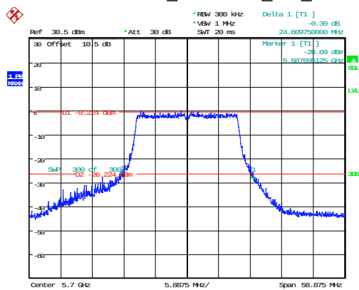
802.11ax20_5700MHz_RU_Full
