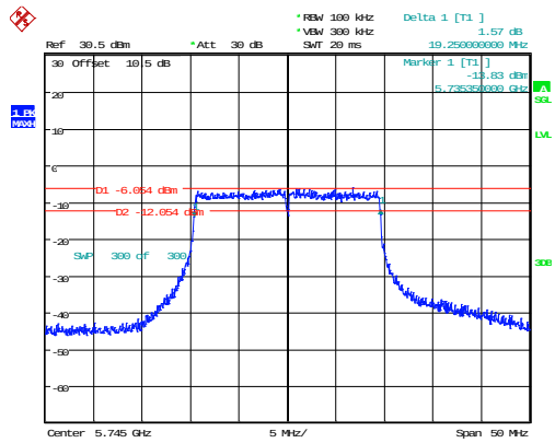
802.11ax20_5745MHz_RU_Full
