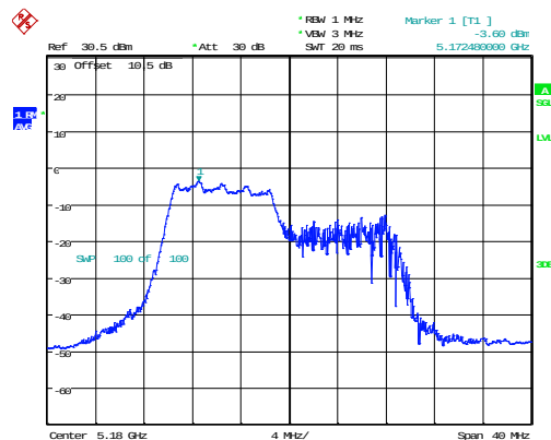
802.11ax20_5180MHz_RU_106/53
