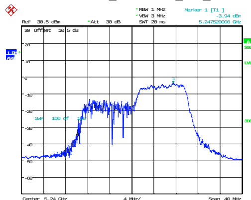
802.11ax20_5240MHz_RU_106/54
