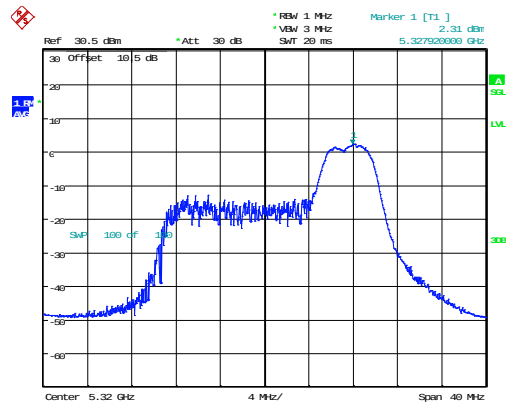
802.11ax20_5320MHz_RU_52/40
