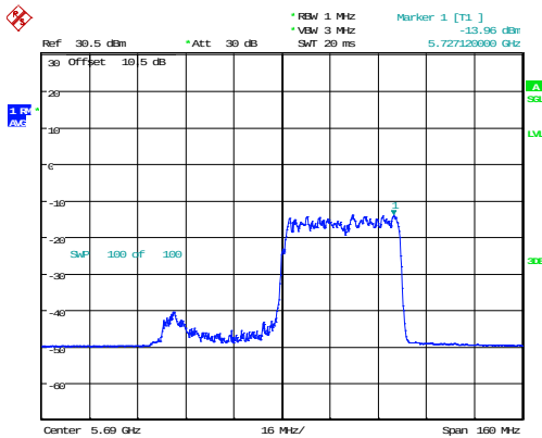
802.11ax80_5690MHz_RU_484/66
