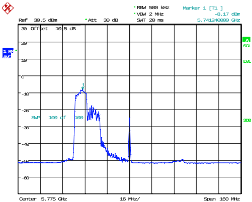
802.11ax80_5775MHz_RU_106/53
