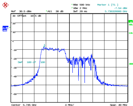
802.11ax20_5745MHz_RU_106/53
