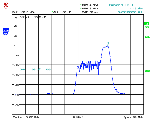
802.11ax40_5670MHz_RU_52/44
