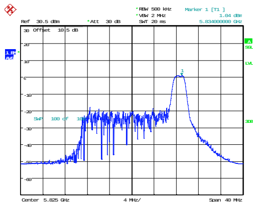
802.11ax20_5825MHz_RU_26/8
