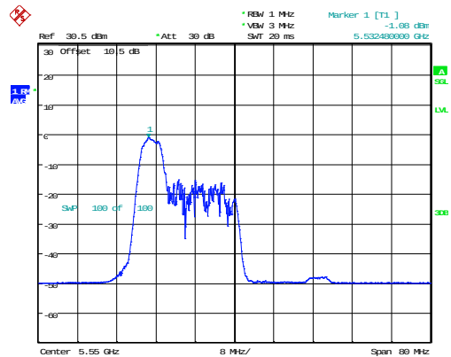
802.11ax40_5550MHz_RU_52/37
