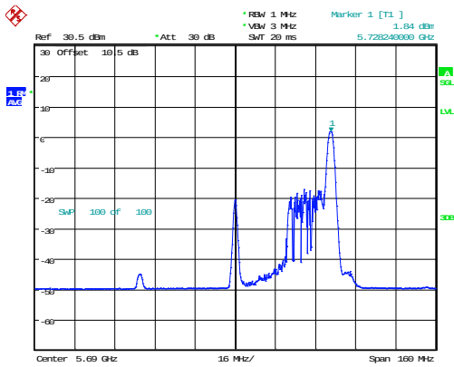
802.11ax80_5690MHz_RU_26/36
