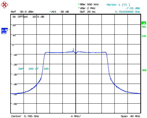
802.11ax20_5785MHz_RU_Full
