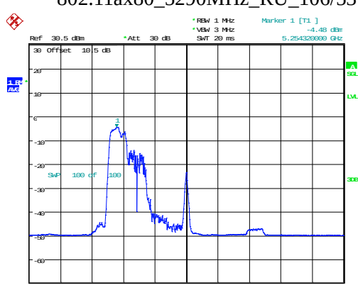
802.11ax80_5290MHz_RU_106/53
