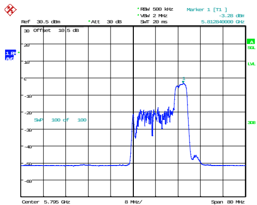
802.11ax40_5795MHz_RU_52/44
