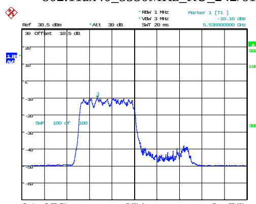
802.11ax40_5550MHz_RU_242/61
