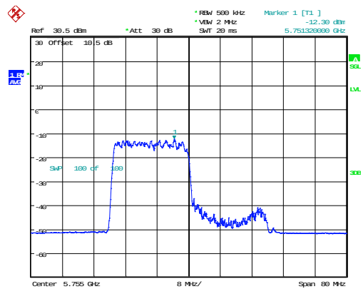
802.11ax40_5755MHz_RU_242/61
