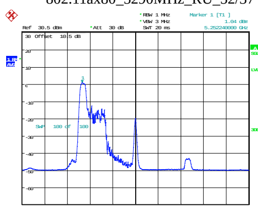
802.11ax80_5290MHz_RU_52/37
