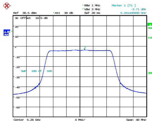
802.11ax20_5260MHz_RU_Full
