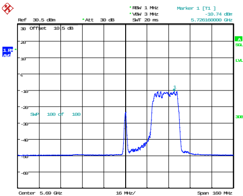
802.11ax80_5690MHz_RU_242/64
