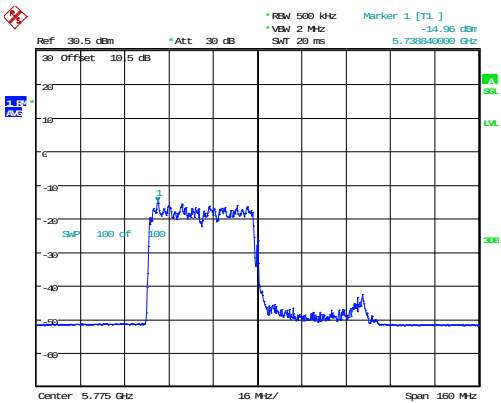
802.11ax80_5775MHz_RU_484/65
