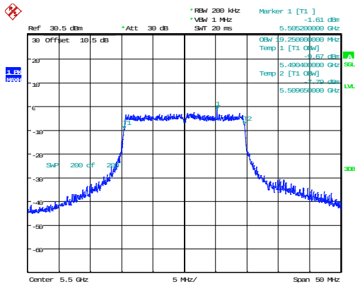
802.11ax20_5500MHz_RU_Full
