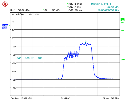
802.11ax40_5670MHz_RU_106/56
