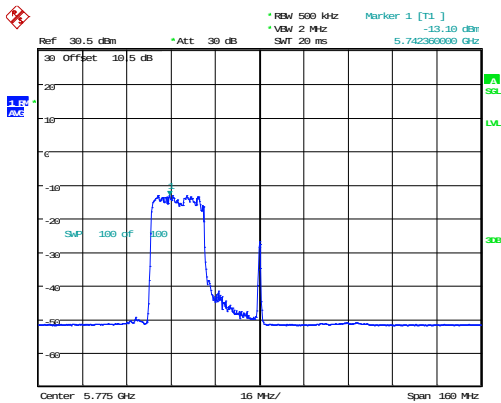
802.11ax80_5775MHz_RU_242/61
