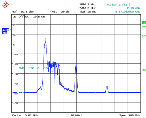
802.11ax80_5610MHz_RU_26/0
