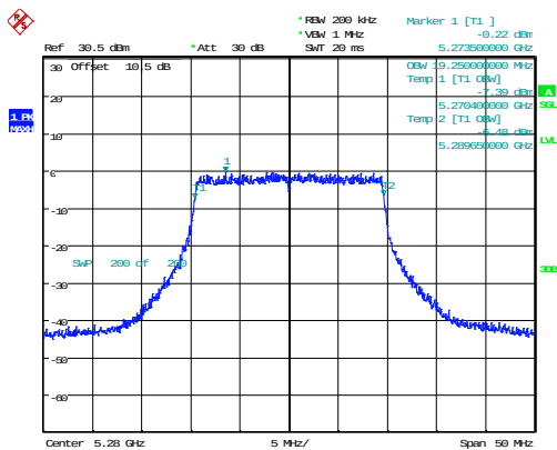
802.11ax20_5280MHz_RU_Full
