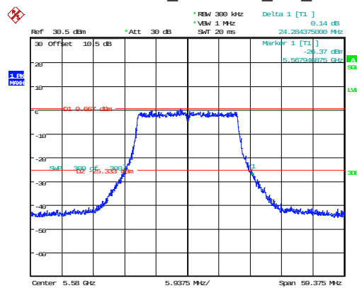
802.11ax20_5580MHz_RU_Full
