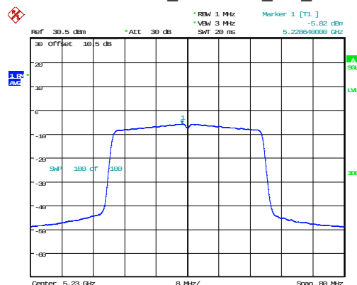
802.11ax40_5230MHz_RU_Full
