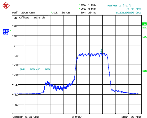
802.11ax40_5310MHz_RU_242/62
