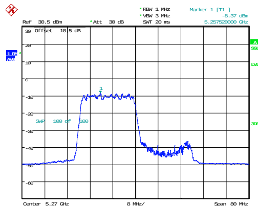
802.11ax40_5270MHz_RU_242/61
