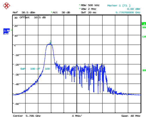
802.11ax20_5785MHz_RU_26/0
