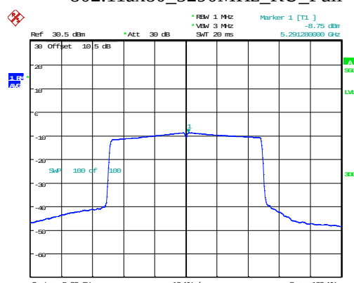
802.11ax80_5290MHz_RU_Full
