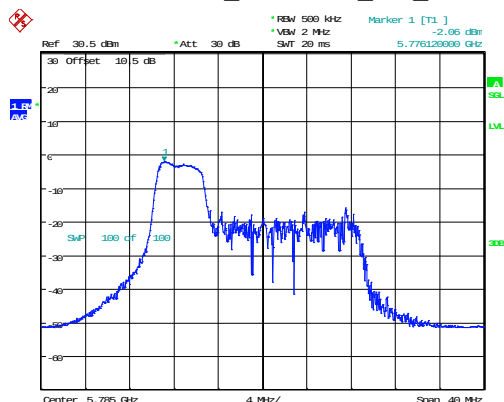
802.11ax20_5785MHz_RU_52/37
