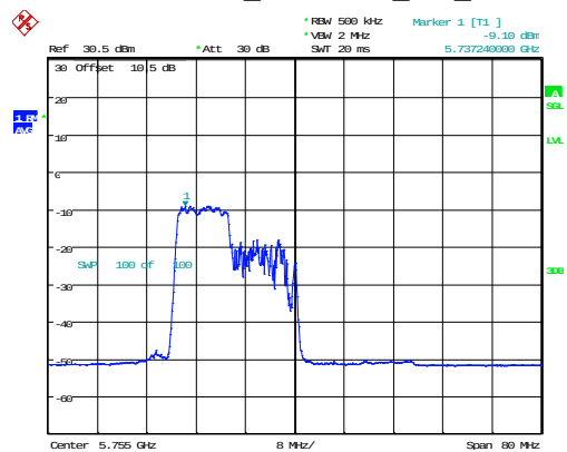
802.11ax40_5755MHz_RU_106/53
