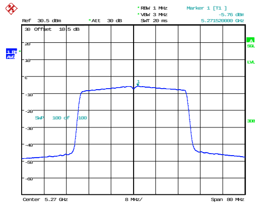
802.11ax40_5270MHz_RU_Full
