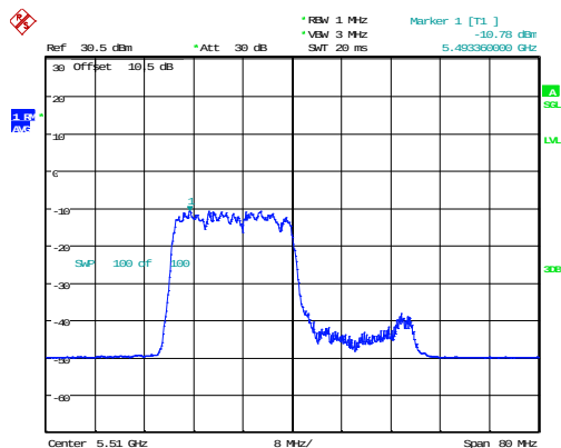
802.11ax40_5510MHz_RU_242/61
