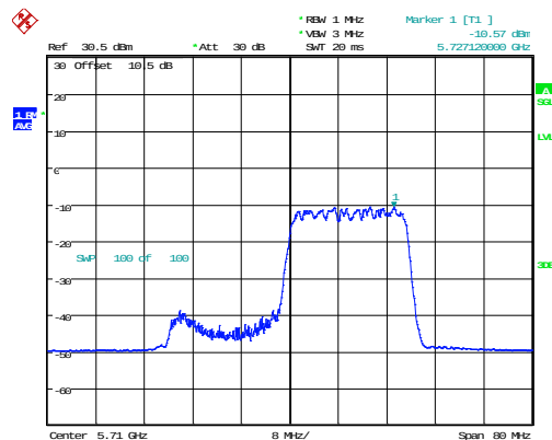
802.11ax40_5710MHz_RU_242/62
