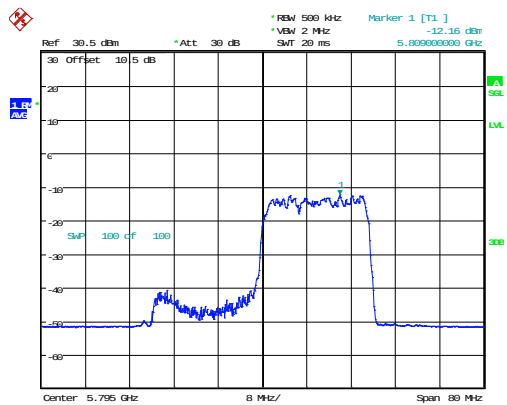
802.11ax40_5795MHz_RU_242/62
