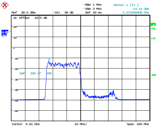
802.11ax80_5610MHz_RU_484/65
