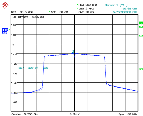
802.11ax40_5755MHz_RU_Full
