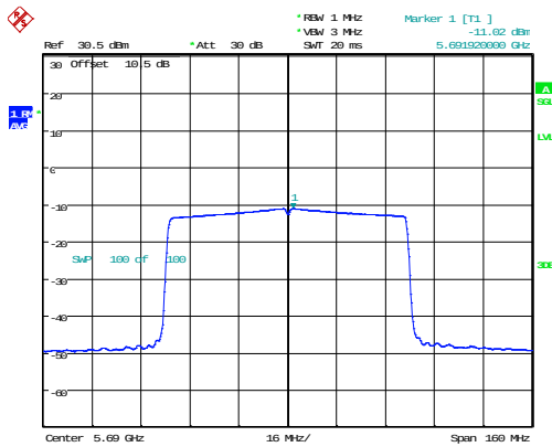
802.11ax80_5690MHz_RU_Full
