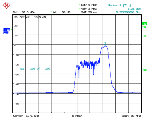
802.11ax40_5710MHz_RU_52/44
