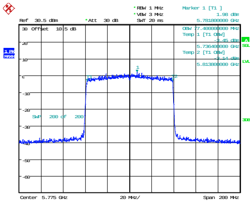
802.11ax80_5775MHz_RU_Full
