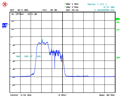
802.11ax40_5510MHz_RU_106/53
