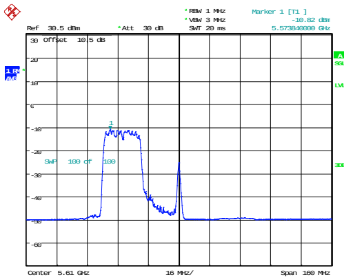
802.11ax80_5610MHz_RU_242/61
