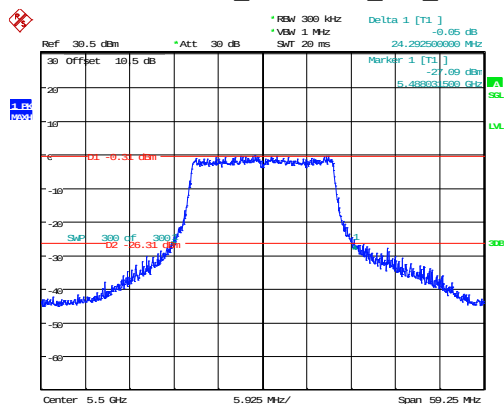
802.11ax20_5500MHz_RU_Full
