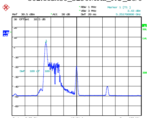
802.11ax80_5290MHz_RU_26/0
