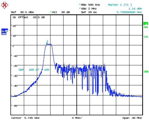
802.11ax20_5745MHz_RU_26/0
