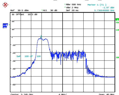
802.11ax20_5745MHz_RU_52/37
