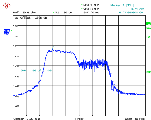
802.11ax20_5280MHz_RU_106/53
