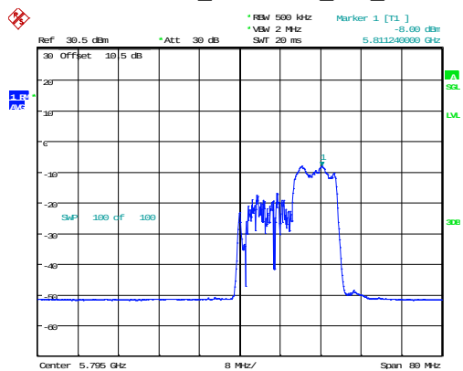
802.11ax40_5795MHz_RU_106/56
