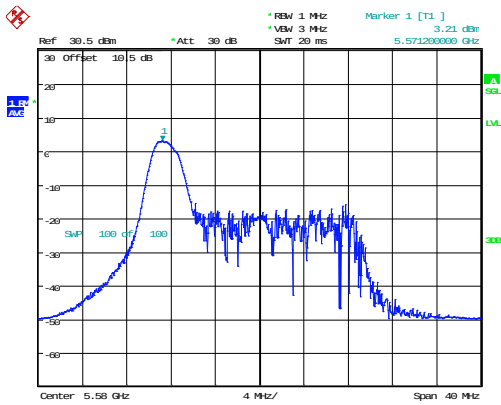
802.11ax20_5580MHz_RU_26/0
