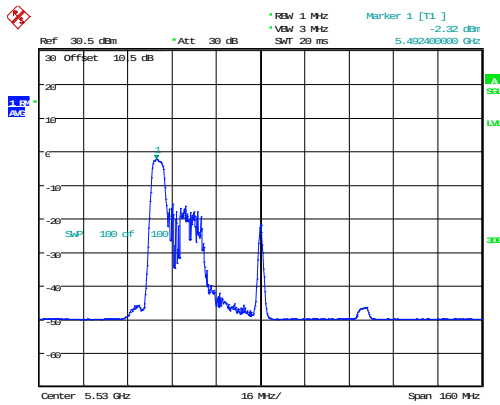
802.11ax80_5530MHz_RU_52/37
