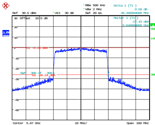
802.11ax40_5670MHz_RU_Full
