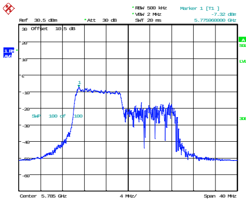
802.11ax20_5785MHz_RU_106/53
