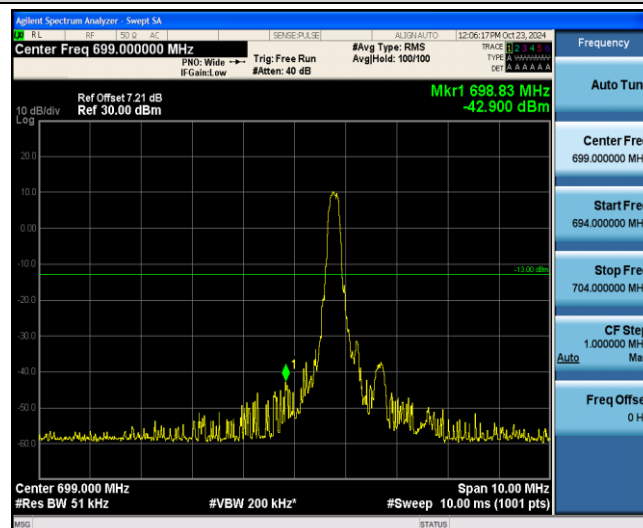
Band12-10MHz-QPSK-23060-1-0-Low--42.90-PASS
