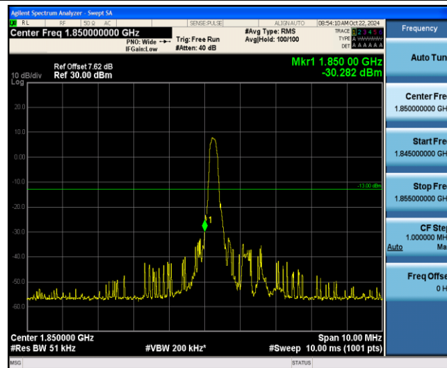
Band2-1.4MHz-16QAM-18607-1-0-Low--30.28-PASS
