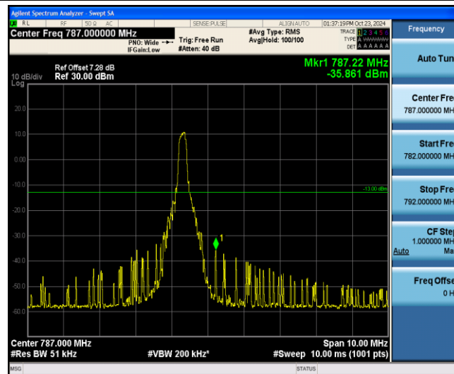
Band13-5MHz-QPSK-23255-1-5-High--35.86-PASS
