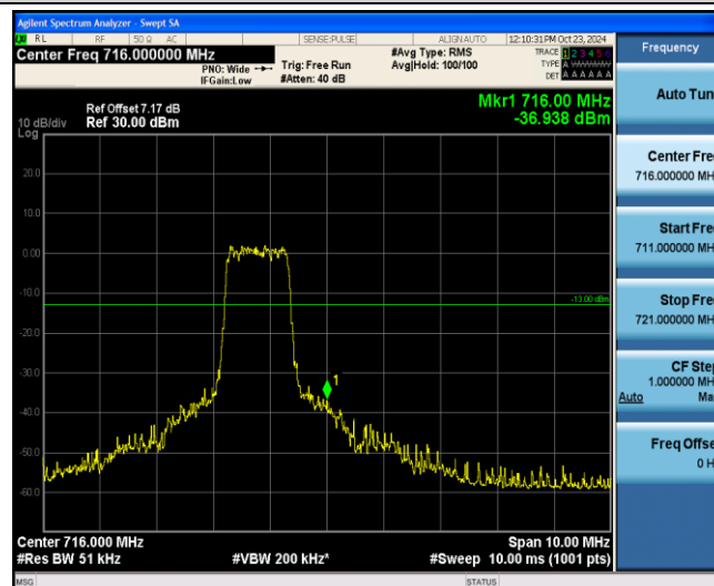
Band12-10MHz-QPSK-23130-6-0-High--36.94-PASS
