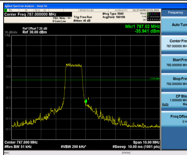
Band13-5MHz-QPSK-23255-6-0-High--35.94-PASS
