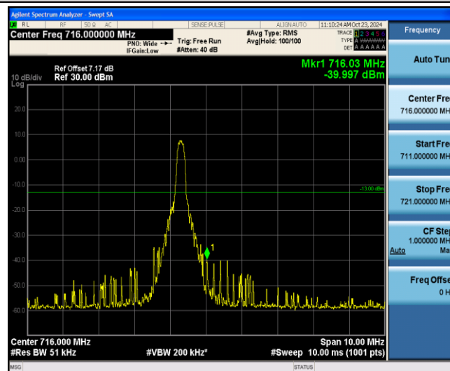
Band12-5MHz-QPSK-23155-1-5-High--40.00-PASS
