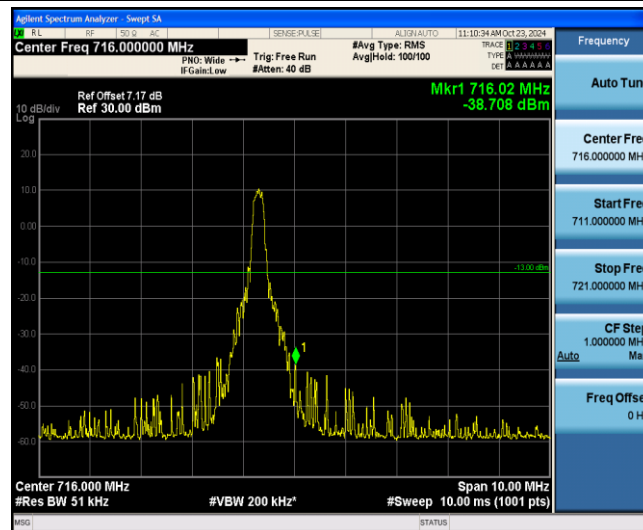
Band12-5MHz-16QAM-23155-1-5-High--38.71-PASS
