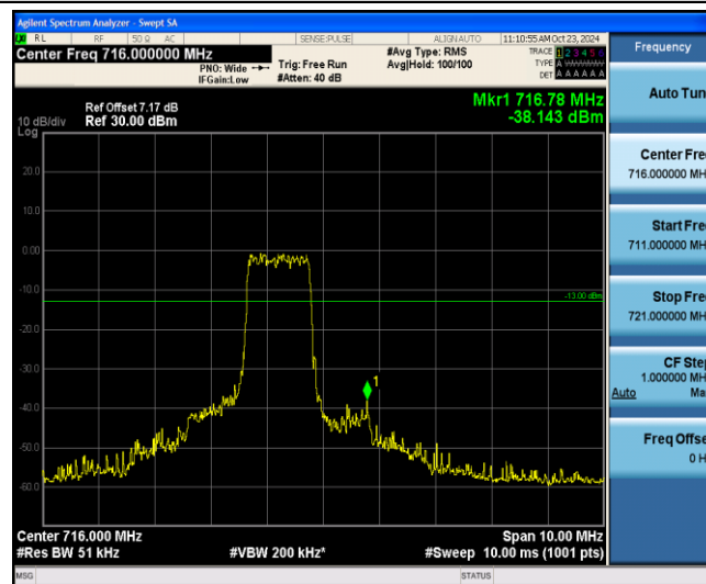
Band12-5MHz-16QAM-23155-6-0-High--38.14-PASS
