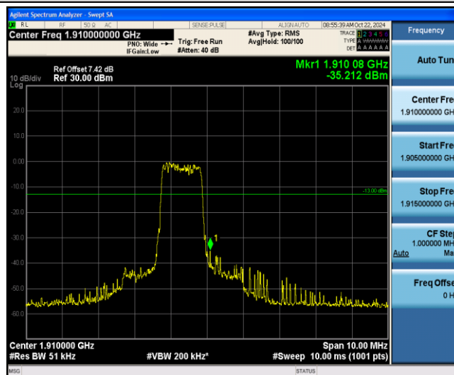
Band2-1.4MHz-QPSK-19193-6-0-High--35.21-PASS
