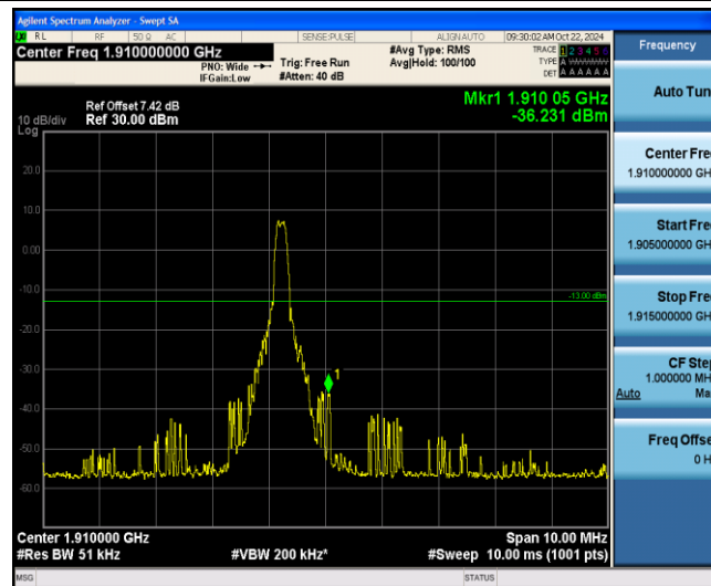
Band2-3MHz-QPSK-19185-1-5-High--36.23-PASS
