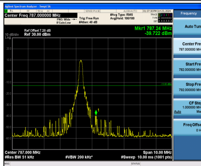
Band13-5MHz-16QAM-23255-1-5-High--39.72-PASS
