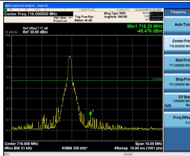
Band12-10MHz-16QAM-23130-1-5-High--46.48-PASS
