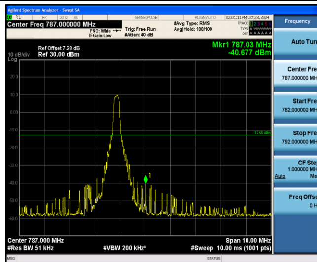
Band13-10MHz-QPSK-23230-1-5-High--40.68-PASS
