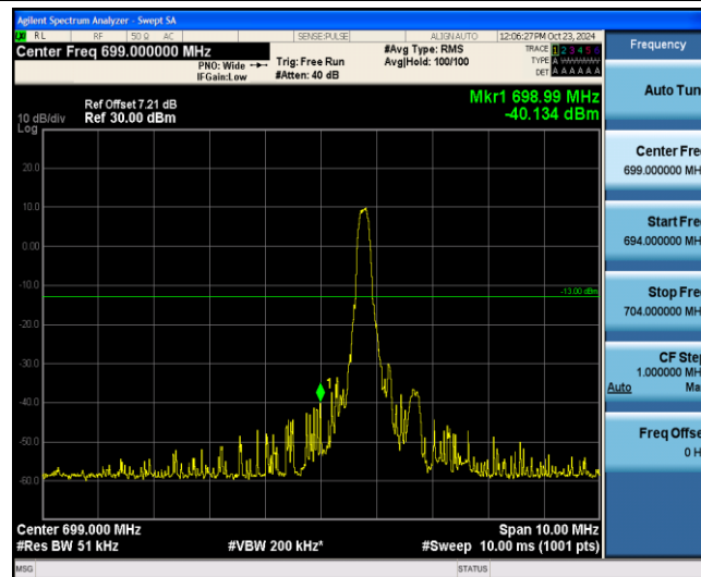
Band12-10MHz-16QAM-23060-1-0-Low--40.13-PASS
