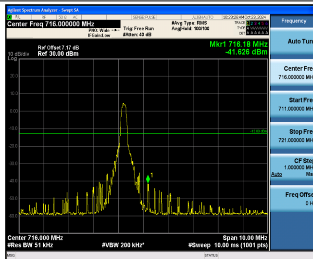
Band12-3MHz-16QAM-23165-1-5-High--41.63-PASS
