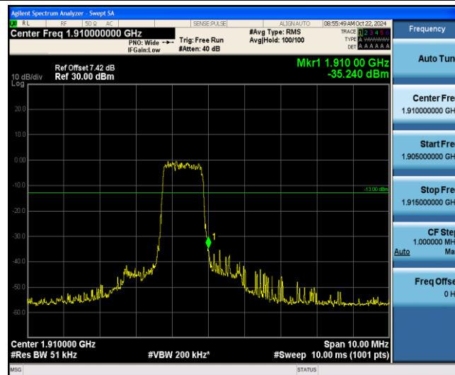
Band2-1.4MHz-16QAM-19193-6-0-High--35.24-PASS
