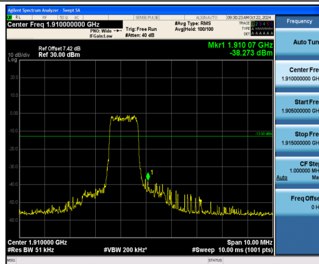
Band2-3MHz-QPSK-19185-6-0-High--38.27-PASS
