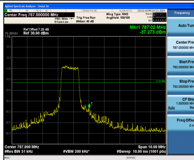
Band13-10MHz-16QAM-23230-6-0-High--37.27-PASS
