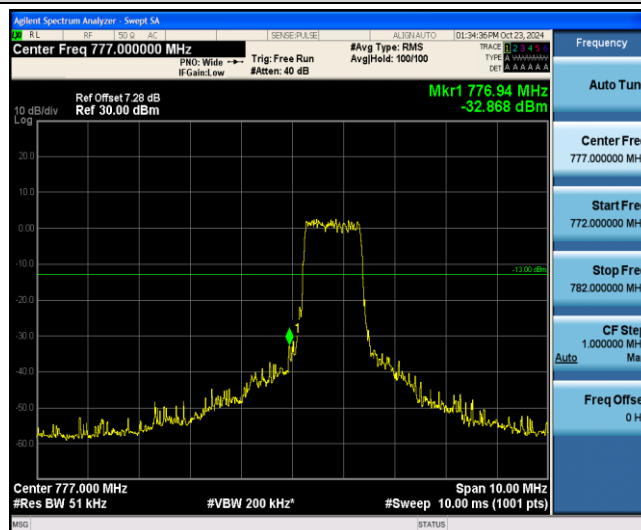
Band13-5MHz-QPSK-23205-6-0-Low--32.87-PASS
