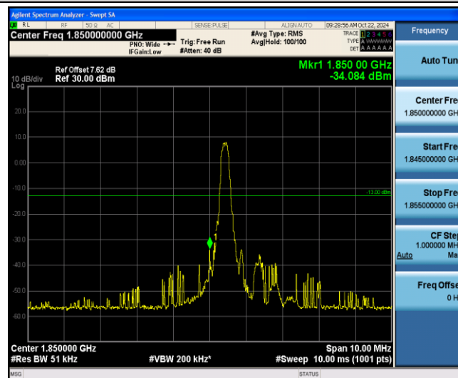
Band2-3MHz-16QAM-18615-1-0-Low--34.08-PASS
