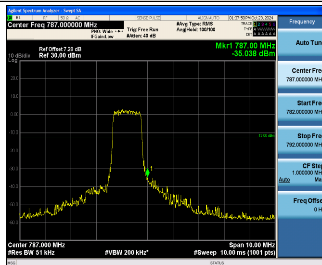
Band13-5MHz-16QAM-23255-6-0-High--35.04-PASS
