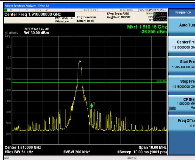
Band2-1.4MHz-16QAM-19193-1-5-High--36.86-PASS
