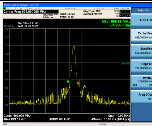
Band12-5MHz-16QAM-23035-1-0-Low--34.97-PASS
