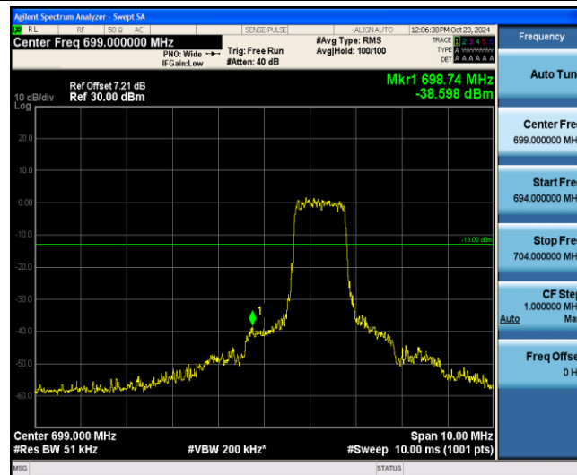
Band12-10MHz-QPSK-23060-6-0-Low--38.60-PASS
