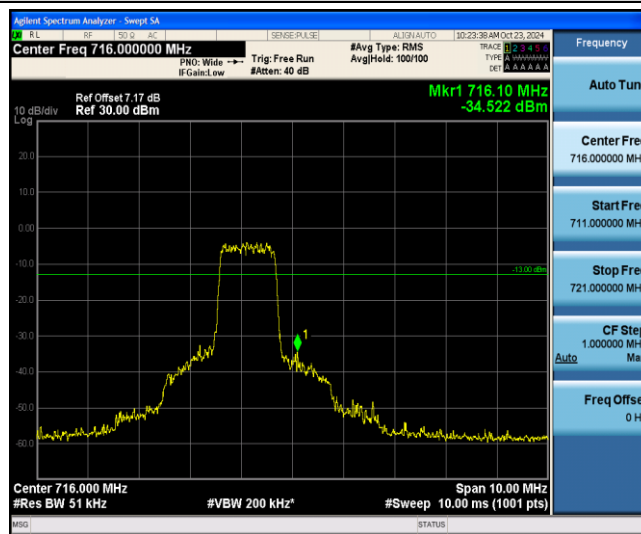
Band12-3MHz-QPSK-23165-6-0-High--34.52-PASS
