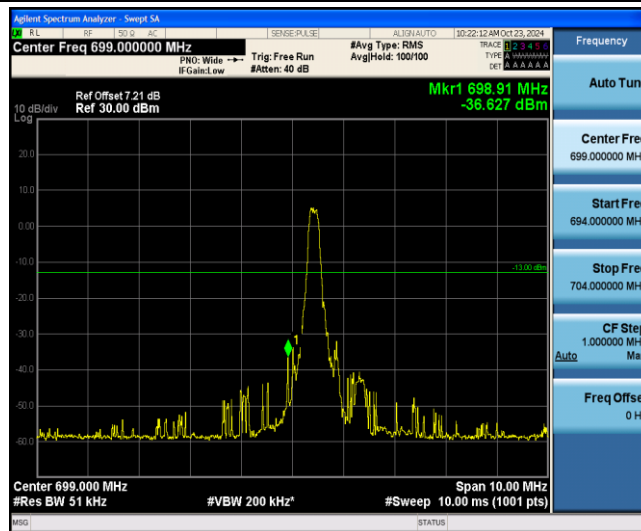
Band12-3MHz-16QAM-23025-1-0-Low--36.63-PASS
