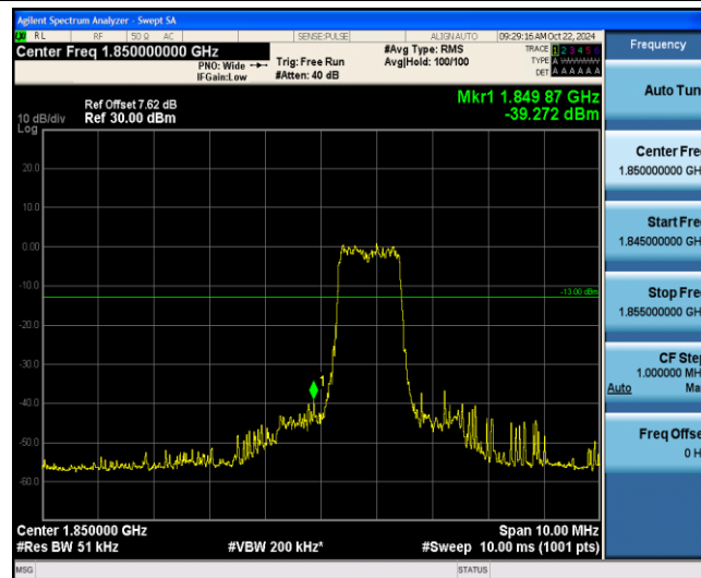
Band2-3MHz-16QAM-18615-6-0-Low--39.27-PASS
