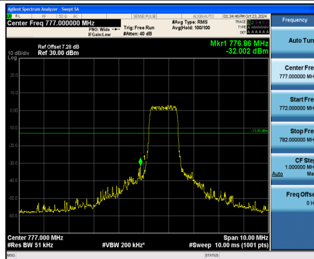
Band13-5MHz-16QAM-23205-6-0-Low--32.00-PASS
