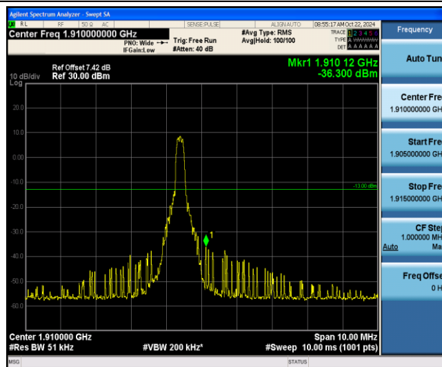
Band2-1.4MHz-QPSK-19193-1-5-High--36.30-PASS
