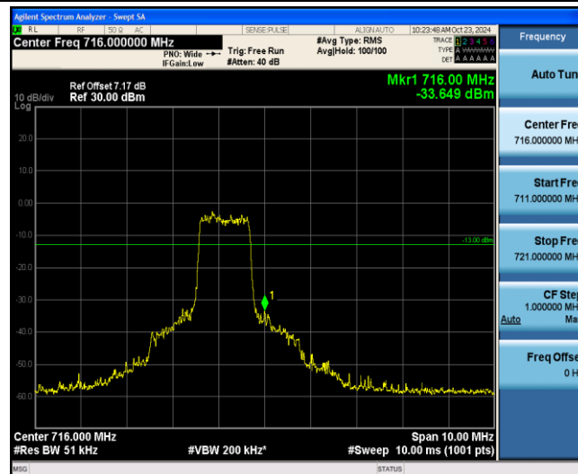
Band12-3MHz-16QAM-23165-6-0-High--33.65-PASS
