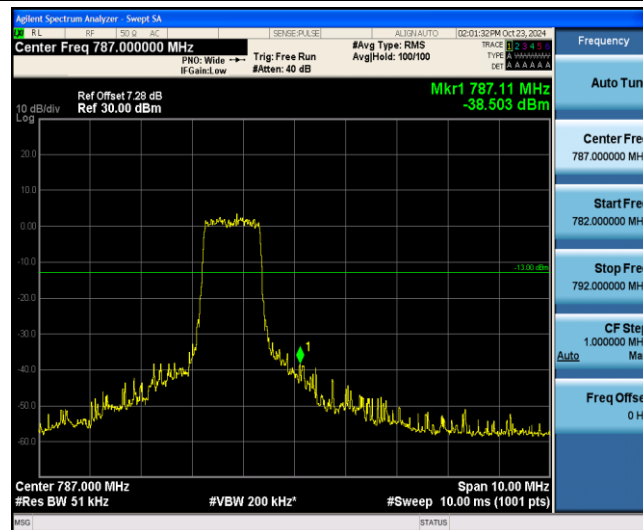
Band13-10MHz-QPSK-23230-6-0-High--38.50-PASS
