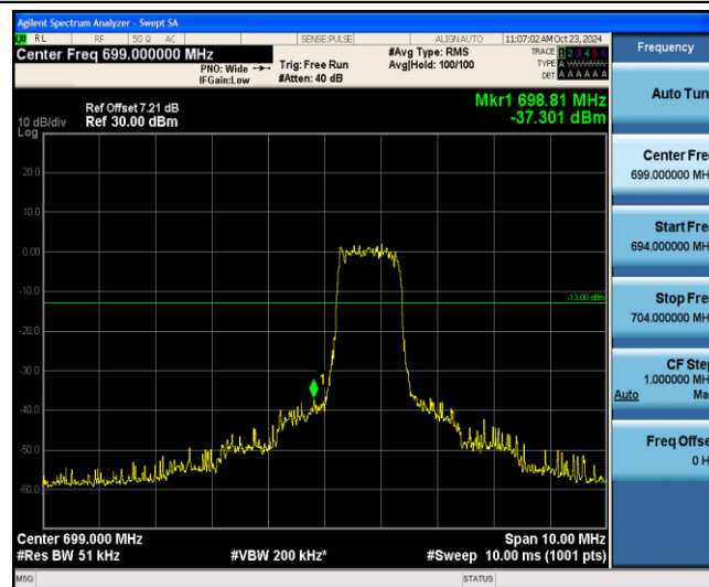
Band12-5MHz-QPSK-23035-6-0-Low--37.30-PASS
