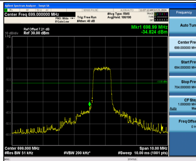
Band12-5MHz-16QAM-23035-6-0-Low--34.82-PASS
