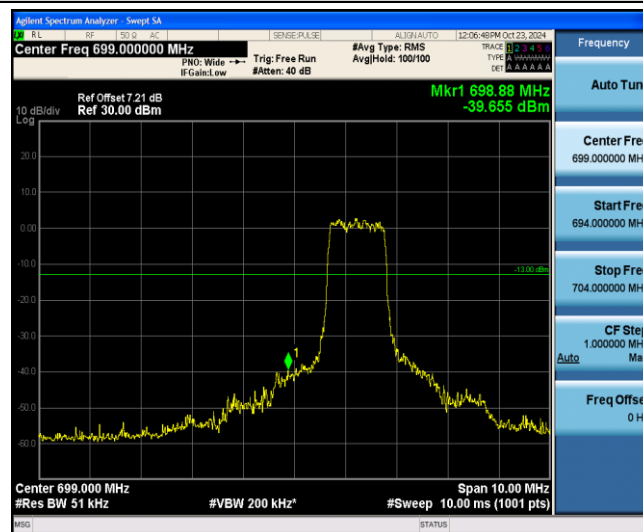
Band12-10MHz-16QAM-23060-6-0-Low--39.65-PASS
