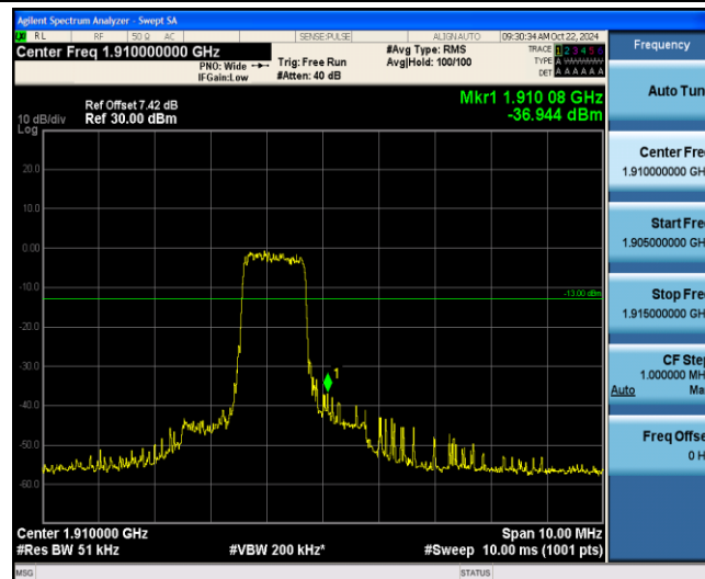
Band2-3MHz-16QAM-19185-6-0-High--36.94-PASS
