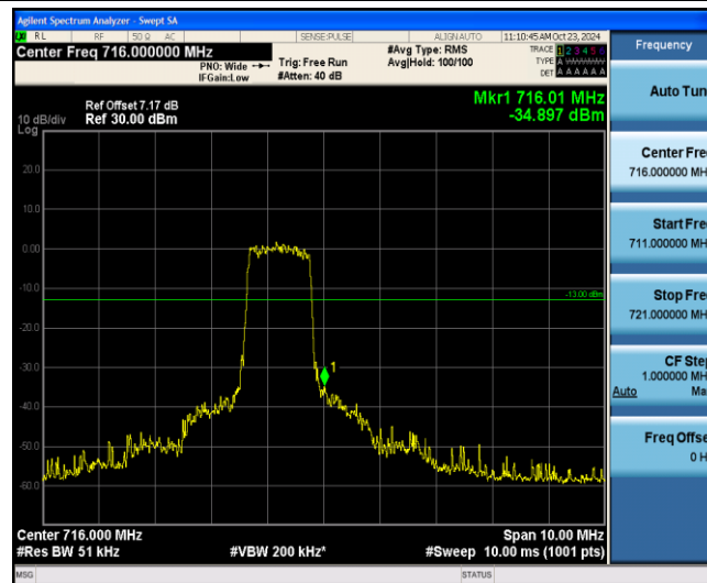
Band12-5MHz-QPSK-23155-6-0-High--34.90-PASS
