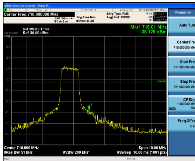
Band12-10MHz-16QAM-23130-6-0-High--38.13-PASS
