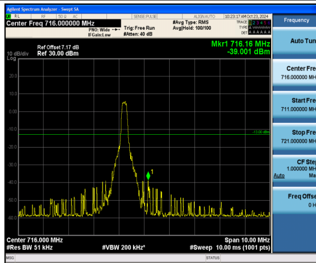
Band12-3MHz-QPSK-23165-1-5-High--39.00-PASS
