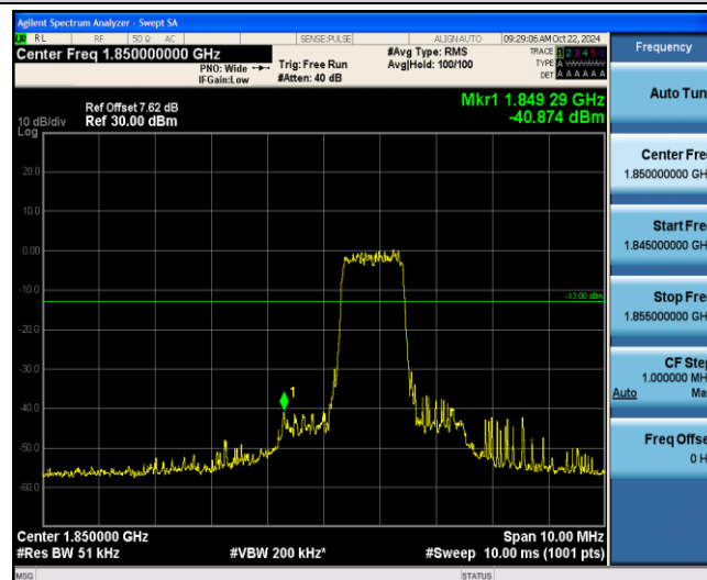
Band2-3MHz-QPSK-18615-6-0-Low--40.87-PASS
