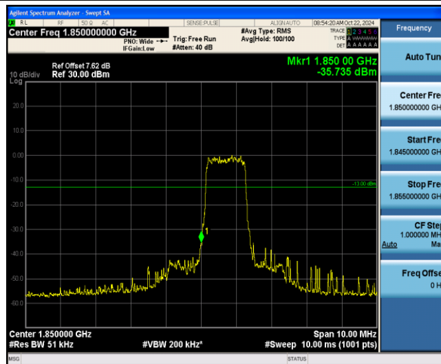
Band2-1.4MHz-QPSK-18607-6-0-Low--35.73-PASS
