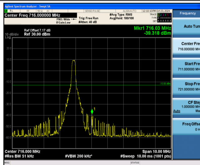
Band12-10MHz-QPSK-23130-1-5-High--39.32-PASS
