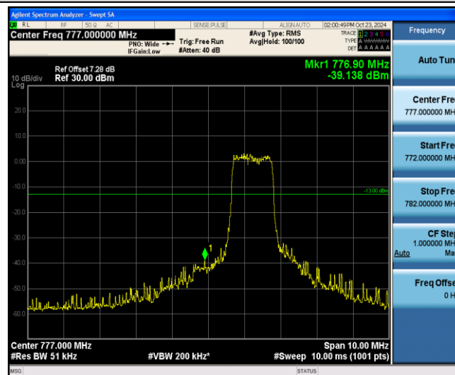
Band13-10MHz-QPSK-23230-6-0-Low--39.14-PASS
