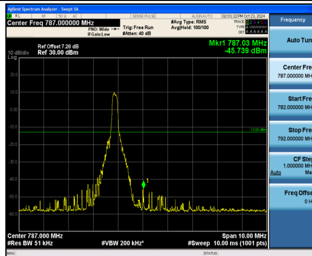
Band13-10MHz-16QAM-23230-1-5-High--45.74-PASS
