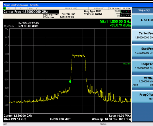
Band2-1.4MHz-16QAM-18607-6-0-Low--35.08-PASS
