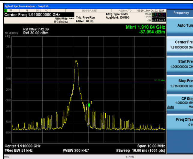
Band2-3MHz-16QAM-19185-1-5-High--37.09-PASS
