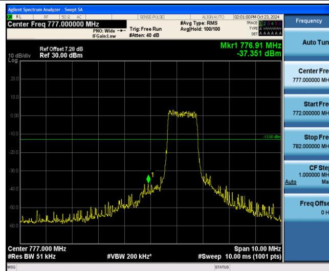
Band13-10MHz-16QAM-23230-6-0-Low--37.35-PASS
