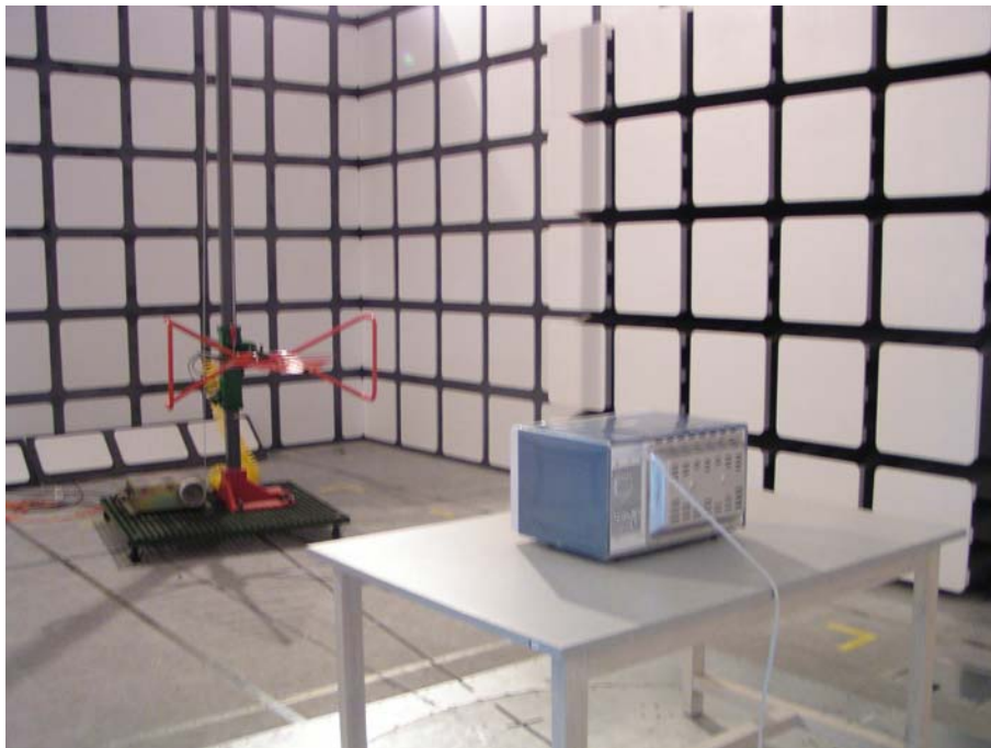
Radiated Emission (30MHz to 1000MHz) - Rear View
