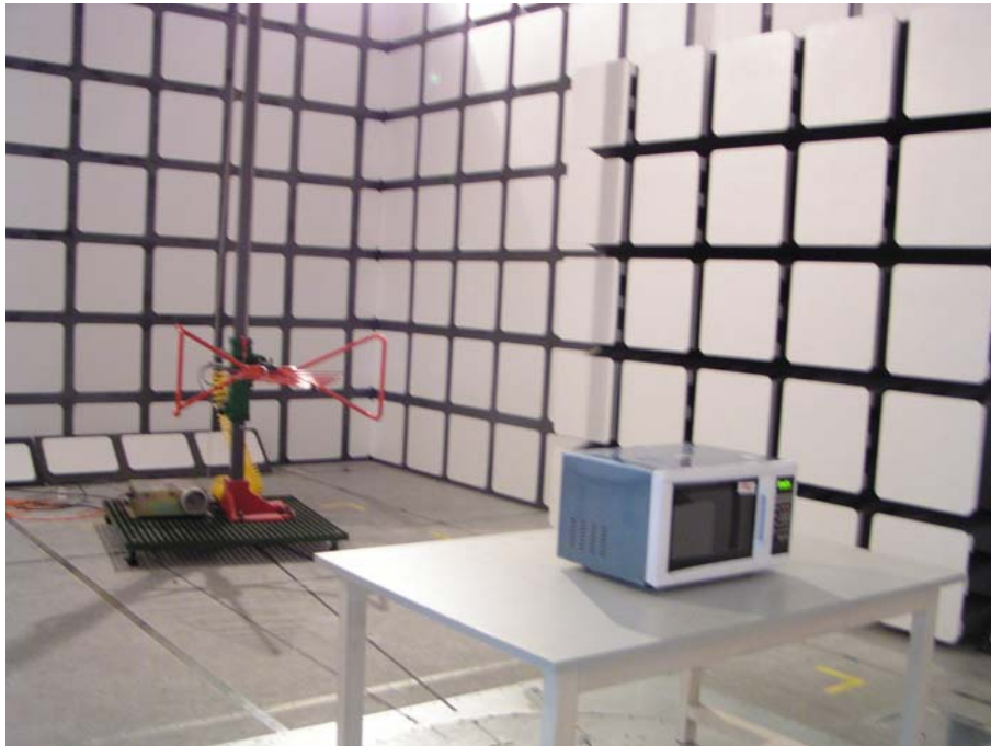
Radiated Emission (30MHz to 1000MHz) - Front View
