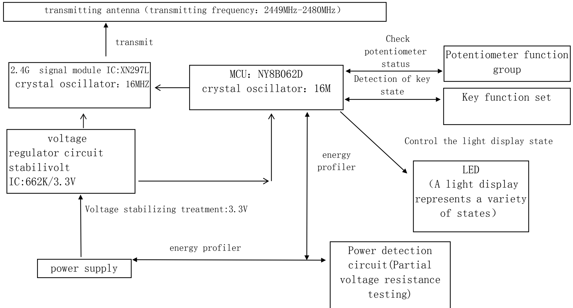
DHW-E58T block diagram
