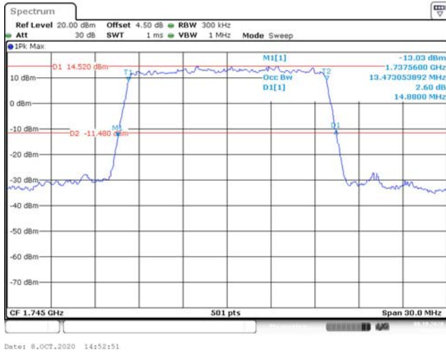
15M, QPSK, High Channel
