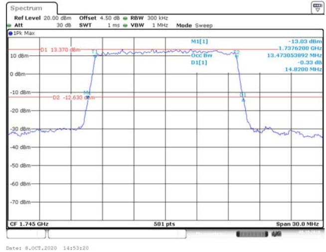
15M, 16QAM, High Channel
