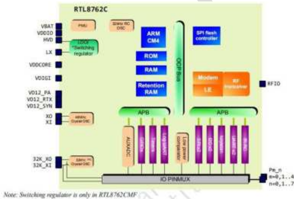
Figure 1. Block Diagram of RTL8762CMF
