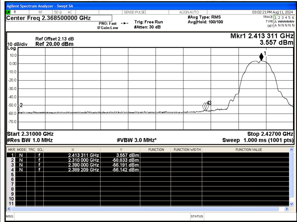
Restrict Band NVNT b 2412MHz Ant Average
