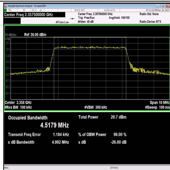
40(2350-2360)-5MHz-16QAM-39225-25RB#0-PASS
