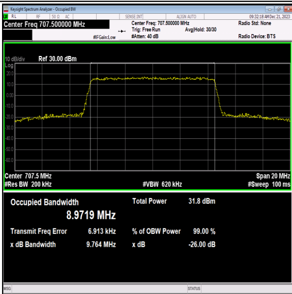
Band12-10MHz-QPSK-23095-50RB#0-PASS
