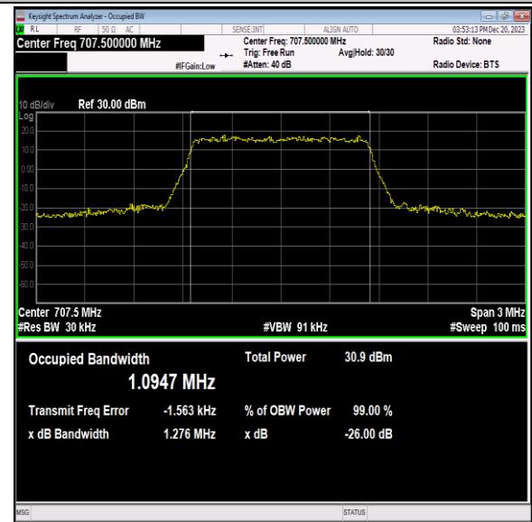
Band12-1.4MHz-QPSK-23095-6RB#0-PASS
