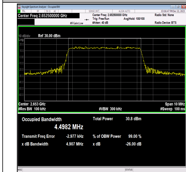
41(2535-2655)-5MHz-64QAM-41215-25RB#0-PASS
