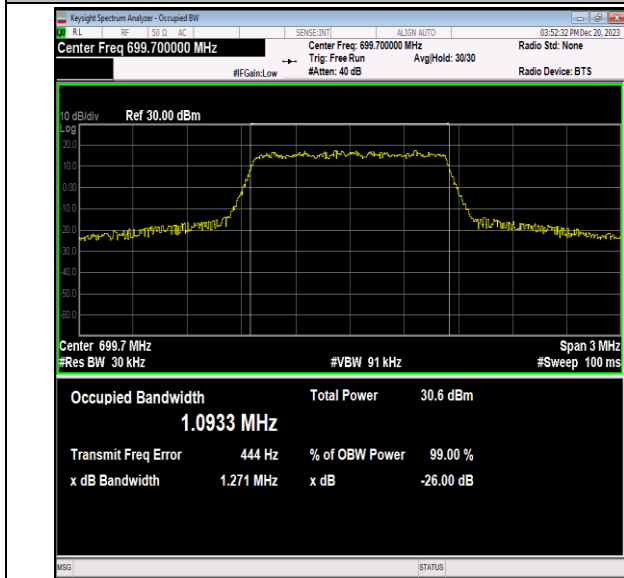
Band12-1.4MHz-QPSK-23017-6RB#0-PASS
