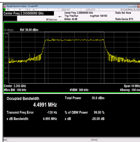
40(2350-2360)-5MHz-64QAM-39200-25RB#0-PASS
