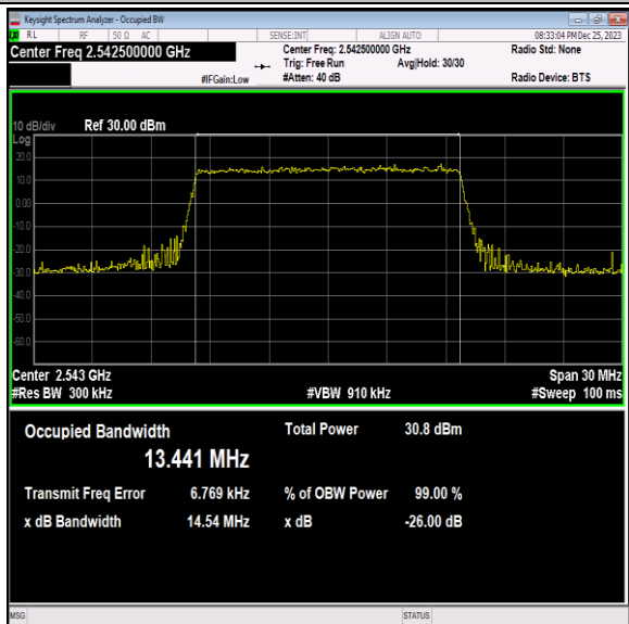
41(2535-2655)-15MHz-64QAM-40115-75RB#0-PASS
