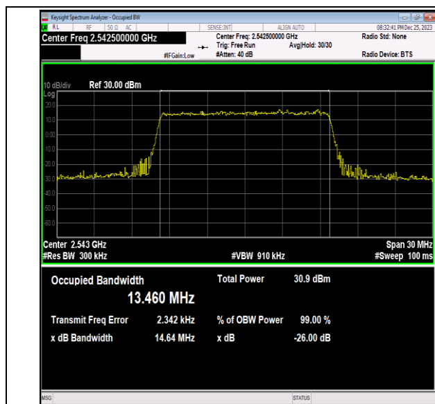
41(2535-2655)-15MHz-QPSK-40115-75RB#0-PASS
