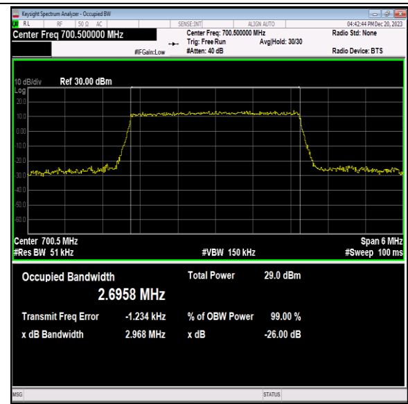
Band12-3MHz-64QAM-23025-15RB#0-PASS
