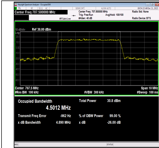
Band12-5MHz-16QAM-23095-25RB#0-PASS
