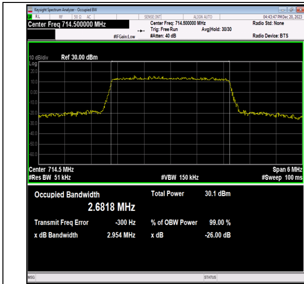
Band12-3MHz-16QAM-23165-15RB#0-PASS
