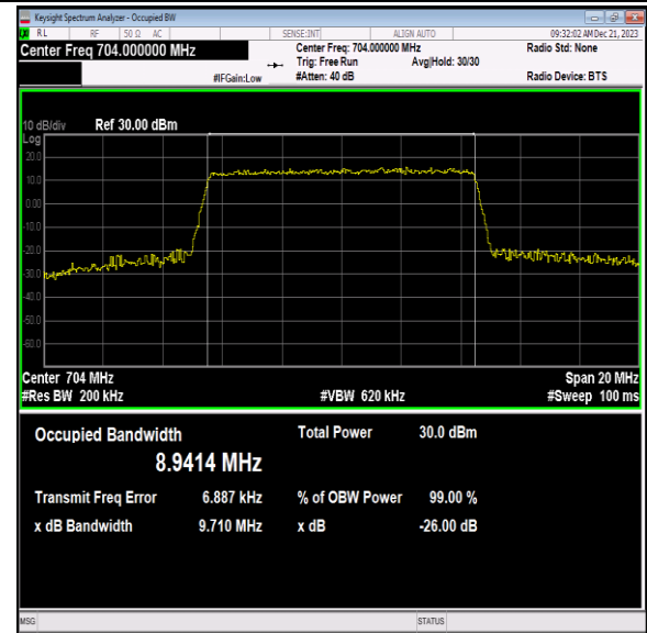
Band12-10MHz-64QAM-23060-50RB#0-PASS
