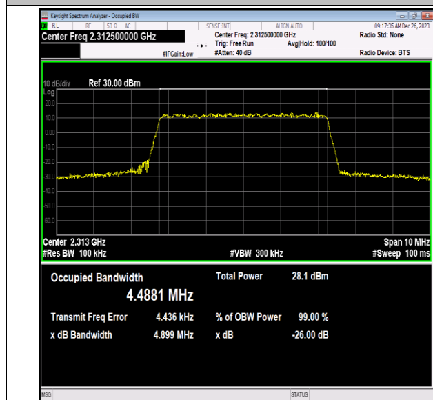
40(2305-2315)-5MHz-64QAM-38775-25RB#0-PASS
