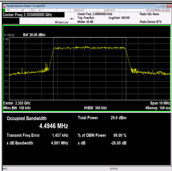
40(2350-2360)-5MHz-16QAM-39200-25RB#0-PASS
