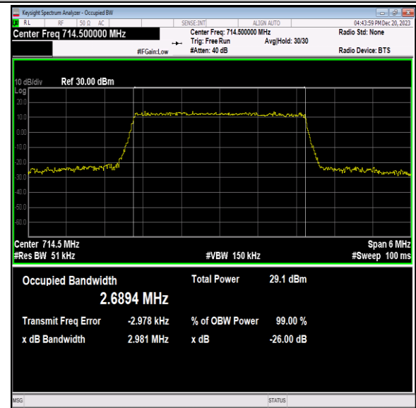
Band12-3MHz-64QAM-23165-15RB#0-PASS
