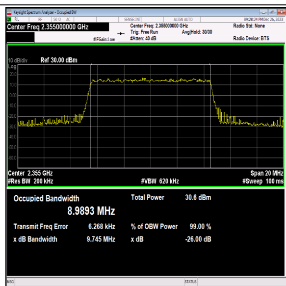
40(2350-2360)-10MHz-64QAM-39200-50RB#0-PASS
