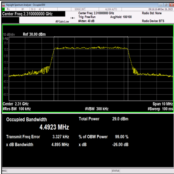
40(2305-2315)-5MHz-16QAM-38750-25RB#0-PASS
