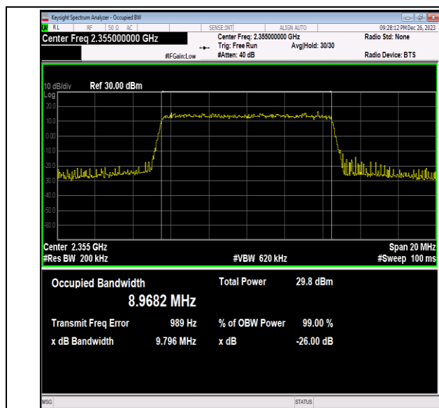
40(2350-2360)-10MHz-16QAM-39200-50RB#0-PASS
