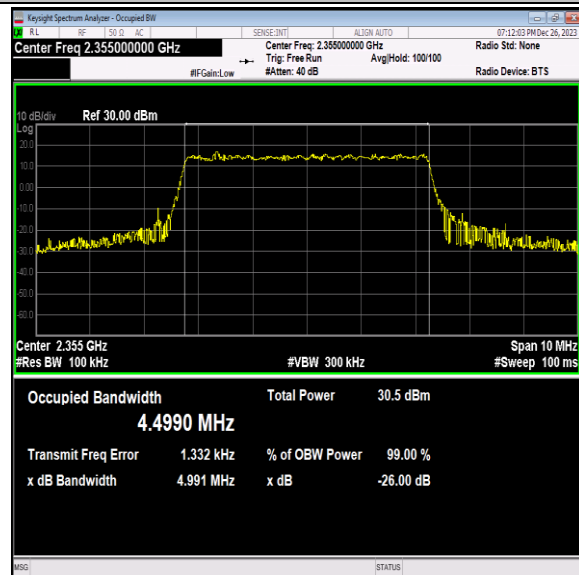
40(2350-2360)-5MHz-QPSK-39200-25RB#0-PASS
