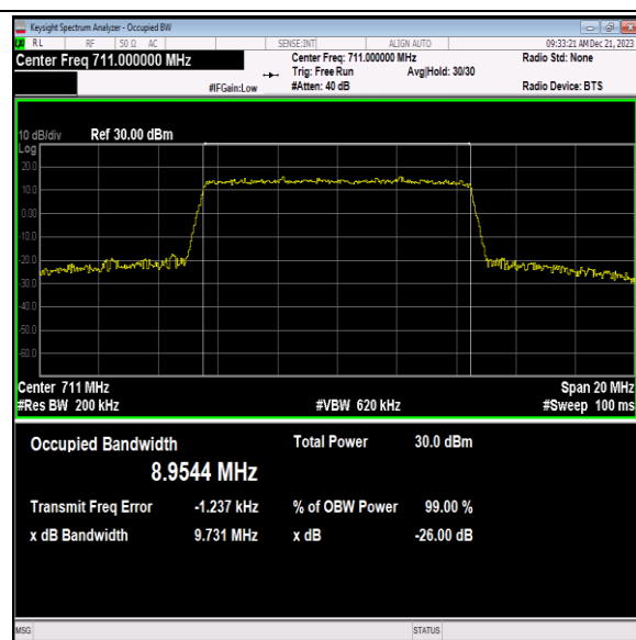
Band12-10MHz-64QAM-23130-50RB#0-PASS
