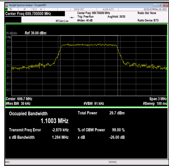
Band12-1.4MHz-16QAM-23017-6RB#0-PASS
