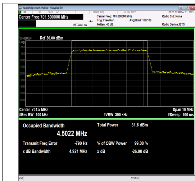
Band12-5MHz-QPSK-23035-25RB#0-PASS
