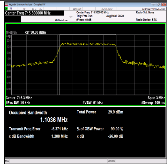
Band12-1.4MHz-16QAM-23173-6RB#0-PASS
