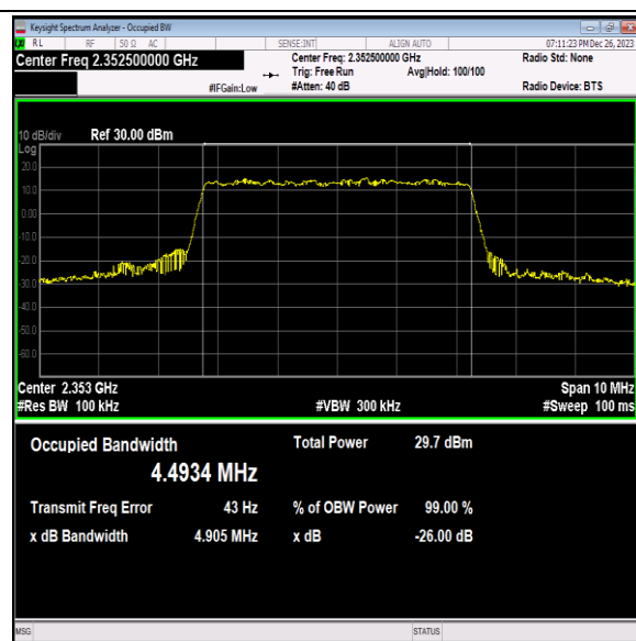
40(2350-2360)-5MHz-16QAM-39175-25RB#0-PASS
