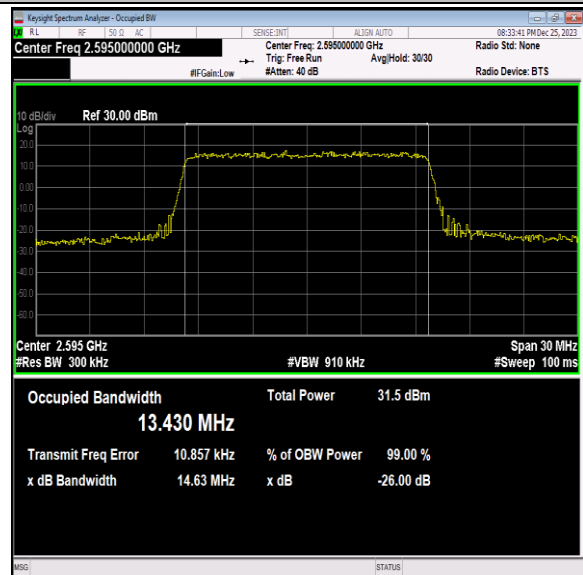
41(2535-2655)-15MHz-64QAM-40640-75RB#0-PASS
