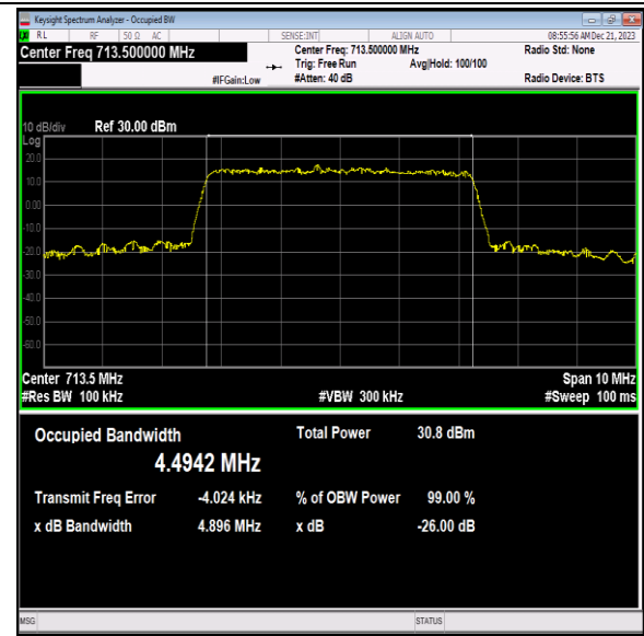
Band12-5MHz-16QAM-23155-25RB#0-PASS
