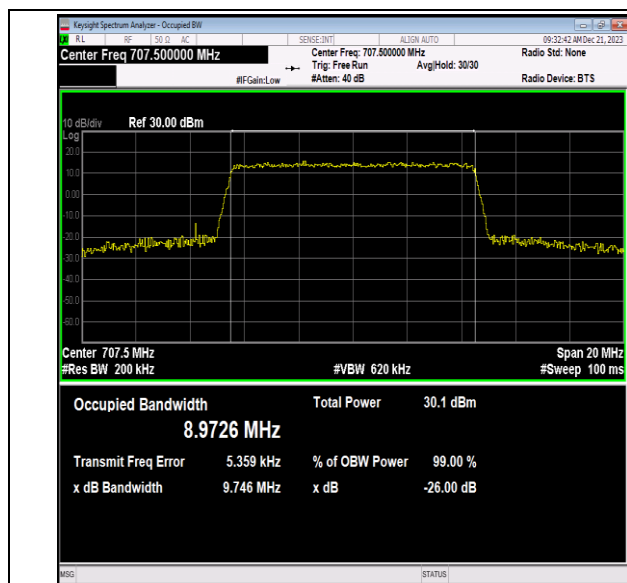
Band12-10MHz-64QAM-23095-50RB#0-PASS
