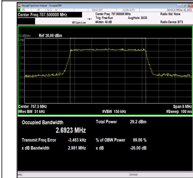
Band12-3MHz-64QAM-23095-15RB#0-PASS
