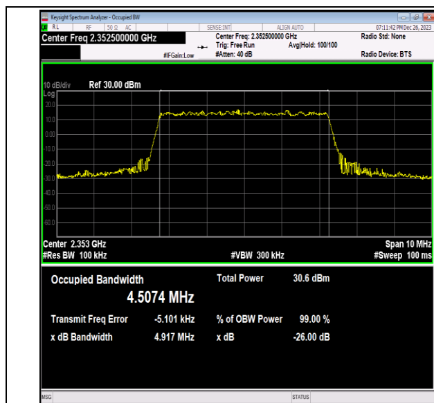
40(2350-2360)-5MHz-64QAM-39175-25RB#0-PASS
