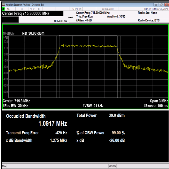
Band12-1.4MHz-64QAM-23173-6RB#0-PASS
