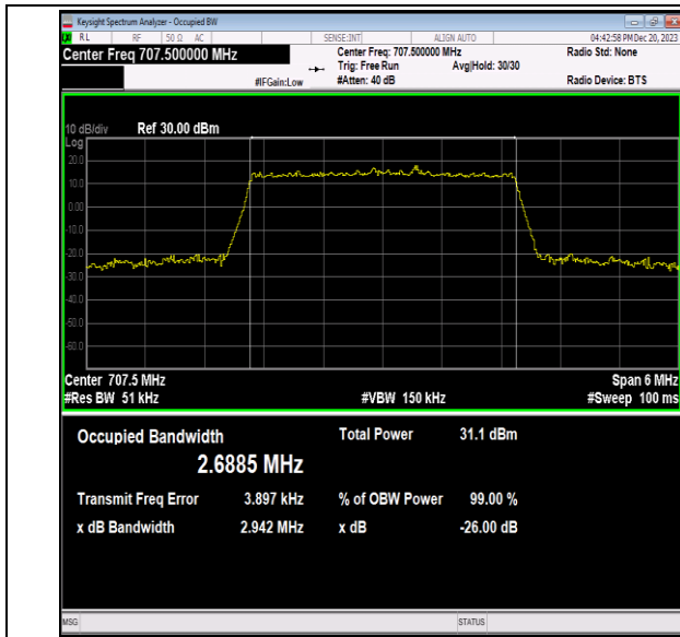
Band12-3MHz-QPSK-23095-15RB#0-PASS
