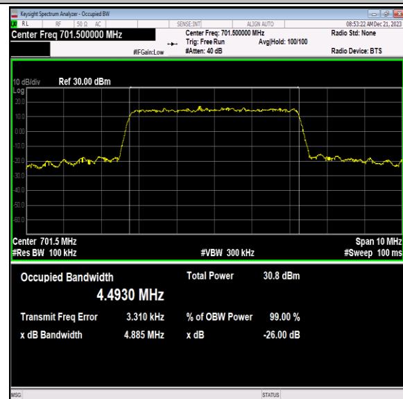
Band12-5MHz-16QAM-23035-25RB#0-PASS
