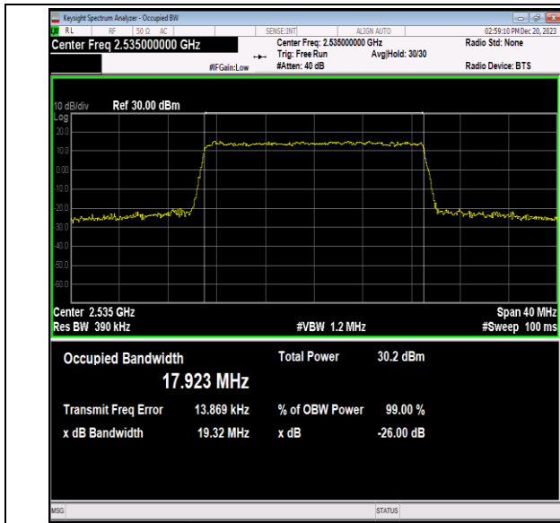
Band7-20MHz-64QAM-21100-100RB#0-PASS
