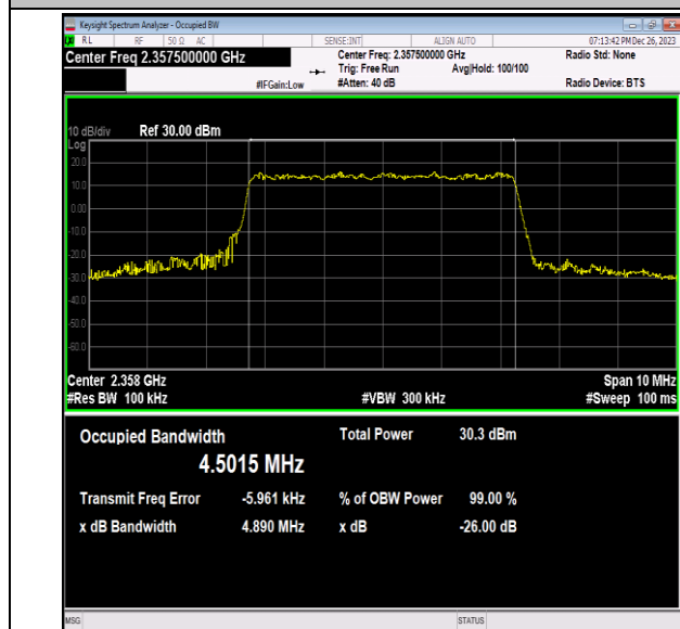
40(2350-2360)-5MHz-64QAM-39225-25RB#0-PASS
