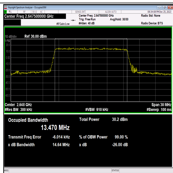
41(2535-2655)-15MHz-16QAM-41165-75RB#0-PASS
