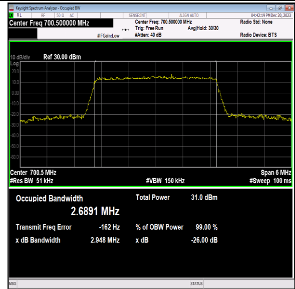
Band12-3MHz-QPSK-23025-15RB#0-PASS
