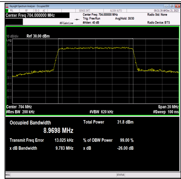
Band12-10MHz-QPSK-23060-50RB#0-PASS
