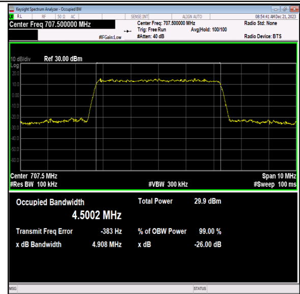
Band12-5MHz-64QAM-23095-25RB#0-PASS
