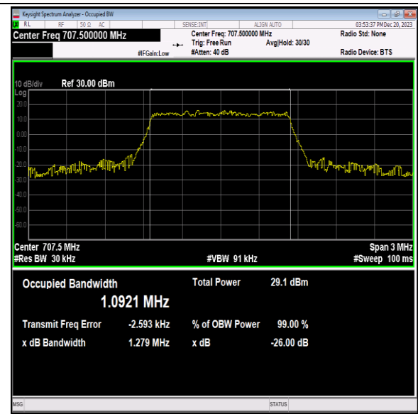
Band12-1.4MHz-64QAM-23095-6RB#0-PASS
