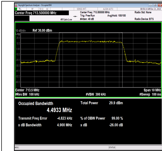
Band12-5MHz-64QAM-23155-25RB#0-PASS
