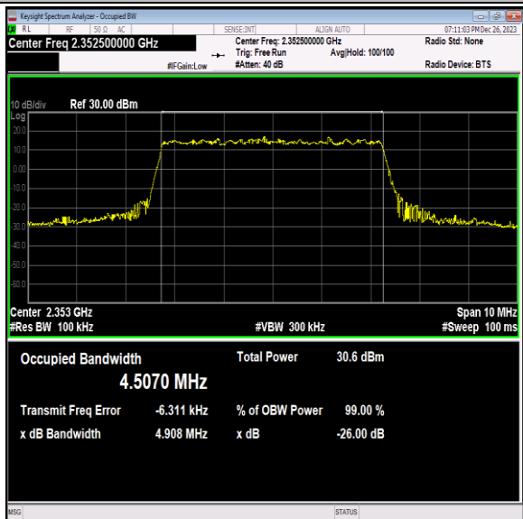
40(2350-2360)-5MHz-QPSK-39175-25RB#0-PASS
