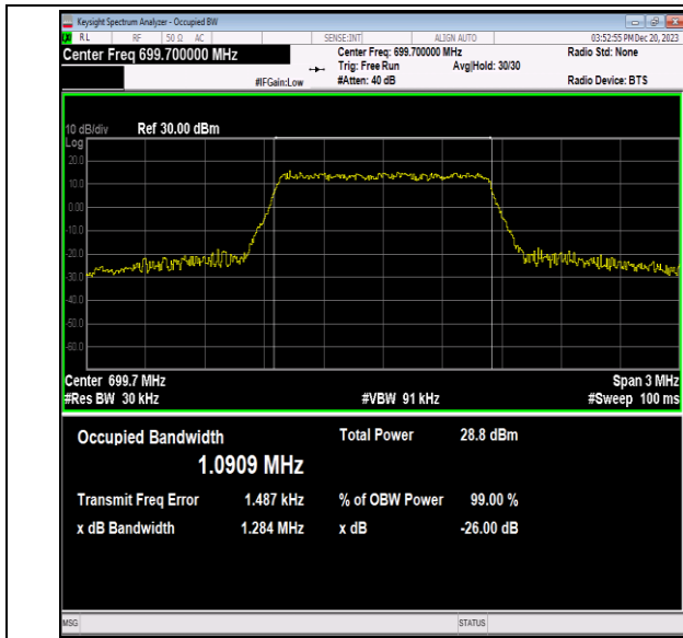
Band12-1.4MHz-64QAM-23017-6RB#0-PASS
