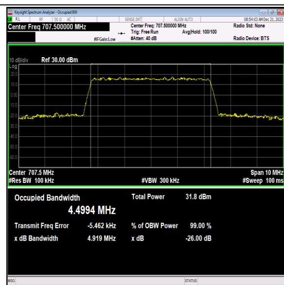
Band12-5MHz-QPSK-23095-25RB#0-PASS
