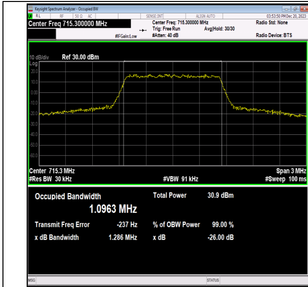
Band12-1.4MHz-QPSK-23173-6RB#0-PASS
