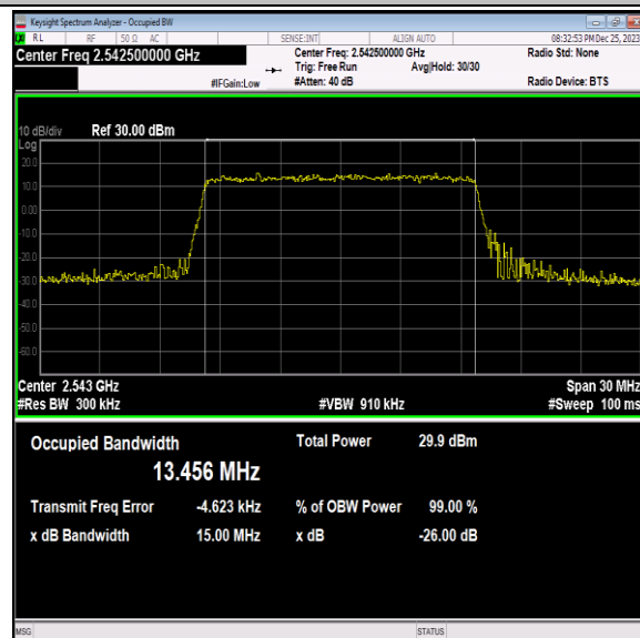
41(2535-2655)-15MHz-16QAM-40115-75RB#0-PASS
