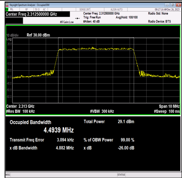
40(2305-2315)-5MHz-16QAM-38775-25RB#0-PASS
