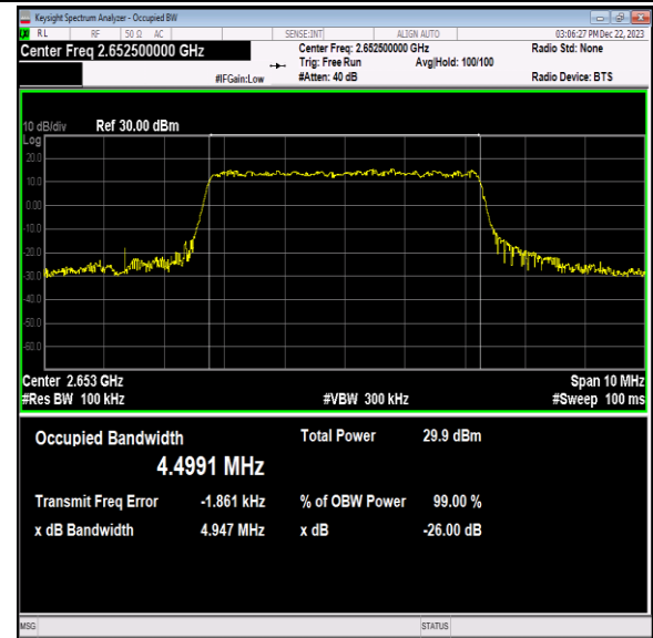
41(2535-2655)-5MHz-16QAM-41215-25RB#0-PASS
