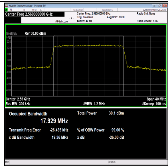
Band7-20MHz-64QAM-21350-100RB#0-PASS
