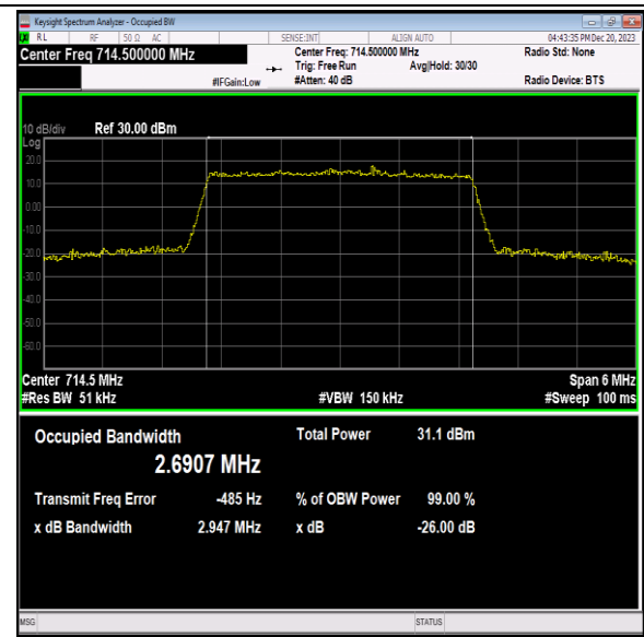
Band12-3MHz-QPSK-23165-15RB#0-PASS
