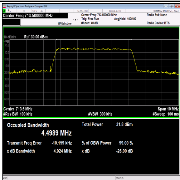
Band12-5MHz-QPSK-23155-25RB#0-PASS
