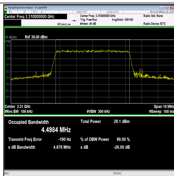
40(2305-2315)-5MHz-64QAM-38750-25RB#0-PASS
