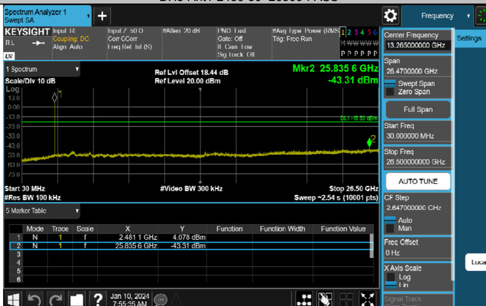
DH5-Ant1-2480-30~26500-PASS
