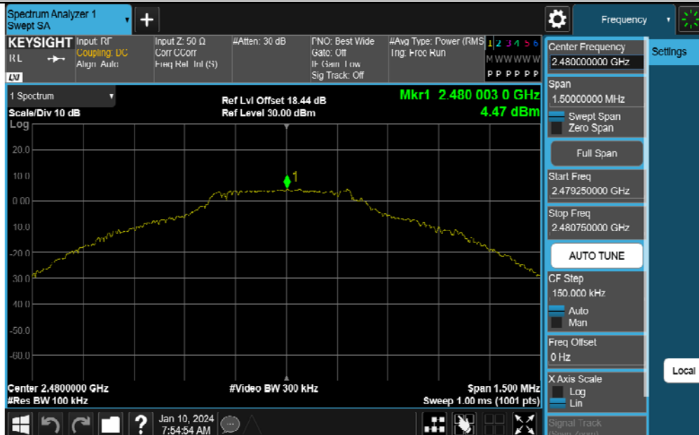
DH5-Ant1-2480-PASS
