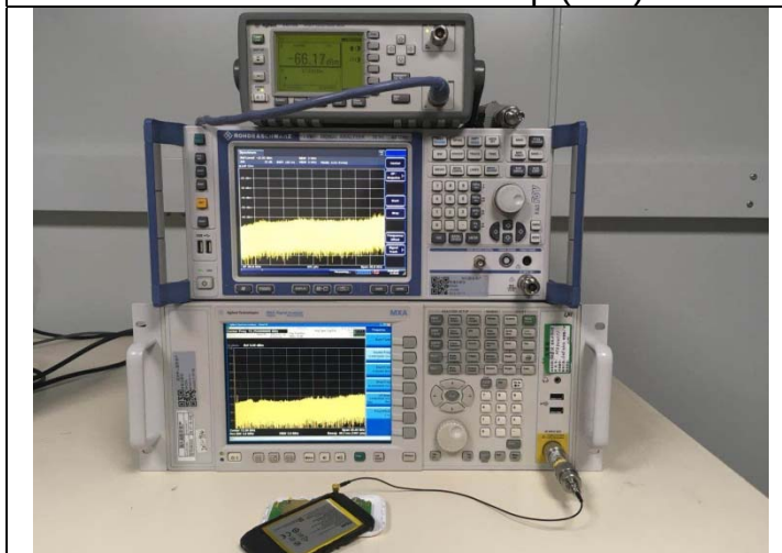
RF Conducted Test setup (WIFI)
