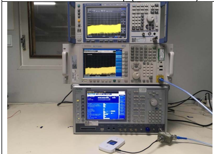
RF Conducted Test setup (LTE)
