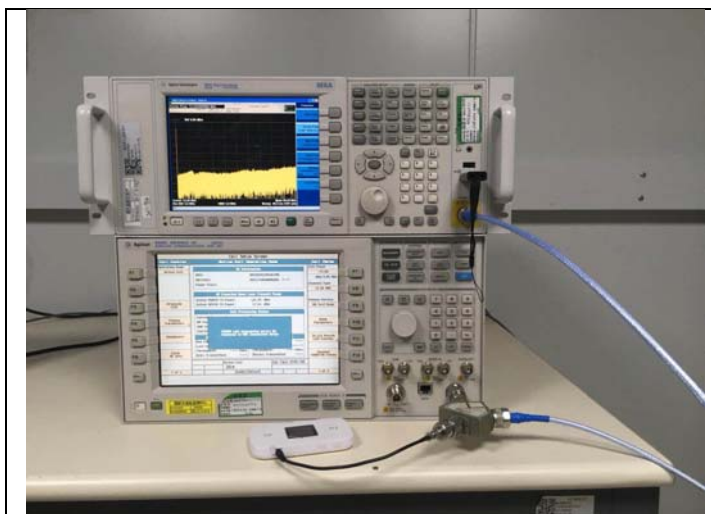
RF Conducted Test setup (GSM/WCDMA)
