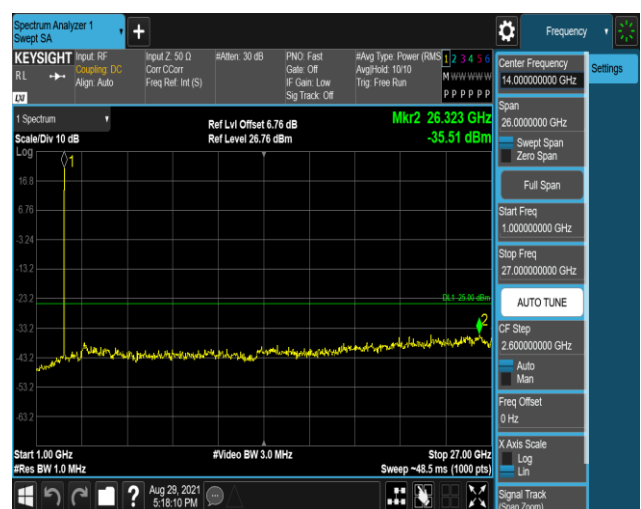
Band38-20MHz-16QAM-38150:1000~27000MHz
