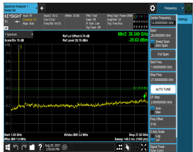
Band7-5MHz-16QAM-21100:1000~27000MHz
