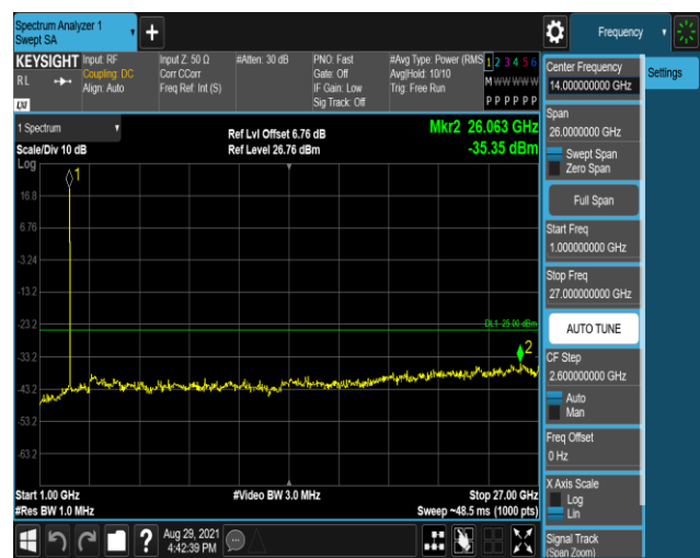
Band38-5MHz-16QAM-38000:1000~27000MHz
