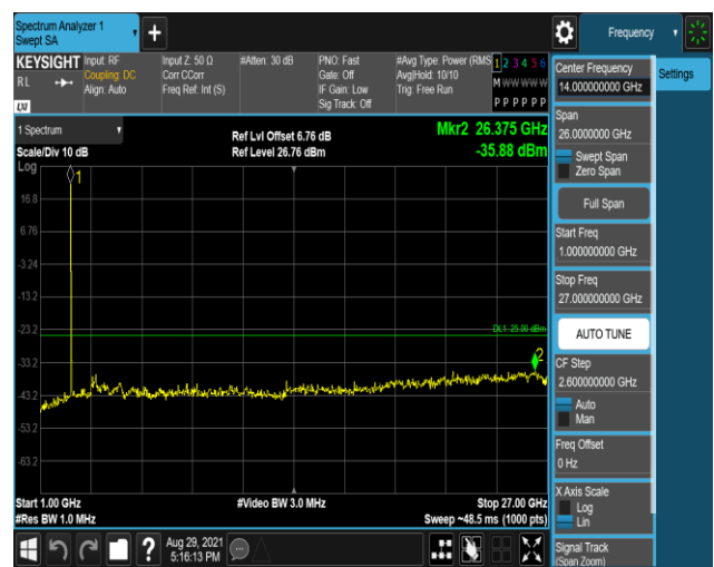
Band38-20MHz-16QAM-38000:1000~27000MHz
