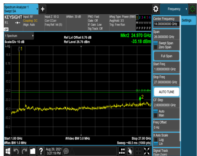
Band7-20MHz-16QAM-21100:1000~27000MHz
