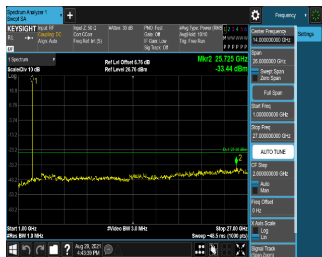
Band38-5MHz-16QAM-38225:1000~27000MHz
