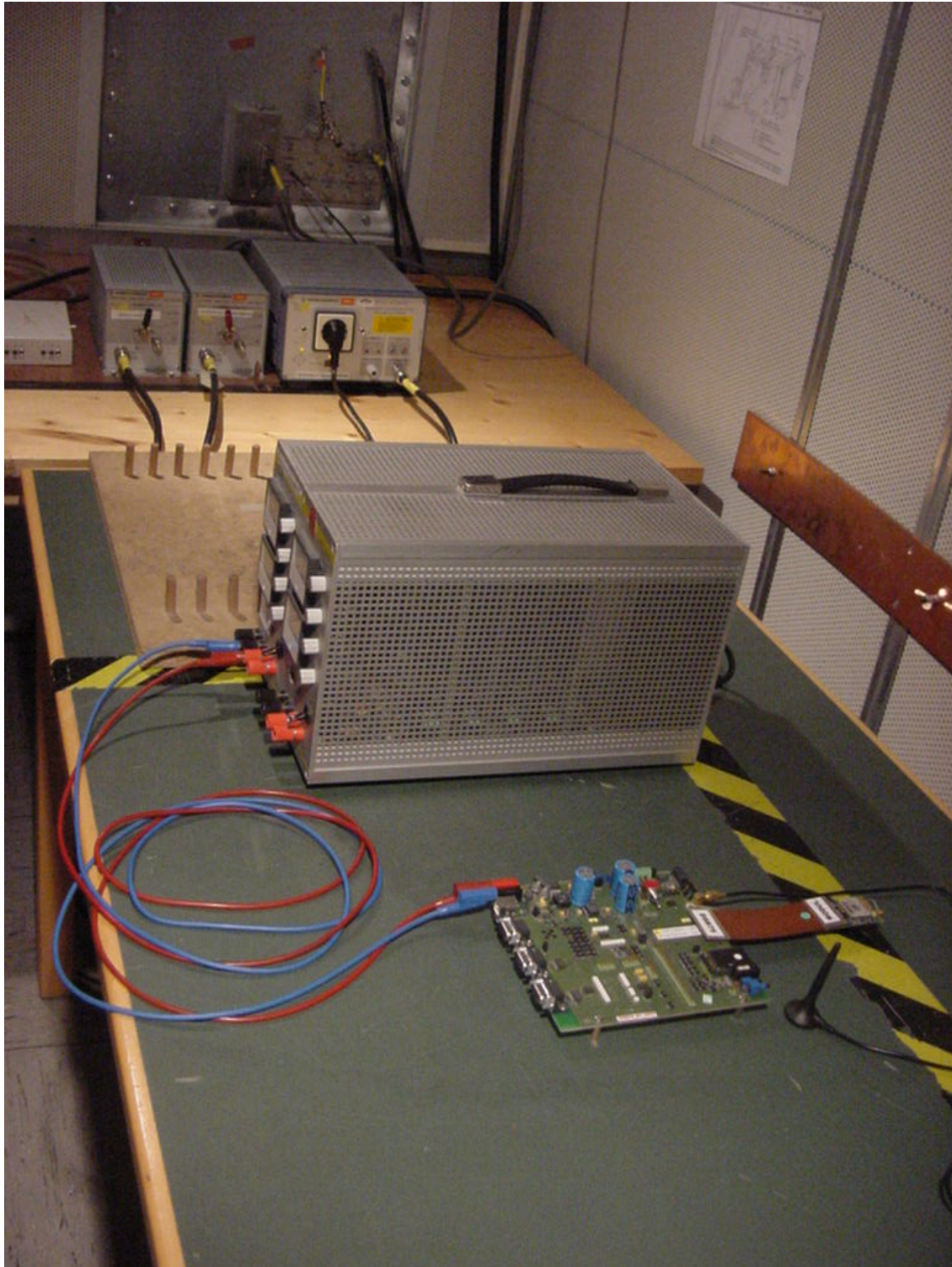
Photo 3 (Conducted Emissions):
