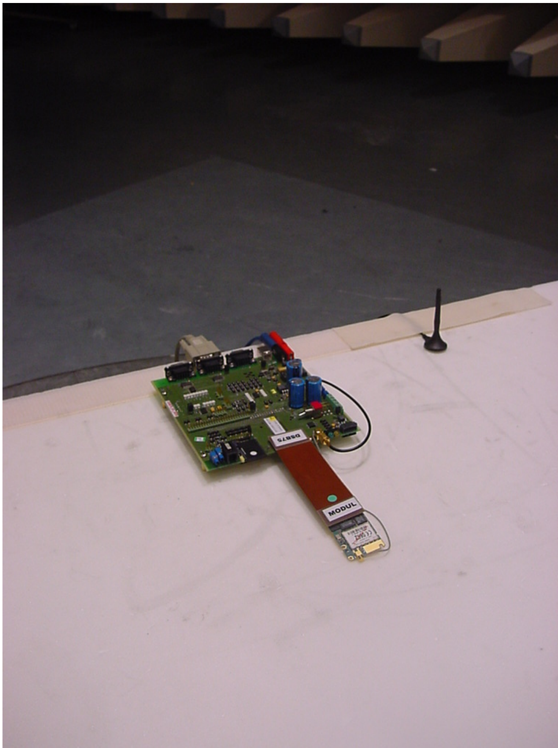
Photo 2 (Radiated Emissions):
