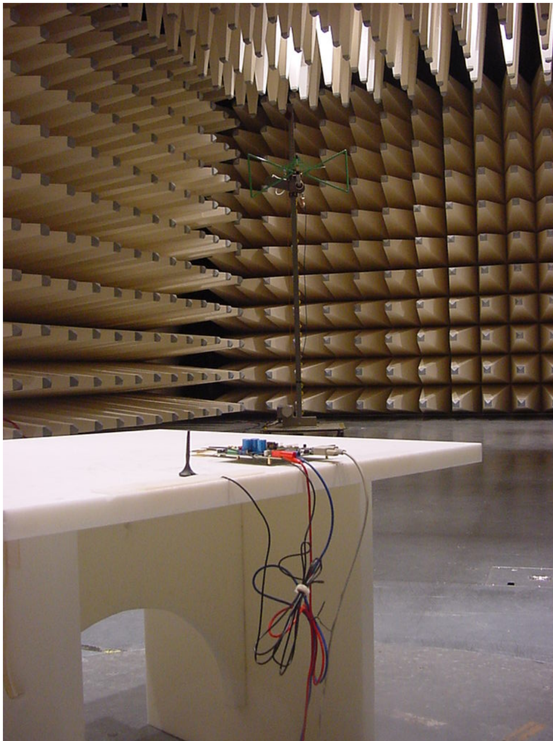
Photo 1 (Radiated Emissions):
