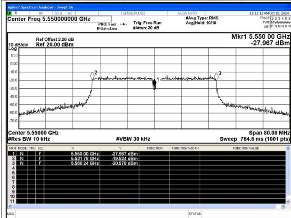
Freq. Stability NVNT ac40 5550MHz Ant1
