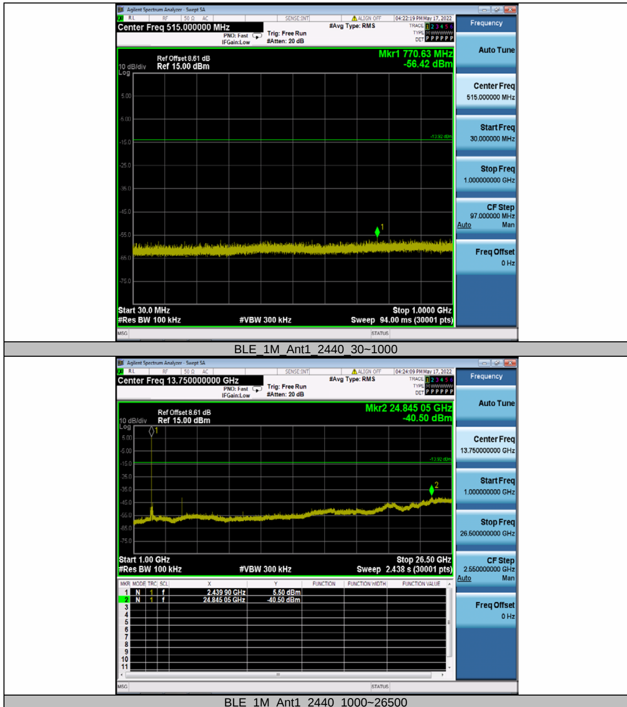
BLE_1M_Ant1_2440_1000~26500
