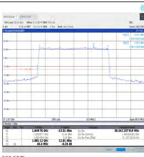
1-N25-15-40-L-7-CP-16QAM-Outer_Full-216@0-Ant 1-38.542-40.400-≤40-PASS
