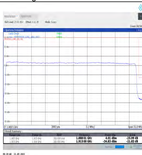
1-N25-15-30-H-3-DFT-PI2BPSK-Outer_Full-160@0-Ant1-seegraph-PASS-see graph
