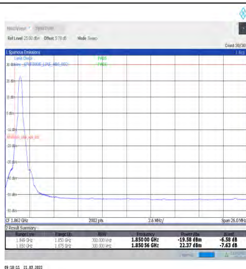
1-N25-15-25-L-1-DFT-PI2BPSK-Edge_1RB_Left-1@0-Ant1-seegraph-PASS-see graph
