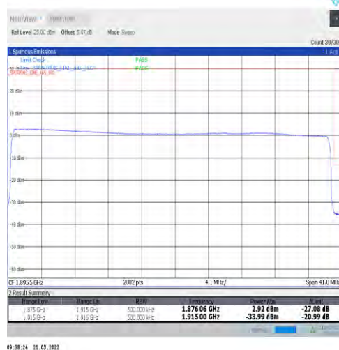
1-N25-15-40-H-6-CP-QPSK-Outer_Full-216@0-Ant1-seegraph-PASS-see graph
