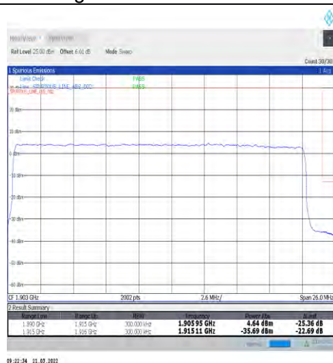
1-N25-15-25-H-3-DFT-PI2BPSK-Outer_Full-128@0-Ant1-seegraph-PASS-see graph
