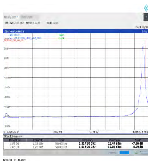
1-N25-15-40-H-2-DFT-PI2BPSK-Edge_1RB_Right-1@215-Ant1-seegraph-PASS-see graph
