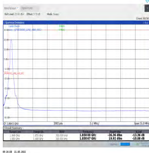
1-N25-15-30-L-4-CP-QPSK-Edge_1RB_Left-1@0-Ant1-seegraph-PASS-see graph
