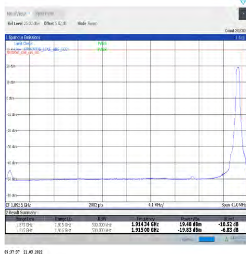
1-N25-15-40-H-5-CP-QPSK-Edge_1RB_Right-1@215-Ant1-seegraph-PASS-see graph
