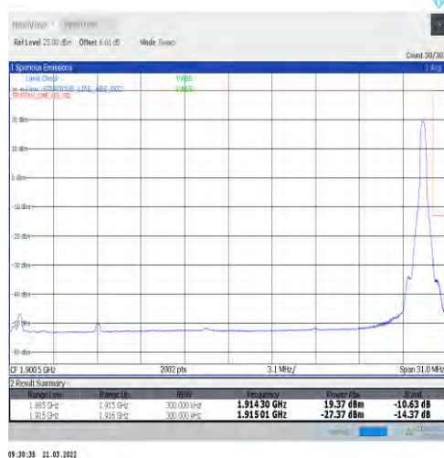
1-N25-15-30-H-5-CP-QPSK-Edge_1RB_Right-1@159-Ant1-seegraph-PASS-see graph
