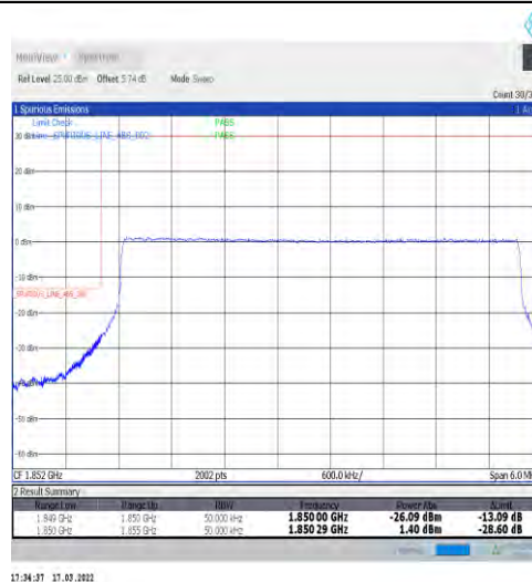
1-N25-15-5-L-6-CP-QPSK-Outer_Full-25@0-Ant1-seegraph-PASS-see graph
