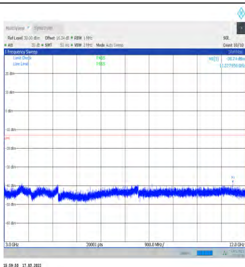
1-N25-15-40-L-1-DFT-PI2BPSK-Inner_1RB_Left-1@ 1-3000-12000-Ant1--38.74--13-PASS
