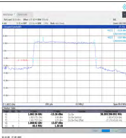
1-N25-15-40-M-6-CP-QPSK-Outer_Full-216@0-Ant1 -38.595-40.400-≤40-PASS
