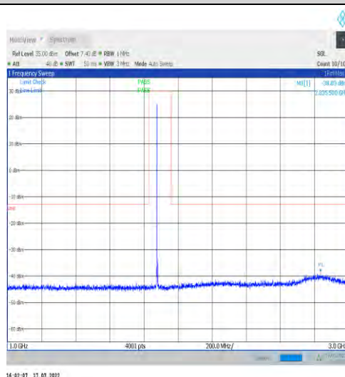
1-N25-15-40-H-1-DFT-PI2BPSK-Inner_1RB_Left-1@ 1-1000-3000-Ant1--38.80--13-PASS
