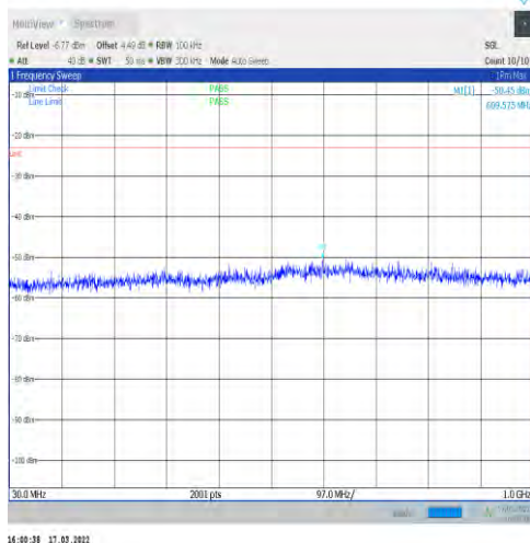
1-N25-15-40-M-1-DFT-PI2BPSK-Inner_1RB_Left-1 @1-30-1000-Ant1--50.45--23-PASS
