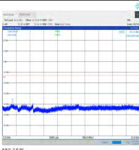
1-N25-15-40-M-1-DFT-PI2BPSK-Inner_1RB_Left-1 @1-3000-12000-Ant1--39.14--13-PASS
