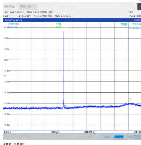
1-N25-15-40-M-1-DFT-PI2BPSK-Inner_1RB_Left-1@ 1-1000-3000-Ant1--39.03--13-PASS
