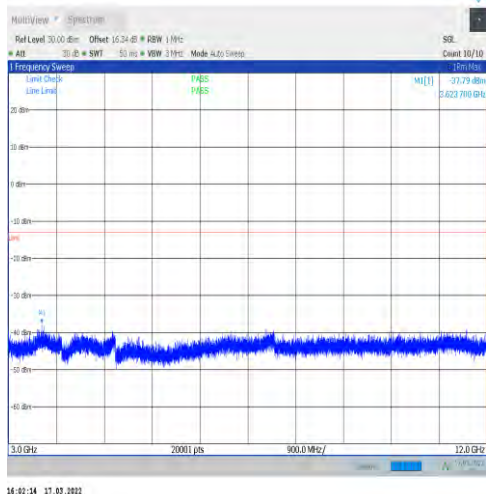
1-N25-15-40-H-1-DFT-PI2BPSK-Inner_1RB_Left-1 @1-3000-12000-Ant1--37.79--13-PASS
