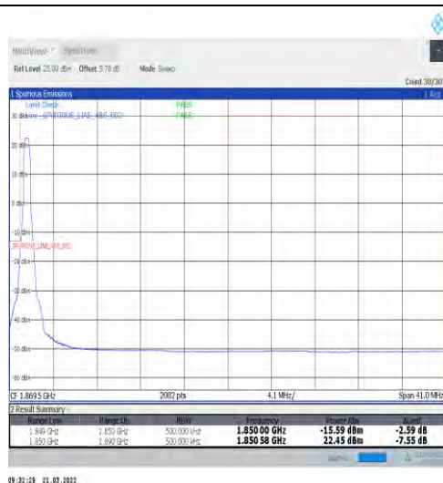
1-N25-15-40-L-1-DFT-PI2BPSK-Edge_1RB_Left-1@0-Ant1-seegraph-PASS-see graph
