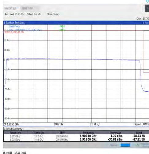
1-N25-15-20-H-6-CP-QPSK-Outer_Full-106@0-Ant1-seegraph-PASS-see graph
