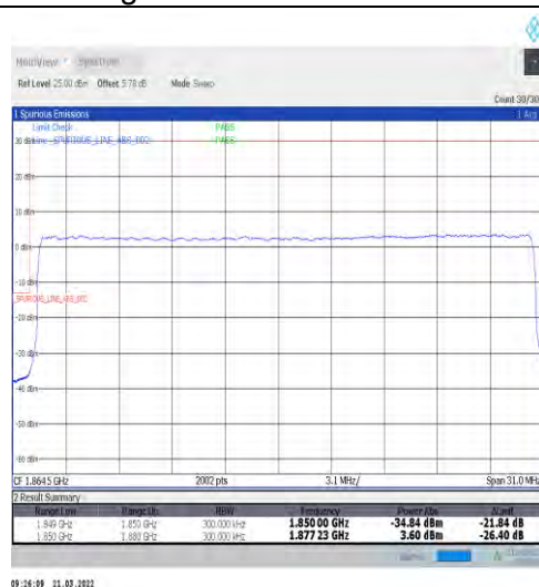
1-N25-15-30-L-3-DFT-PI2BPSK-Outer_Full-160@0-Ant1-seegraph-PASS-see graph
