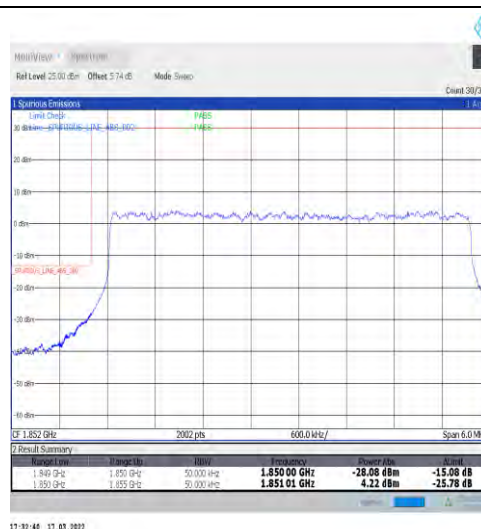
1-N25-15-5-L-3-DFT-PI2BPSK-Outer_Full-25@0-Ant1-seegraph-PASS-see graph
