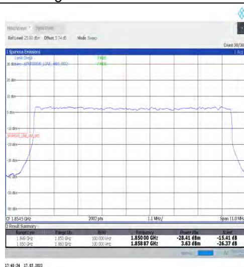
1-N25-15-10-L-3-DFT-PI2BPSK-Outer_Full-50@0-Ant1-seegraph-PASS-see graph
