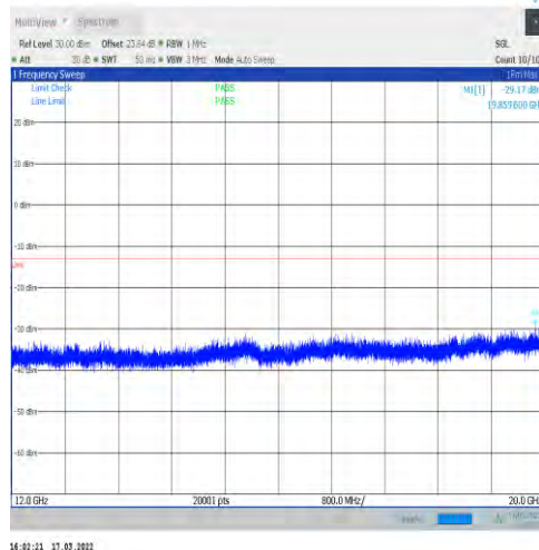
1-N25-15-40-H-1-DFT-PI2BPSK-Inner_1RB_Left-1@ 1-12000-20000-Ant1--29.17--13-PASS
