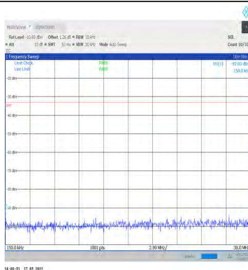
1-N25-15-40-M-1-DFT-PI2BPSK-Inner_1RB_Left-1@ 1-0.15-30-Ant1--92.03--33-PASS
