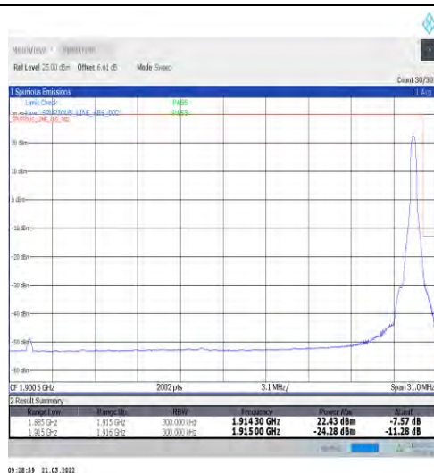
1-N25-15-30-H-2-DFT-PI2BPSK-Edge_1RB_Right-1@159-Ant1-seegraph-PASS-see graph
