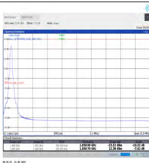
1-N25-15-30-L-1-DFT-PI2BPSK-Edge_1RB_Left-1@0-Ant1-seegraph-PASS-see graph
