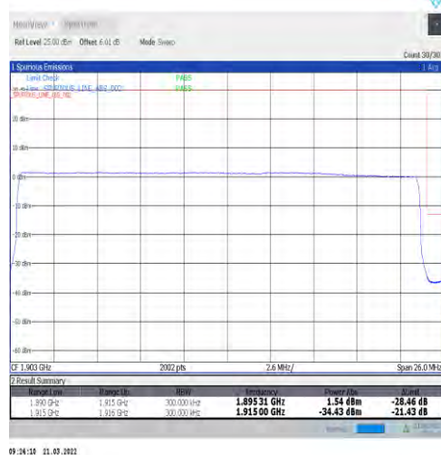
1-N25-15-25-H-6-CP-QPSK-Outer_Full-133@0-Ant1-seegraph-PASS-see graph
