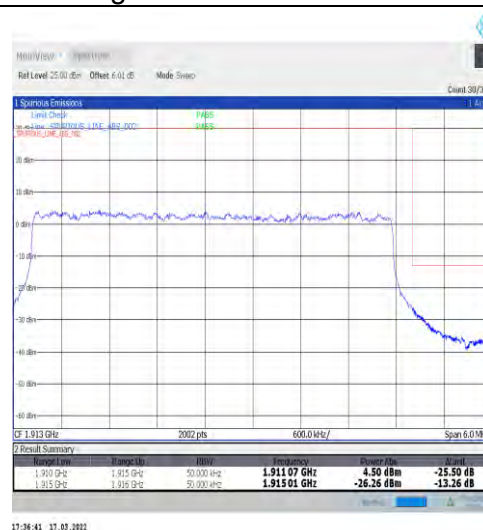
1-N25-15-5-H-3-DFT-PI2BPSK-Outer_Full-25@0-Ant1-seegraph-PASS-see graph
