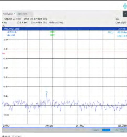
1-N25-15-40-M-1-DFT-PI2BPSK-Inner_1RB_Left-1@ 1-0.009-0.15-Ant1--88.72--43-PASS
