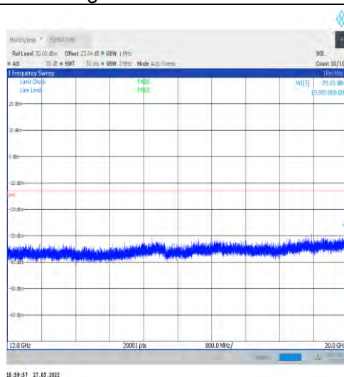
1-N25-15-40-L-1-DFT-PI2BPSK-Inner_1RB_Left-1@ 1-12000-20000-Ant1--29.15--13-PASS
