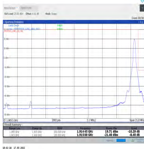
1-N25-15-20-H-5-CP-QPSK-Edge_1RB_Right-1@105-Ant1-seegraph-PASS-see graph
