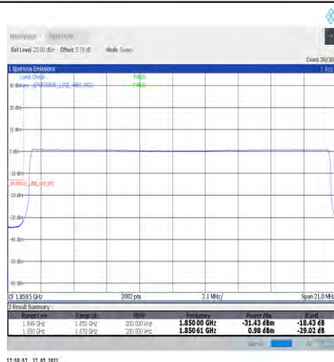
1-N25-15-20-L-6-CP-QPSK-Outer_Full-106@0-Ant1-seegraph-PASS-see graph
