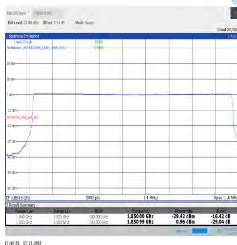
1-N25-15-10-L-6-CP-QPSK-Outer_Full-52@0-Ant1-seegraph-PASS-see graph
