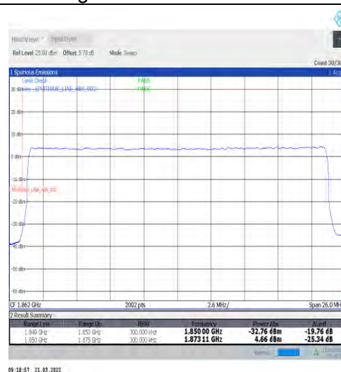
1-N25-15-25-L-3-DFT-PI2BPSK-Outer_Full-128@0-Ant1-seegraph-PASS-see graph
