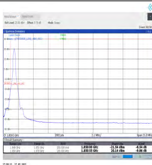
1-N25-15-20-L-4-CP-QPSK-Edge_1RB_Left-1@0-Ant1-seegraph-PASS-see graph
