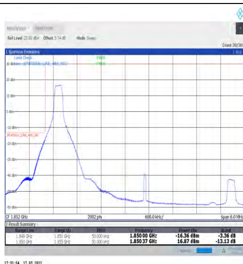
1-N25-15-5-L-1-DFT-PI2BPSK-Edge_1RB_Left-1@0-A nt1-seegraph-PASS-see graph
