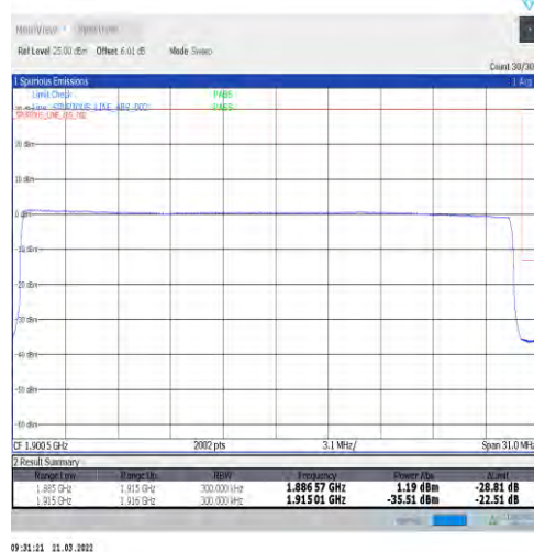
1-N25-15-30-H-6-CP-QPSK-Outer_Full-160@0-Ant1-seegraph-PASS-see graph
