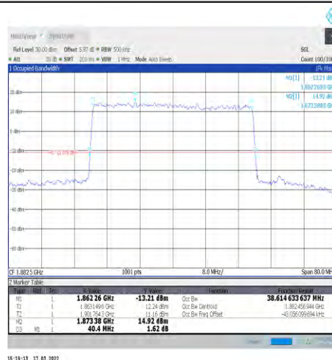
1-N25-15-40-M-1-DFT-QPSK-Outer_Full-216@0-Ant 1-38.615-40.400-≤40-PASS
