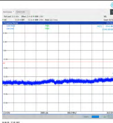
1-N25-15-40-M-1-DFT-PI2BPSK-Inner_1RB_Left-1@ 1-12000-20000-Ant1--29.41--13-PASS
