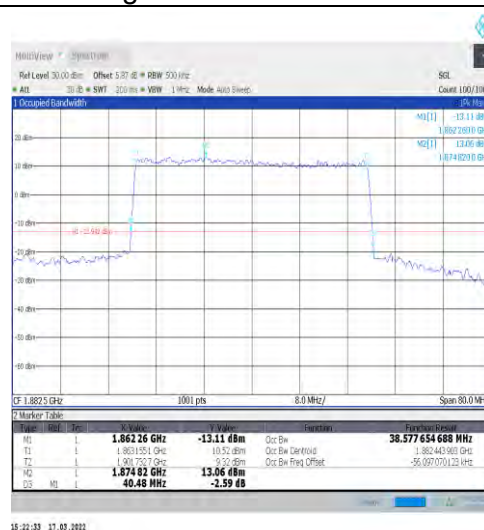
1-N25-15-40-M-7-CP-16QAM-Outer_Full-216@0-Ant1 1-38.578-40.480-≤40-PASS
