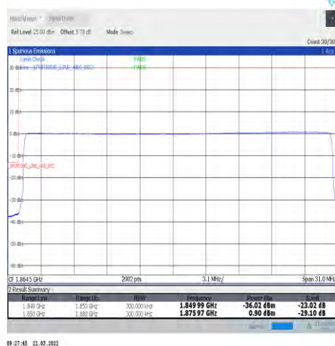
1-N25-15-30-L-6-CP-QPSK-Outer_Full-160@0-Ant1-seegraph-PASS-see graph
