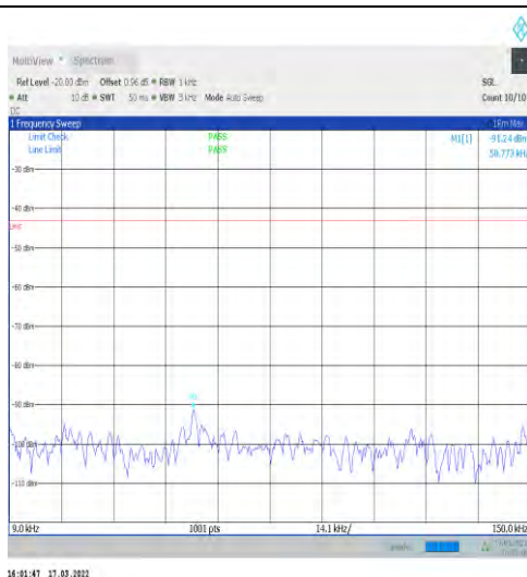
1-N25-15-40-H-1-DFT-PI2BPSK-Inner_1RB_Left-1 @1-0.009-0.15-Ant1--91.24--43-PASS
