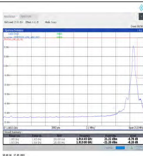
1-N25-15-20-H-2-DFT-PI2BPSK-Edge_1RB_Right-1@105-Ant1-seegraph-PASS-see graph
