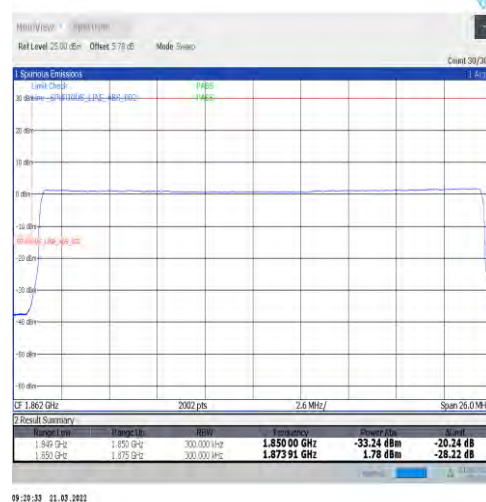
1-N25-15-25-L-6-CP-QPSK-Outer_Full-133@0-Ant1-seegraph-PASS-see graph
