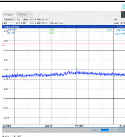
1-N25-15-40-H-1-DFT-PI2BPSK-Inner_1RB_Left-1 @1-30-1000-Ant1--50.08--23-PASS
