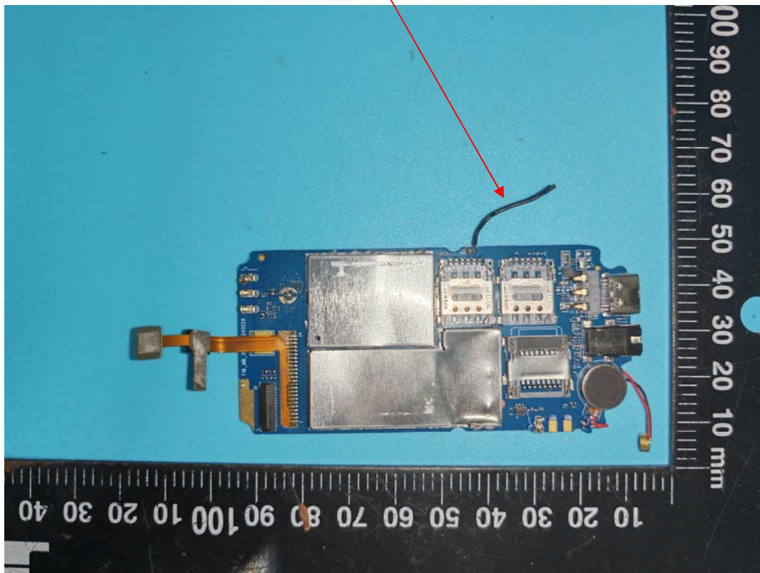
BT Antenna
