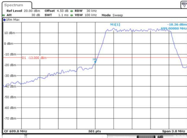
1.4M, 16QAM, Left Band Edge
