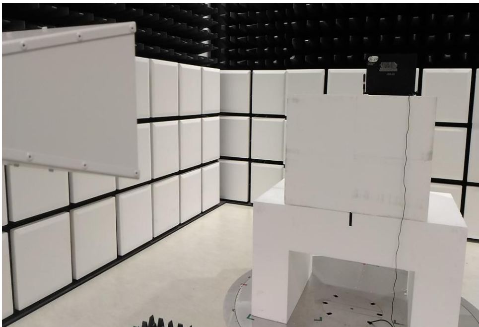
Above 1 GHz _ Rear View
