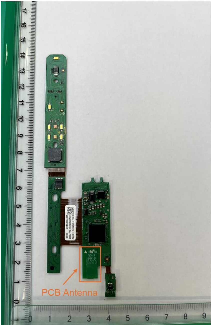
Figure 2: Back side of the PCBs, indicating the back of the PCB antenna.
