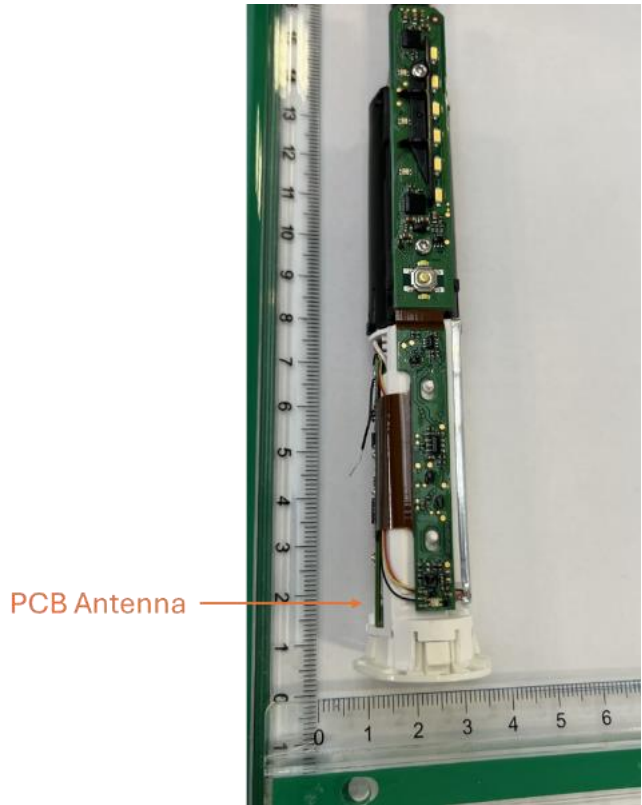
Figure 4: PCBA mounted on the front of the chassis.
