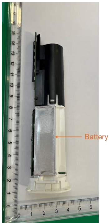
Figure 6: Battery of the device mounted on the side of the chassis ( the PCB antenna is placed on the opposite side of the battery ).
