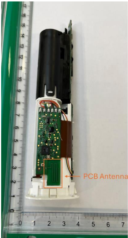
Figure 3: PCBA mounted on the side of the chassis, indicating the PCB Antenna.
