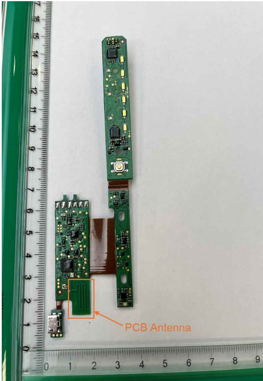
Figure 1: Top of the PCBs, indicating the PCB antenna.
