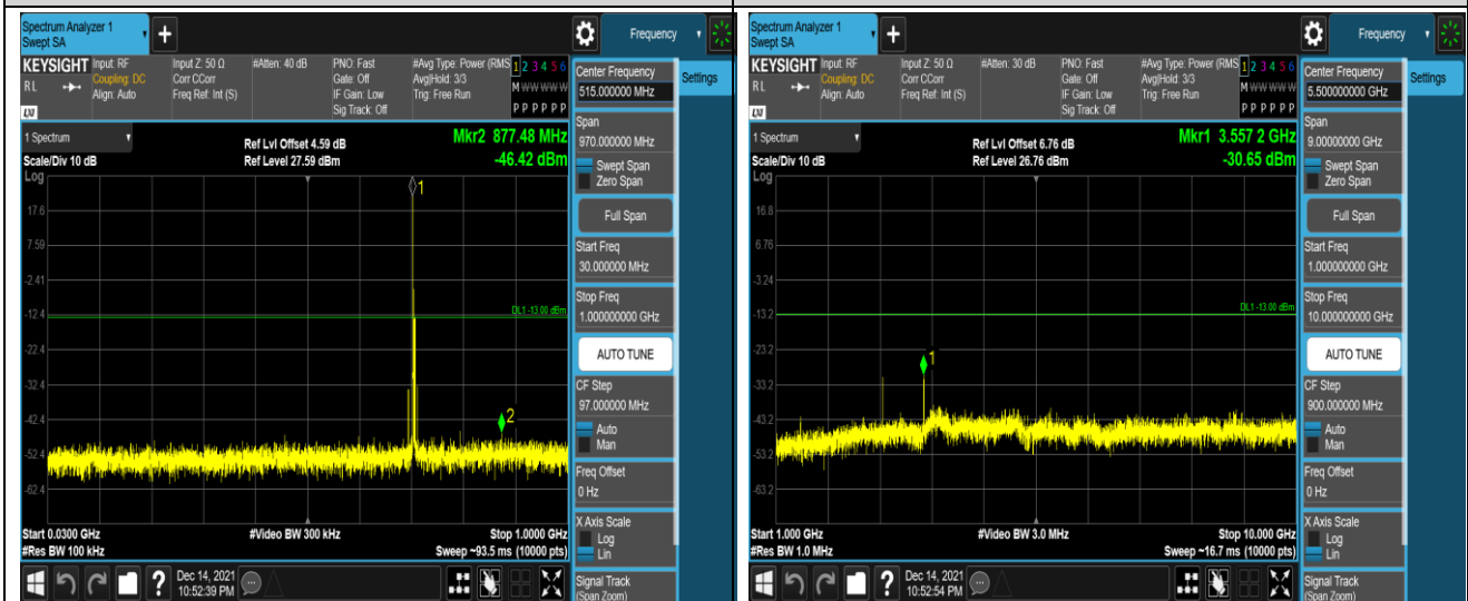
Band17-5MHz-QPSK-23790-1RB#0-Range1:30~10 00MHz
