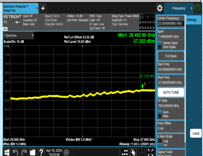
Band7_5MHz_QPSK_21425_1RB#0_20000~27000_20000~27000
