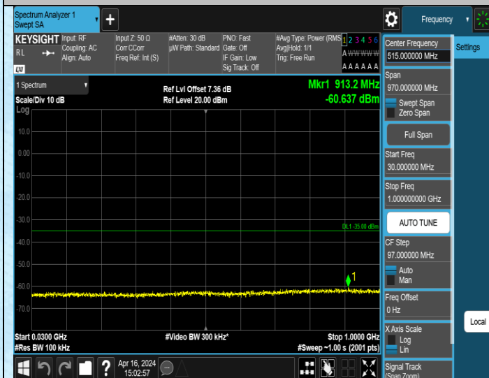
Band7_5MHz_QPSK_21425_1RB#0_30~1000_30~1000
