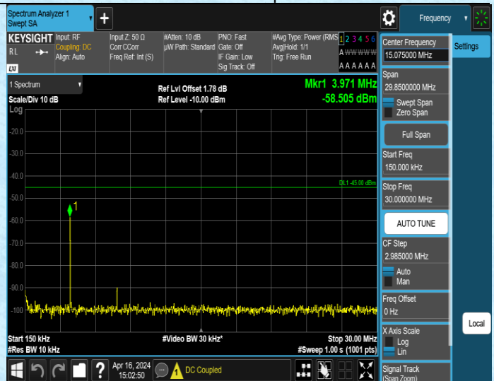
Band7_5MHz_QPSK_21425_1RB#0_0.15~30_0.15~30
