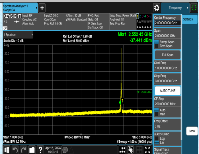
Band7_5MHz_QPSK_21425_1RB#0_1000~3000_1000~3000
