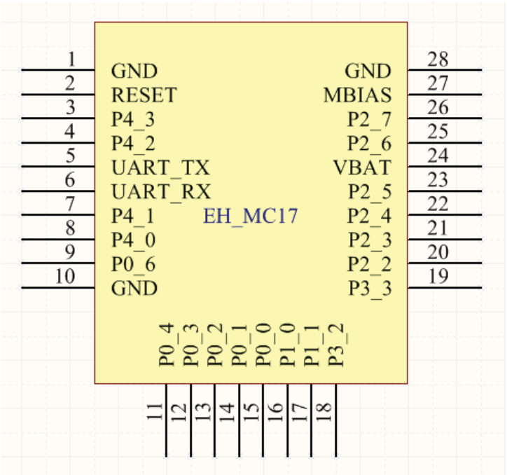
Figure 1: Pinout of EH-MC17
