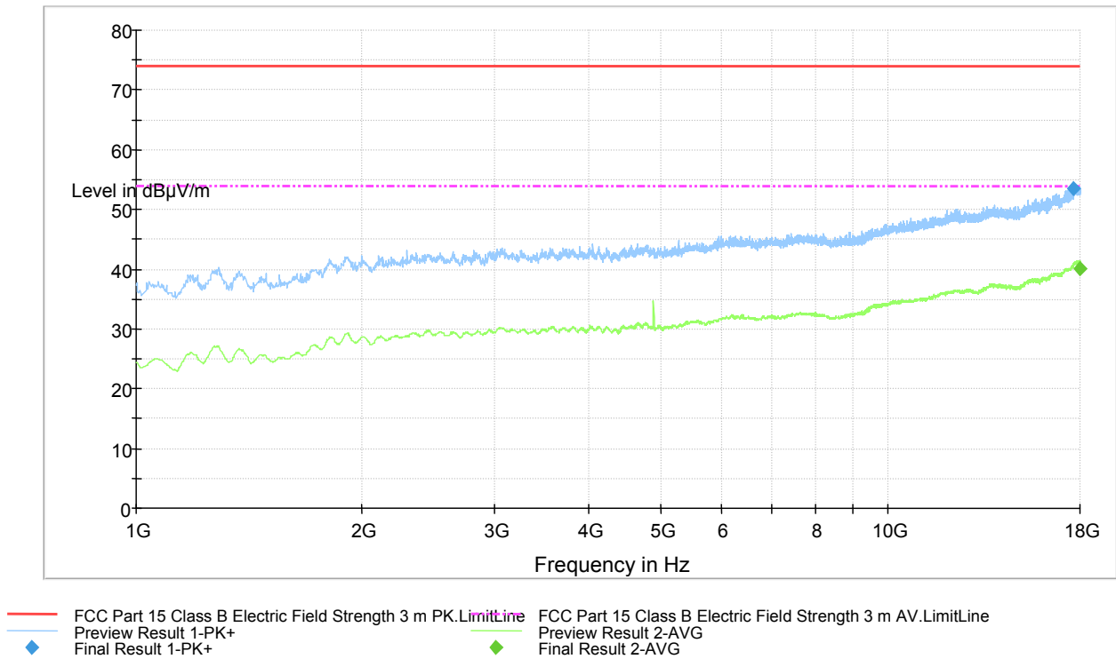
Figure 42. Measured curve with peak-and average detector.
