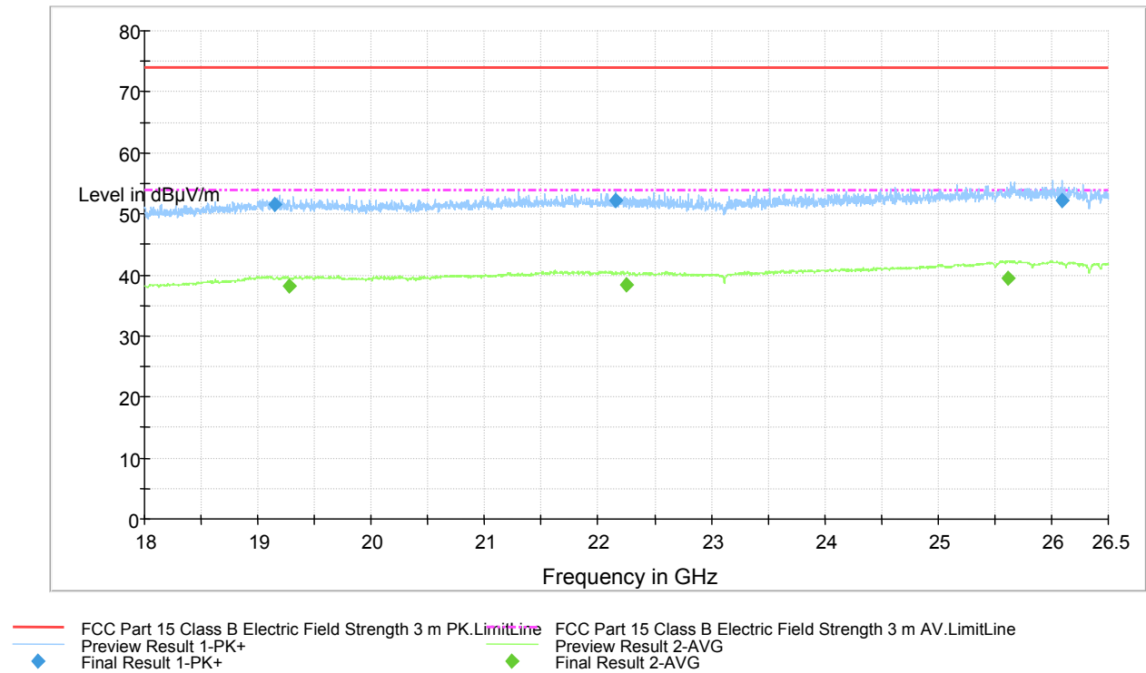
Figure 43. Measured curve with peak-and average detector.
