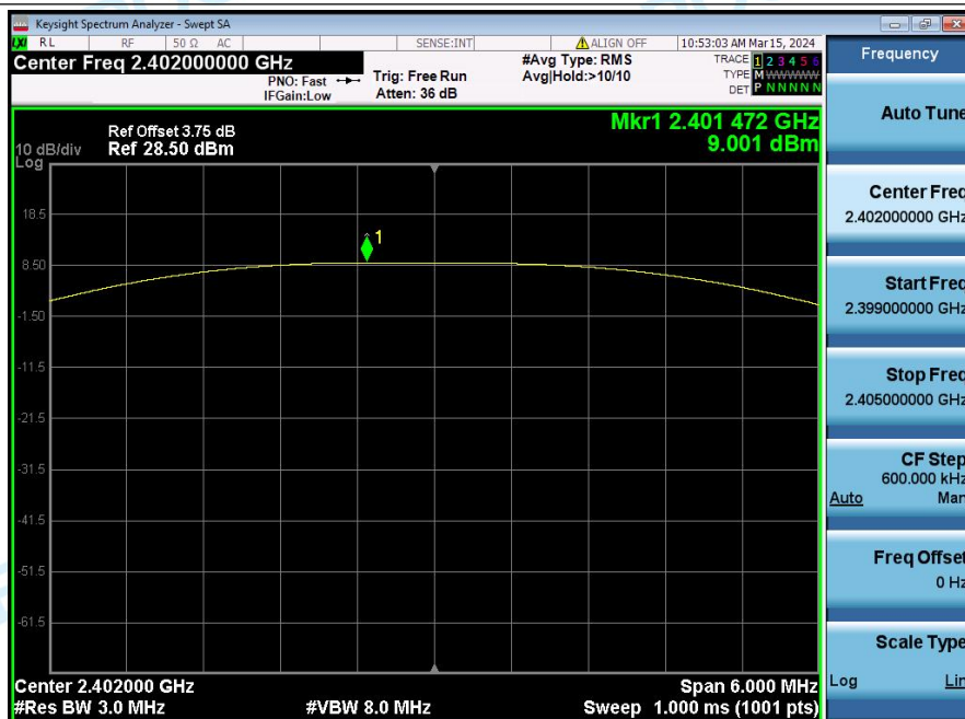
Peak_Output_Power_NVNT_ANT1_2Mbps_2402
