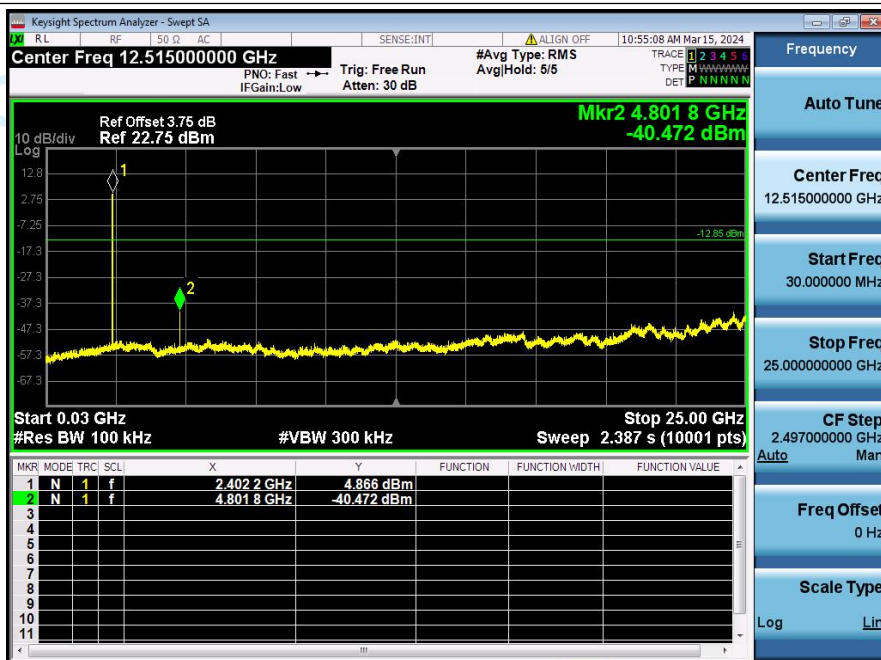
2_Spurious_Emission_NVNT_ANT1_2Mbps_2402
