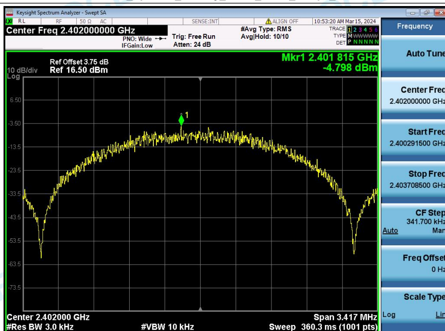
Power_Spectral_Density_NVNT_ANT1_2Mbps_2402
