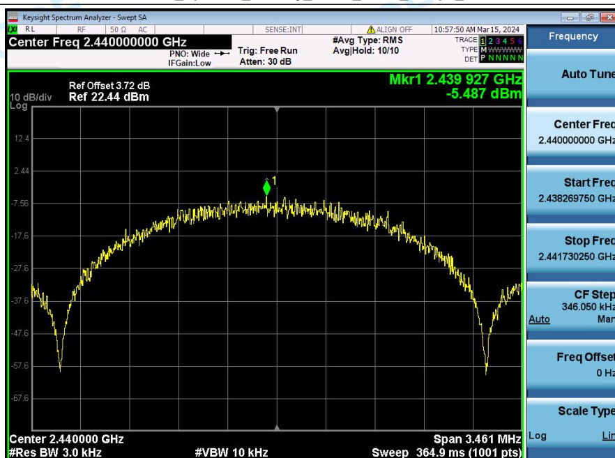
Power_Spectral_Density_NVNT_ANT1_2Mbps_2440
