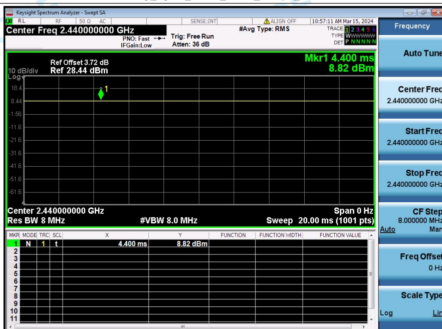
Duty_Cycle_NVNT_ANT1_2Mbps_2440
