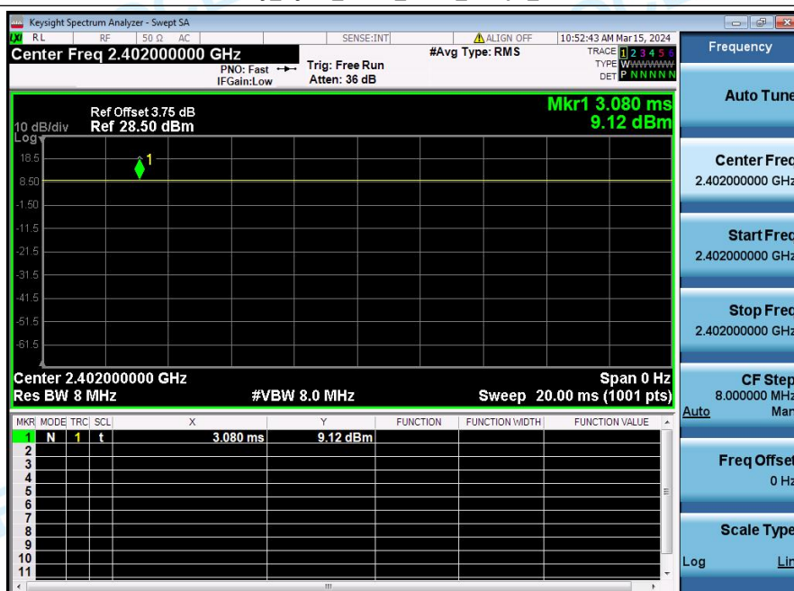
Duty_Cycle_NVNT_ANT1_2Mbps_2402
