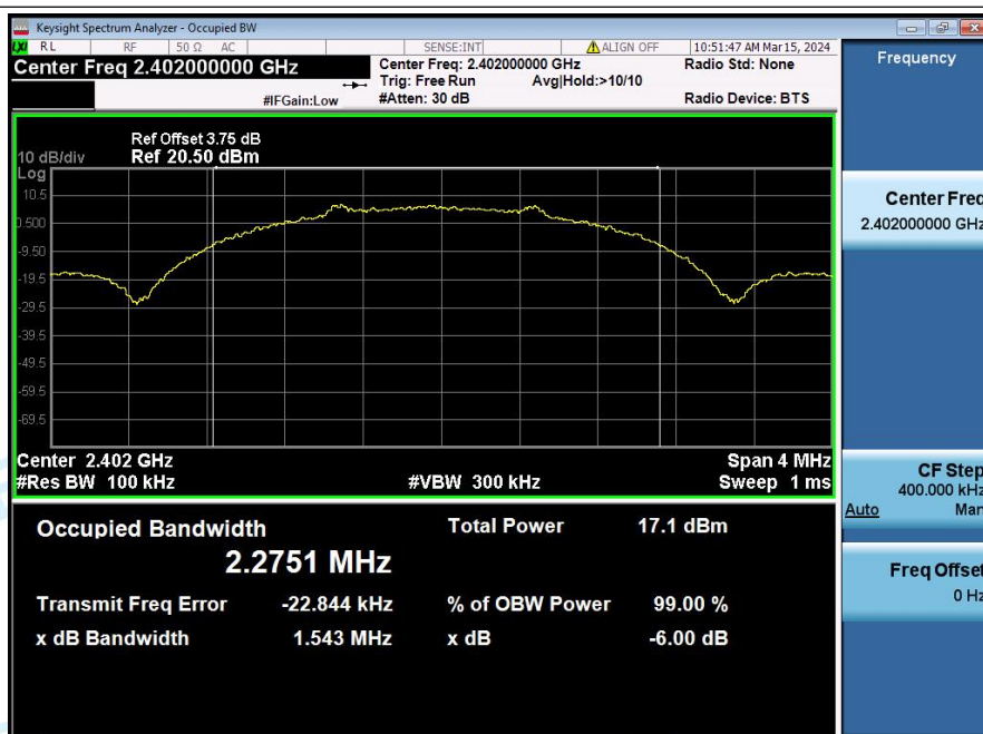
-6dB_Bandwidth_NVNT_ANT1_2Mbps_2402
