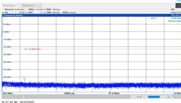
Band2-3MHz-QPSK-19185-1RB#0-30~1000-PASS
