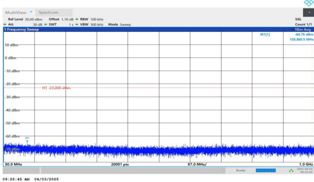
Band2-1.4MHz-QPSK-18900-1RB#0-30~1000-PASS
