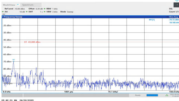
Band2-5MHz-QPSK-18900-1RB#0-0.009~0.15-PASS
