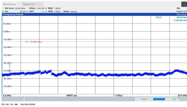
Band2-5MHz-QPSK-18625-1RB#0-3000~20000-PASS
