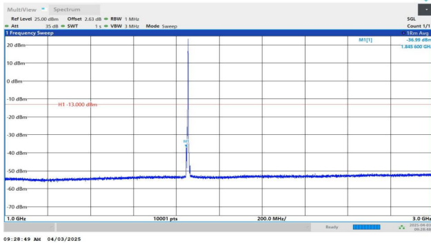
Band2-5MHz-QPSK-18625-1RB#24-1000~3000-PASS
