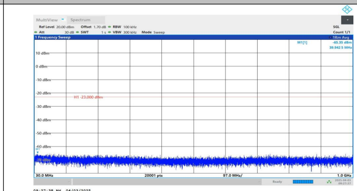
Band2-3MHz-QPSK-18900-1RB#14-30~1000-PASS
