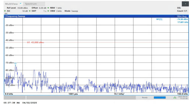
Band2-3MHz-QPSK-18615-1RB#14-0.009~0.15-PASS
