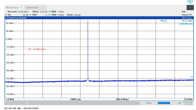
Band2-1.4MHz-QPSK-18900-1RB#0-1000~3000-PASS
