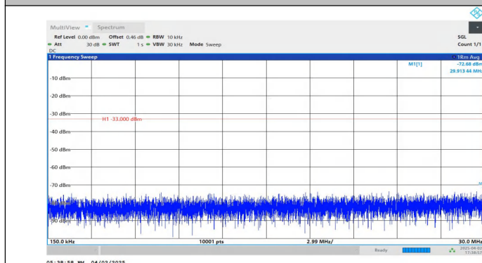
Band2-3MHz-QPSK-18900-1RB#14-0.15~30-PASS
