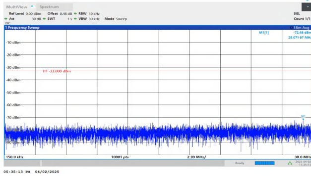
Band2-1.4MHz-QPSK-18900-1RB#5-0.15~30-PASS
