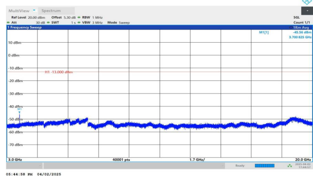
Band2-10MHz-QPSK-18650-1RB#0-3000~20000-PASS
