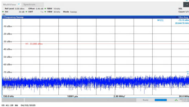
Band2-5MHz-QPSK-18625-1RB#24-0.15~30-PASS
