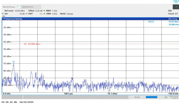
Band2-1.4MHz-QPSK-18900-1RB#0-0.009~0.15-PASS
