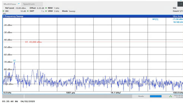
Band2-1.4MHz-QPSK-19193-1RB#0-0.009~0.15-PASS
