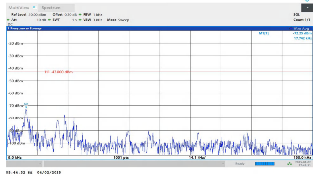
Band2-10MHz-QPSK-18650-1RB#0-0.009~0.15-PASS
