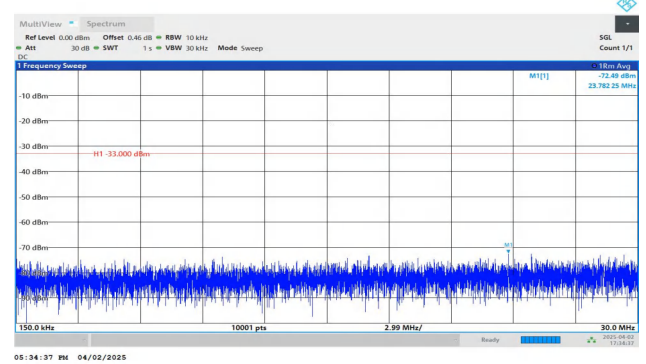
Band2-1.4MHz-QPSK-18900-1RB#0-0.15~30-PASS
