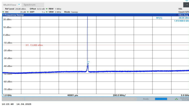
Band2-5MHz-QPSK-19175-1RB#24-1000~3000-PASS
