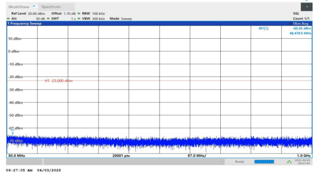
Band2-3MHz-QPSK-18615-1RB#14-30~1000-PASS
