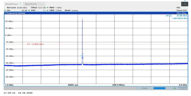
Band2-3MHz-QPSK-18615-1RB#0-1000~3000-PASS
