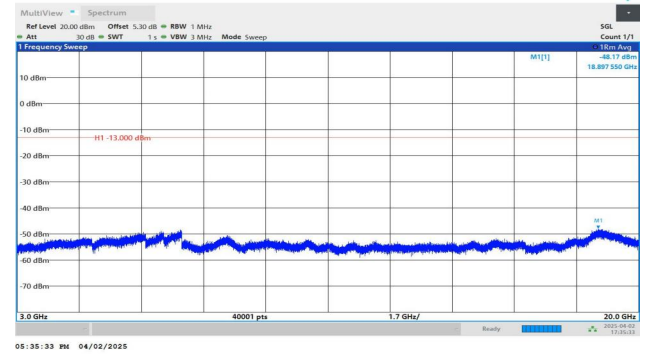
Band2-1.4MHz-QPSK-18900-1RB#5-3000~20000-PASS
