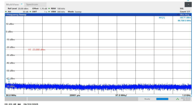
Band2-5MHz-QPSK-19175-1RB#24-30~1000-PASS
