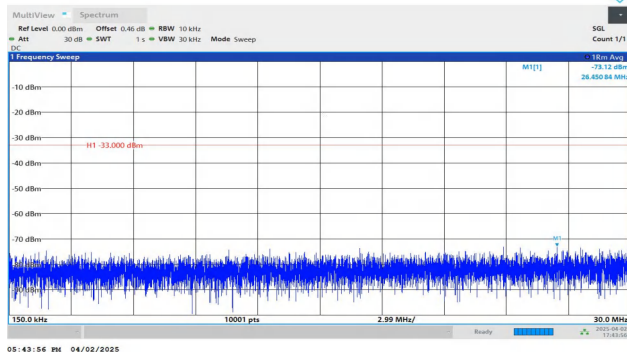
Band2-5MHz-QPSK-19175-1RB#24-0.15~30-PASS
