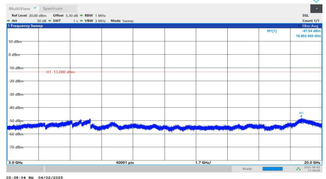
Band2-3MHz-QPSK-18615-1RB#14-3000~20000-PASS
