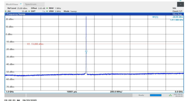
Band2-1.4MHz-QPSK-19193-1RB#0-1000~3000-PASS
