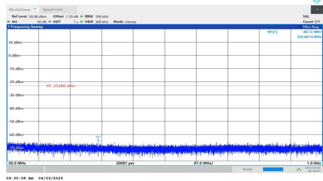
Band2-10MHz-QPSK-18650-1RB#0-30~1000-PASS
