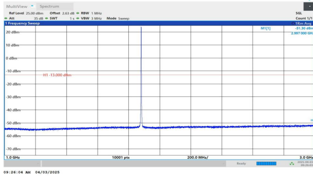
Band2-1.4MHz-QPSK-18900-1RB#5-1000~3000-PASS
