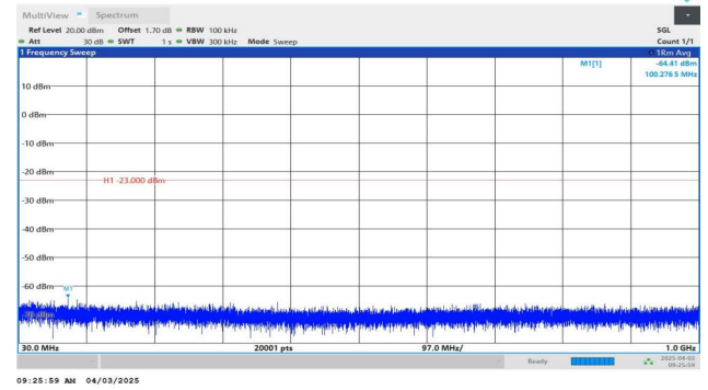
Band2-1.4MHz-QPSK-18900-1RB#5-30~1000-PASS
