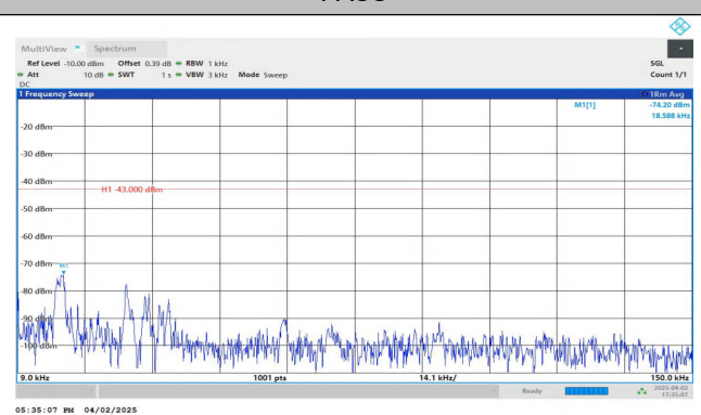
Band2-1.4MHz-QPSK-18900-1RB#5-0.009~0.15-PASS
