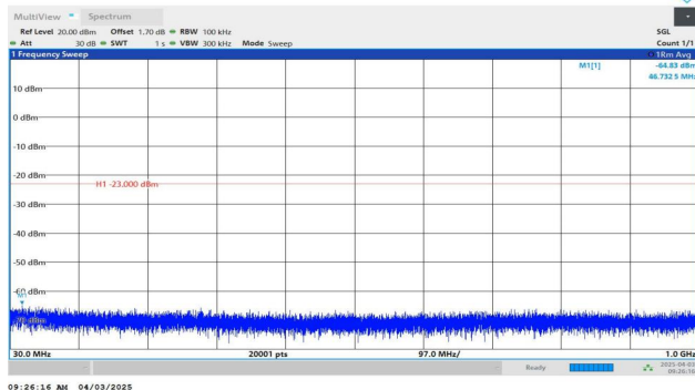
Band2-1.4MHz-QPSK-19193-1RB#0-30~1000-PASS
