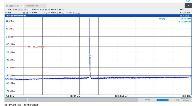
Band2-3MHz-QPSK-19185-1RB#0-1000~3000-PASS
