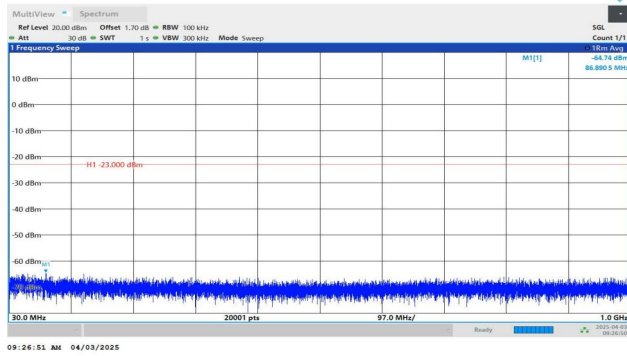
Band2-3MHz-QPSK-18615-1RB#0-30~1000-PASS
