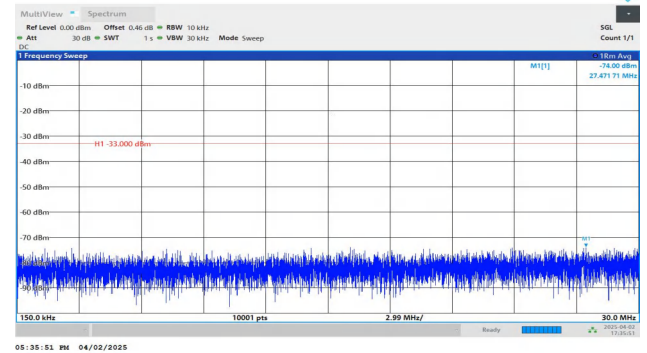
Band2-1.4MHz-QPSK-19193-1RB#0-0.15~30-PASS
