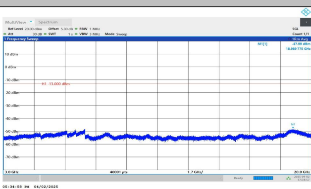
Band2-1.4MHz-QPSK-18900-1RB#0-3000~20000-PASS
