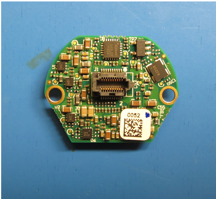
922381_Camera-Board_Portrait_BOTTOM
