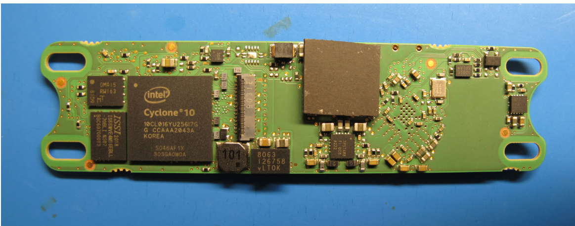
880880_Master_Radar-Board_BOTTOM
