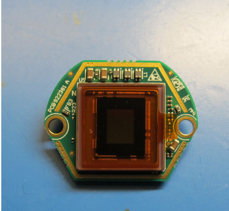
922381_Camera-Board_Portrait_TOP
