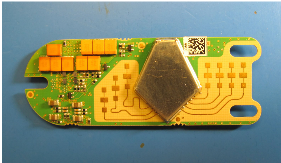
880870_Slave_Radar-Board_TOP-w/o shielding
