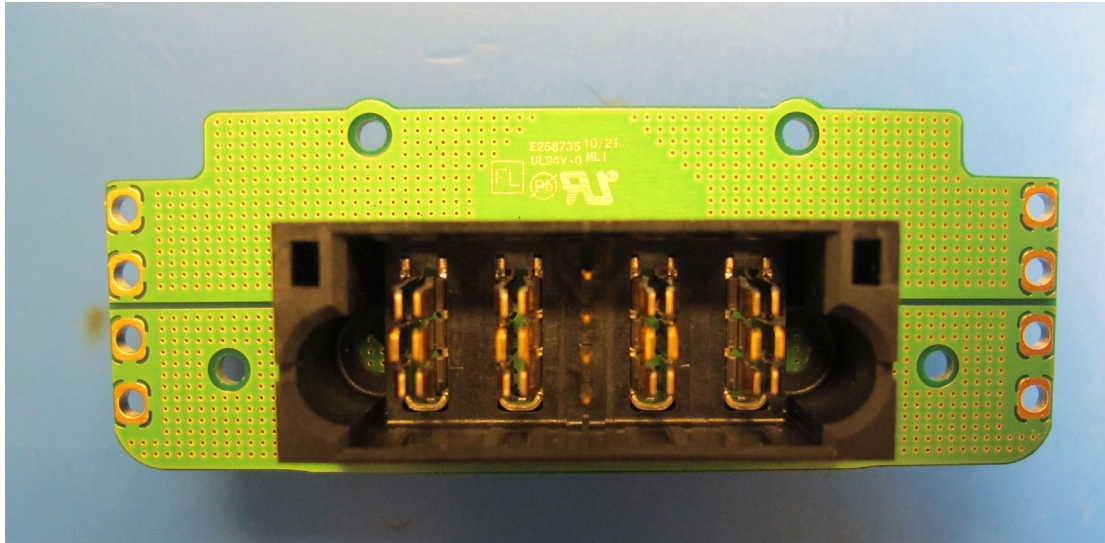
906419_Battery-Connector-Board_TOP
