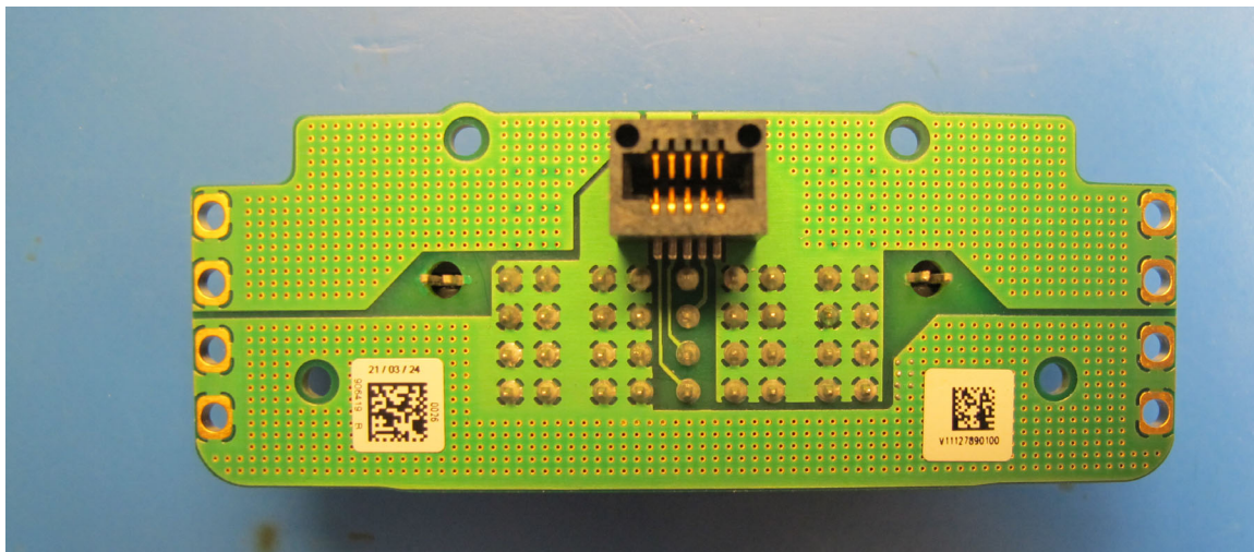
906419_Battery-Connector-Board_BOTTOM
