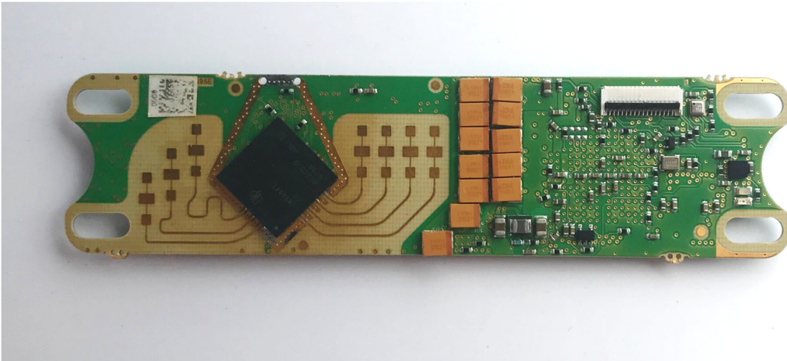
880880_Master_Radar-Board_BOTTOM
