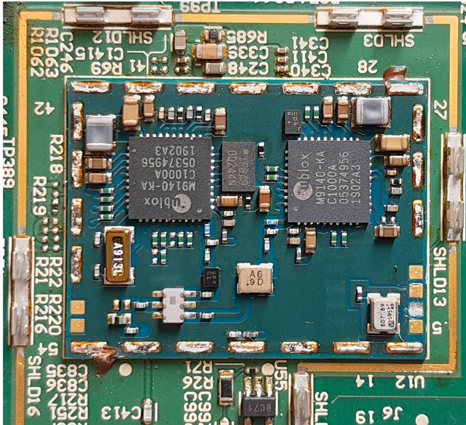
892583_Mainboard_Top – u-Blox ZED-F9P-02B-00 w-o shielding
