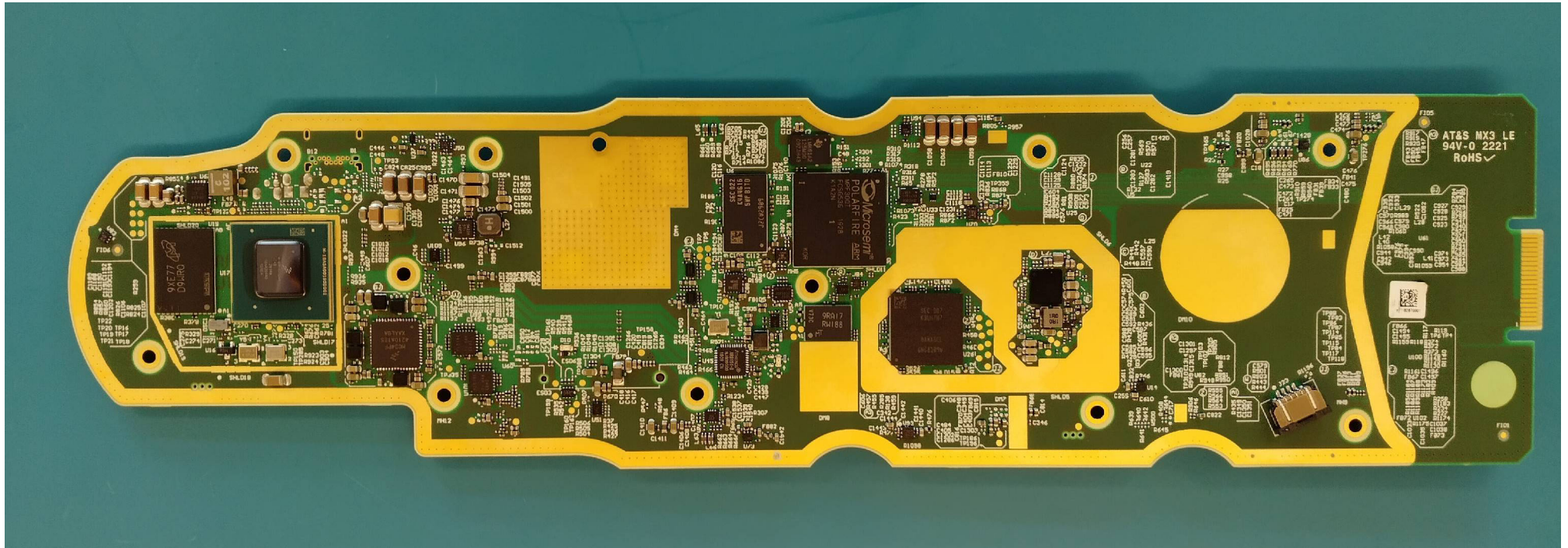
892583_Mainboard_Bottom
