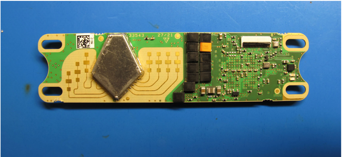
880880_Master_Radar-Board_TOP – w/o shielding
