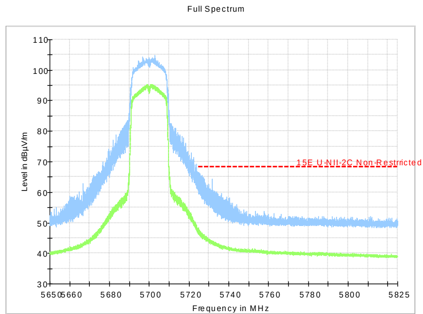
Fig.41 Band Edges (802.11n-HT20, 5700MHz)
