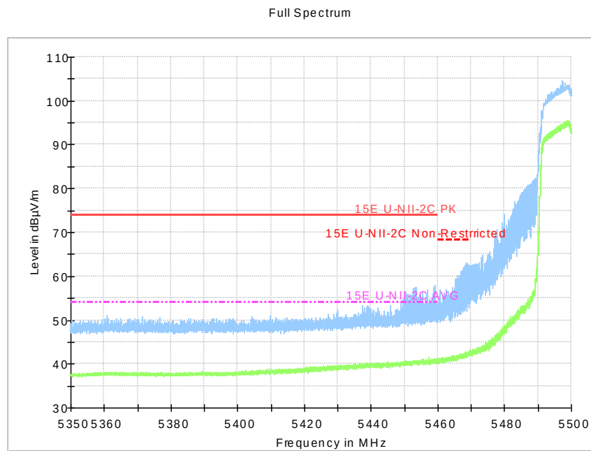
Fig.40 Band Edges (802.11n-HT20, 5500MHz)
