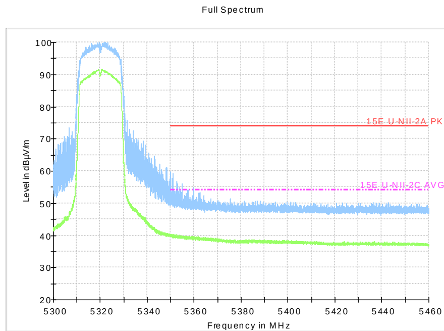
Fig.39 Band Edges (802.11n-HT20, 5320MHz)
