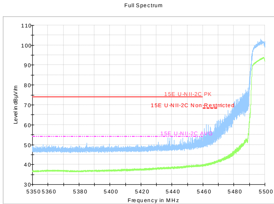
Fig.36 Band Edges (802.11a, 5500MHz)
