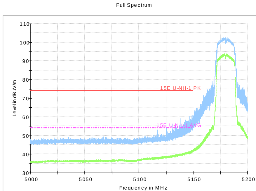
Fig.34 Band Edges (802.11a, 5180MHz)
