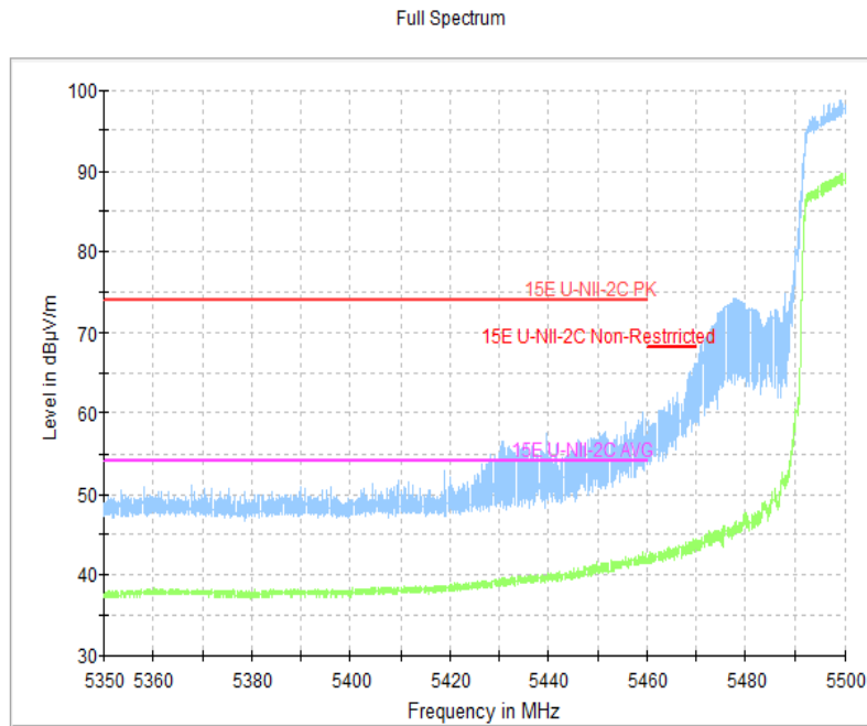
Fig.44 Band Edges (802.11n-HT40, 5510MHz)
