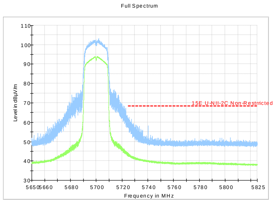
Fig.49 Band Edges (802.11ac-HT20, 5700MHz)
