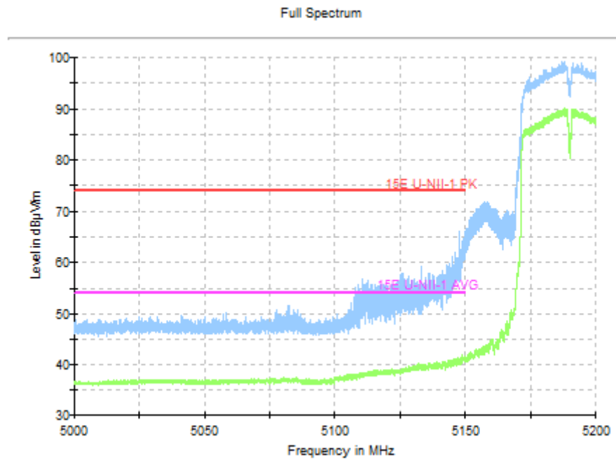
Fig.42 Band Edges (802.11n-HT40, 5190MHz)
