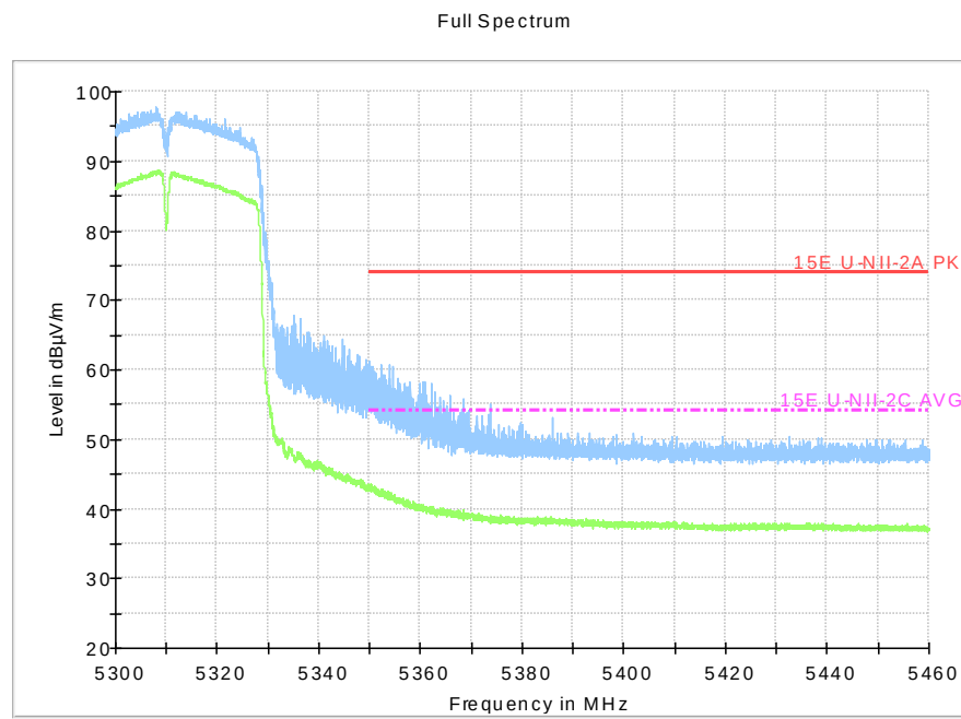
Fig.51 Band Edges (802.11ac-HT40, 5310MHz)
