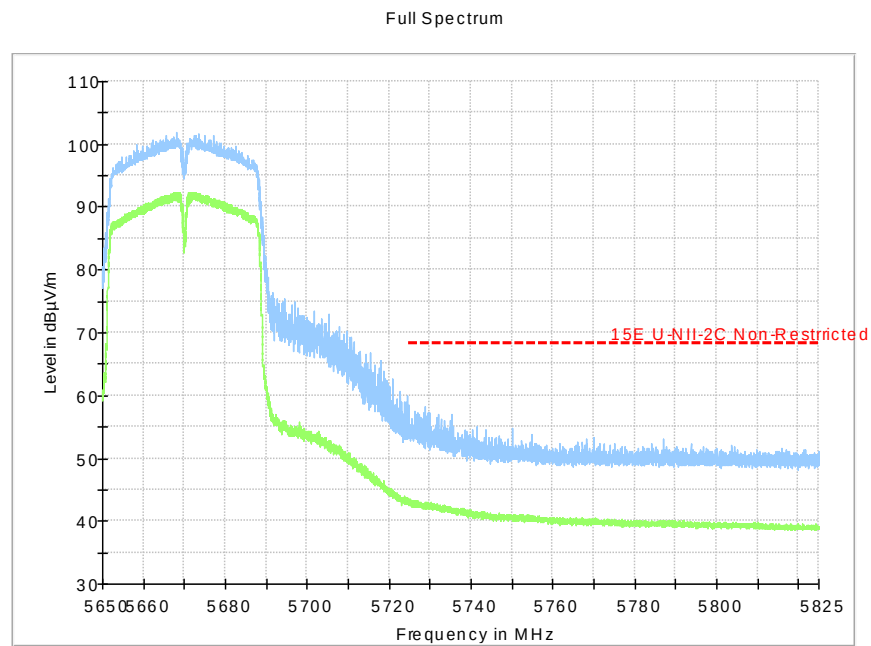
Fig.53 Band Edges (802.11ac-HT40, 5670MHz)
