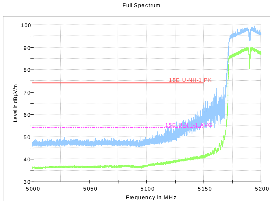
Fig.50 Band Edges (802.11ac-HT40, 5190MHz)
