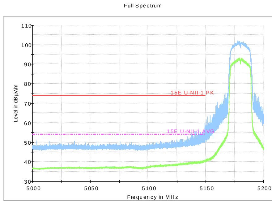
Fig.46 Band Edges (802.11ac-HT20, 5180MHz)
