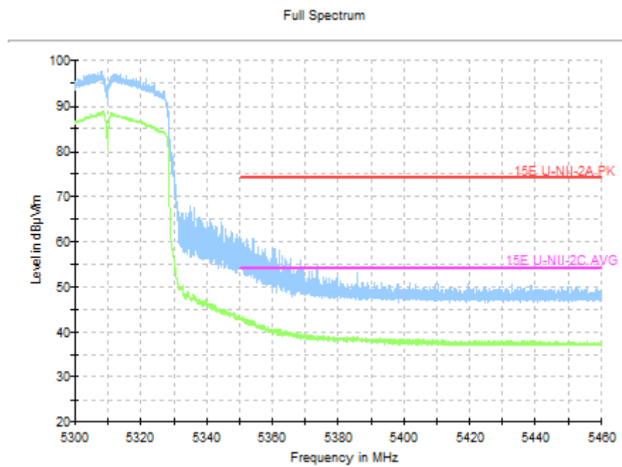
Fig.43 Band Edges (802.11n-HT40, 5310MHz)
