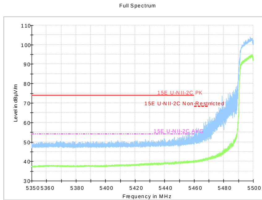
Fig.48 Band Edges (802.11ac-HT20, 5500MHz)
