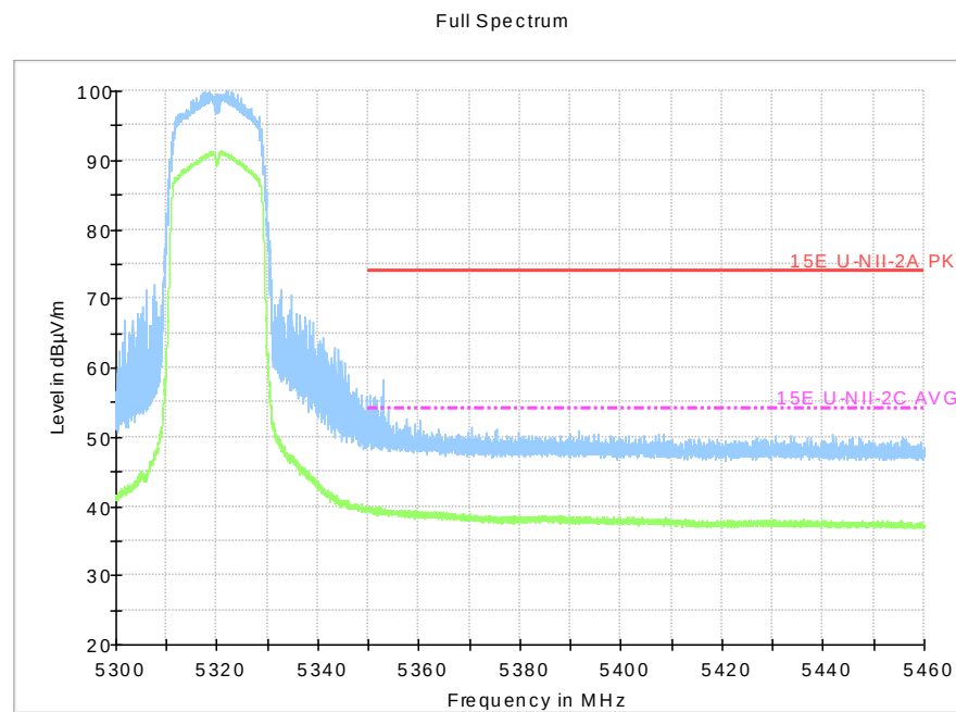
Fig.47 Band Edges (802.11ac-HT20, 5320MHz)
