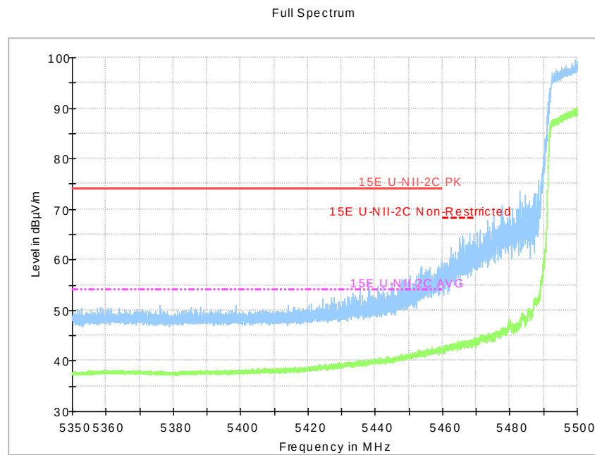
Fig.52 Band Edges (802.11ac-HT40, 5510MHz)
