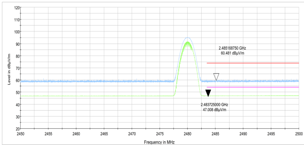
Fig.18. Frequency Band Edges: 8DPSK, Channel 78, 2.45 GHz - 2.50GHz
