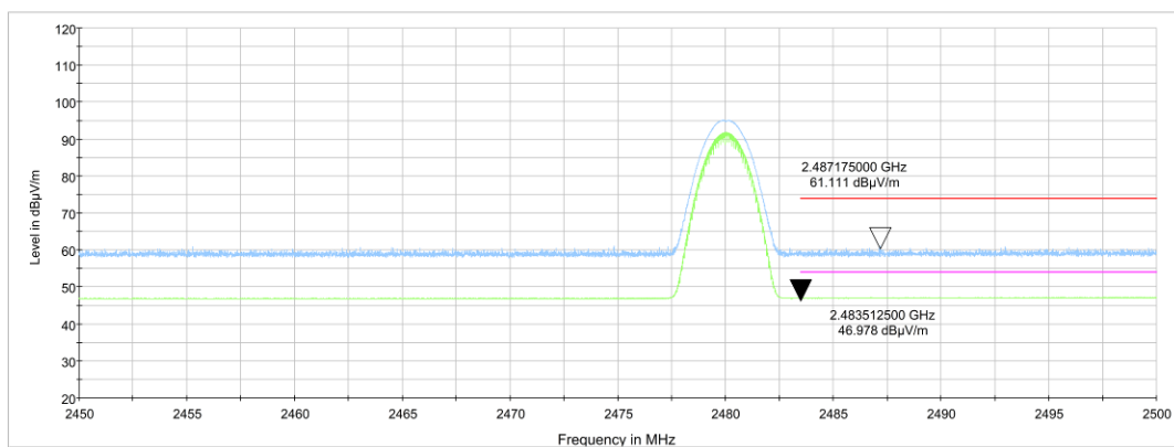
Fig.16. Frequency Band Edges: \pi/4 DQPSK, Channel 78, 2.45 GHz - 2.50GHz
