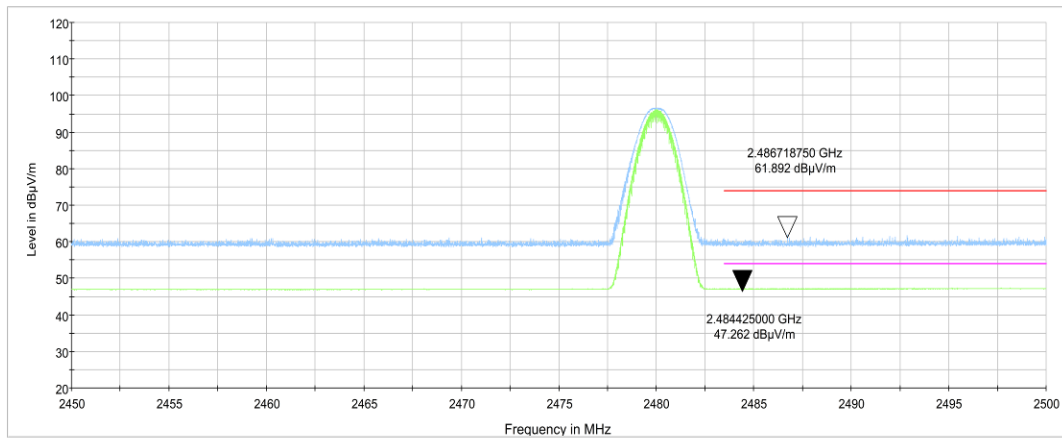
Fig.14. Frequency Band Edges: GFSK, Channel 78, ch11, 2.45 GHz - 2.50GHz
