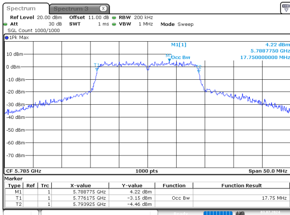
n20_5785MHz_Chain 0
