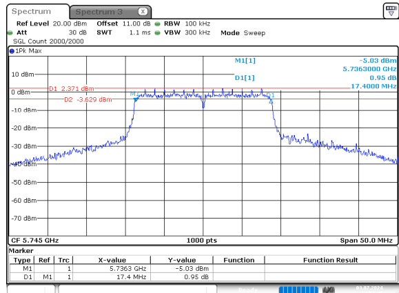
n20_5745MHz_Chain 0
