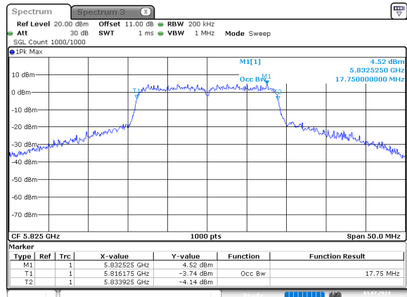
n20_5825MHz_Chain 0
