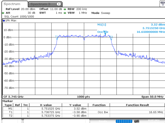
a_5745MHz_Chain 0
