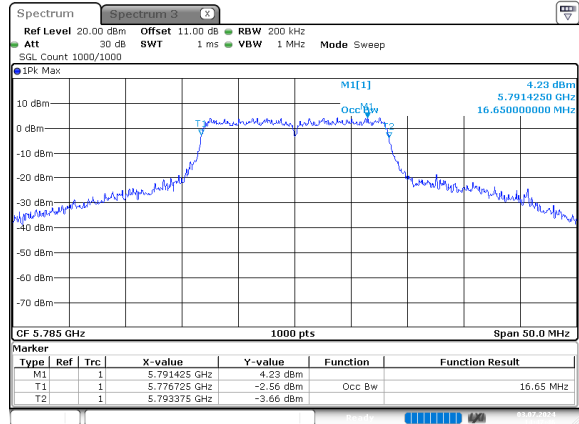
a_5785MHz_Chain 0
