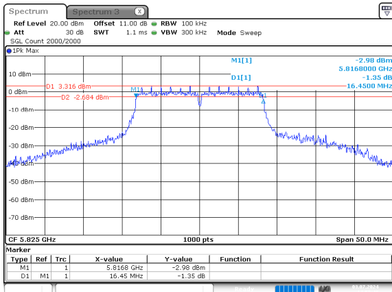
a_5825MHz_Chain 0
