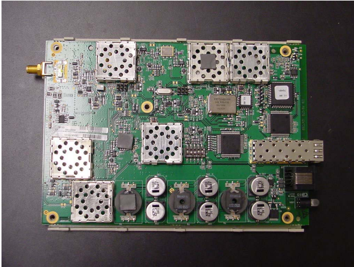
Digivance ICS 1900 MHz Digital Remote Unit Open Top View
