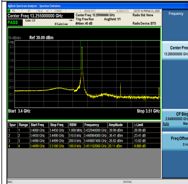
NTNV-n77(3450-3550)-PC2-30-60-L-CP-QPSK- Edge_1RB_Left-PASS
