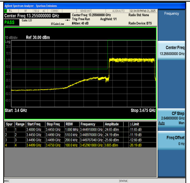
NTNV-n77(3450-3550)-PC2-30-25-L-CP-QPSK- Outer_Full-PASS
