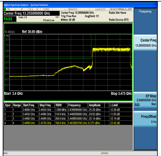
NTNV-n77(3450-3550)-PC2-30-25-L-DFT-BPSK- Outer_Full-PASS
