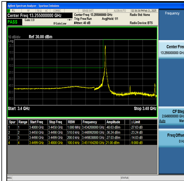
NTNV-n77(3450-3550)-PC2-30-30-L-DFT-BPSK- Edge_1RB_Left-PASS
