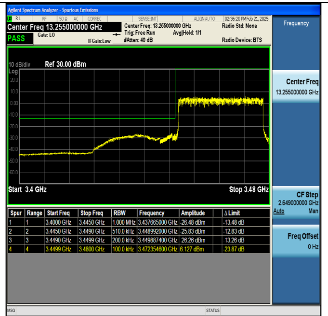
NTNV-n77(3450-3550)-PC2-30-30-L-DFT-BPSK- Outer_Full-PASS
