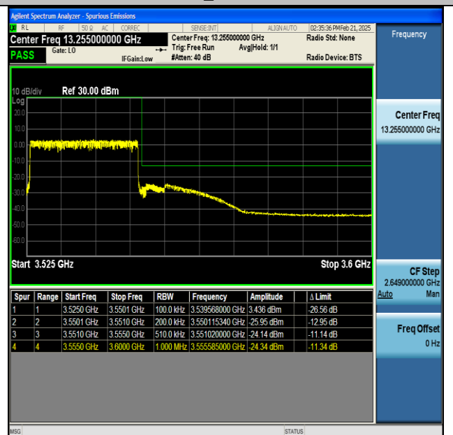
NTNV-n77(3450-3550)-PC2-30-25-H-CP-QPSK- Outer_Full-PASS
