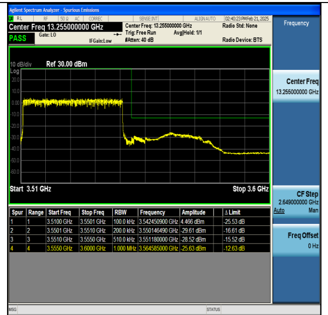
NTNV-n77(3450-3550)-PC2-30-40-H-DFT-BPSK- Outer_Full-PASS
