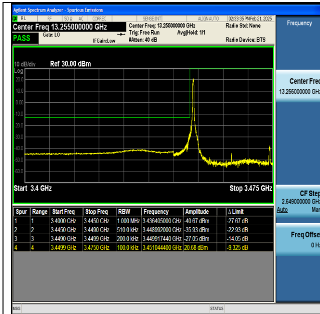
NTNV-n77(3450-3550)-PC2-30-25-L-DFT-BPSK- Edge_1RB_Left-PASS
