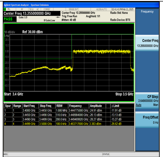
NTNV-n77(3450-3550)-PC2-30-50-L-DFT-BPSK- Outer_Full-PASS
