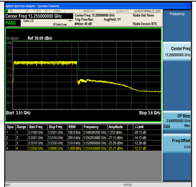
NTNV-n77(3450-3550)-PC2-30-40-H-CP-QPSK- Outer_Full-PASS
