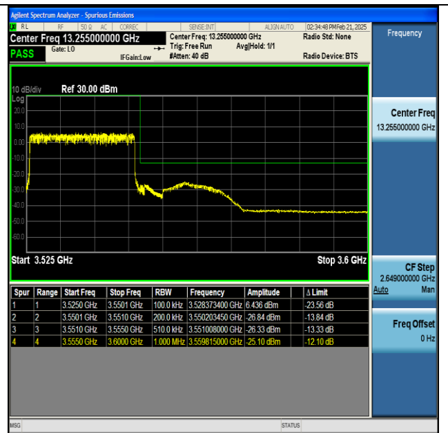
NTNV-n77(3450-3550)-PC2-30-25-H-DFT-BPSK- Outer_Full-PASS
