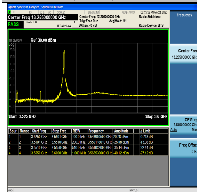
NTNV-n77(3450-3550)-PC2-30-25-H-CP-QPSK- Edge_1RB_Right-PASS
