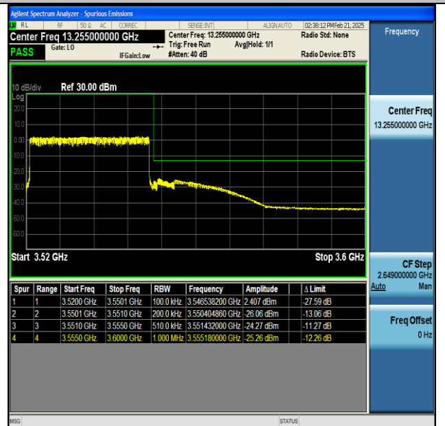
NTNV-n77(3450-3550)-PC2-30-30-H-CP-QPSK- Outer_Full-PASS
