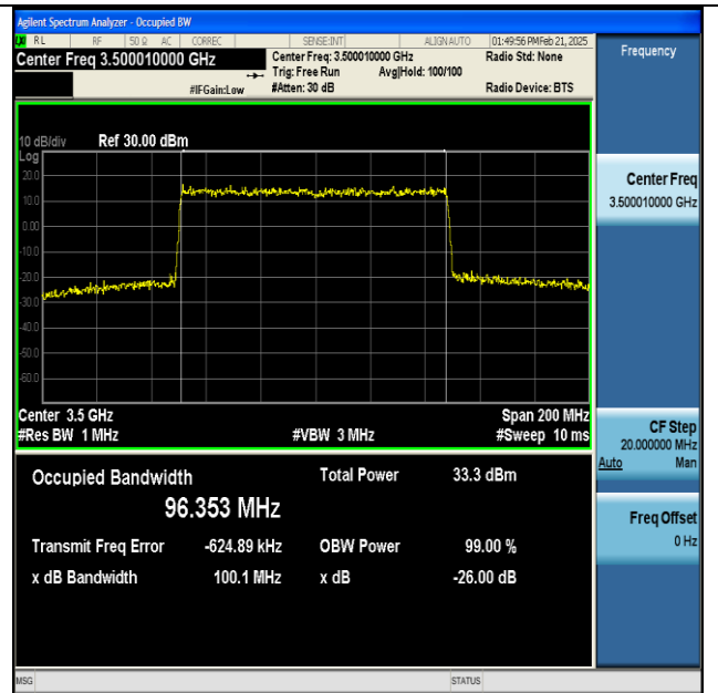
NTNV-n77(3450-3550)-PC2-30-100-H-DFT-16QAM- Outer_Full-Ant1-PASS
