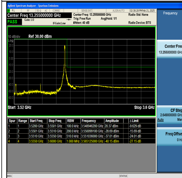
NTNV-n77(3450-3550)-PC2-30-30-H-CP-QPSK- Edge_1RB_Right-PASS
