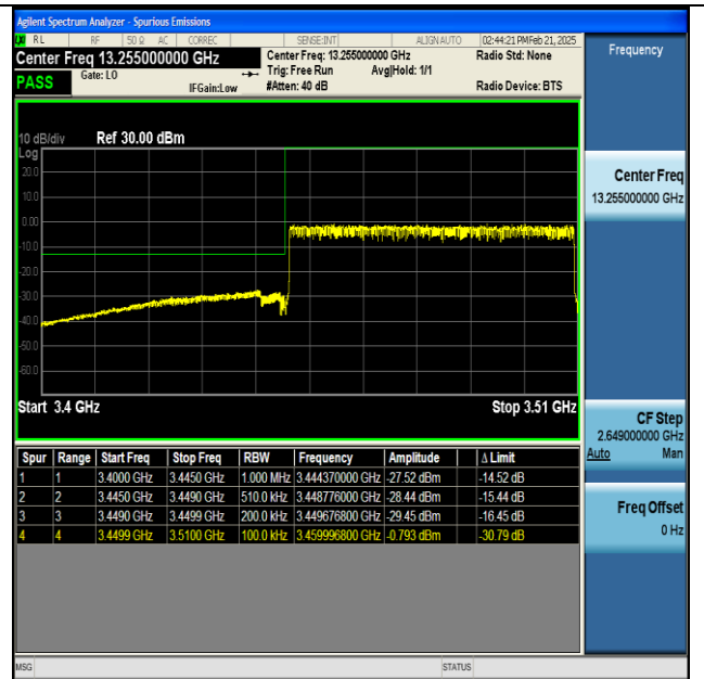
NTNV-n77(3450-3550)-PC2-30-60-L-DFT-BPSK- Outer_Full-PASS
