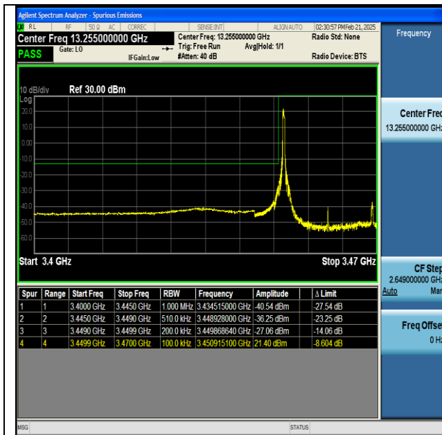
NTNV-n77(3450-3550)-PC2-30-20-L-DFT-BPSK- Edge_1RB_Left-PASS
