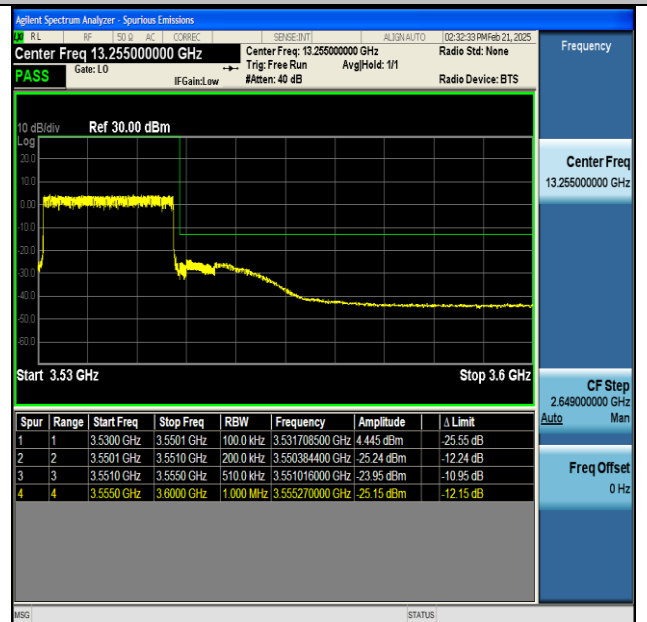
NTNV-n77(3450-3550)-PC2-30-20-H-CP-QPSK- Outer_Full-PASS
