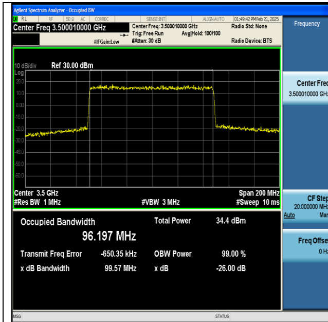
NTNV-n77(3450-3550)-PC2-30-100-H-DFT-QPSK- Outer_Full-Ant1-PASS
