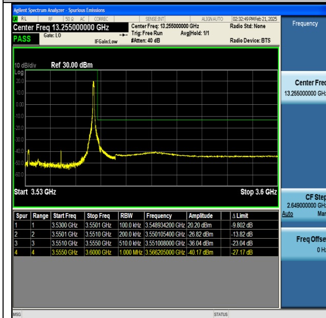
NTNV-n77(3450-3550)-PC2-30-20-H-CP-QPSK- Edge_1RB_Right-PASS
