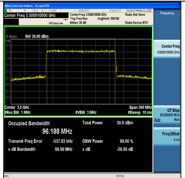
NTNV-n77(3450-3550)-PC2-30-100-H-DFT-256QAM- Outer_Full-Ant1-PASS
