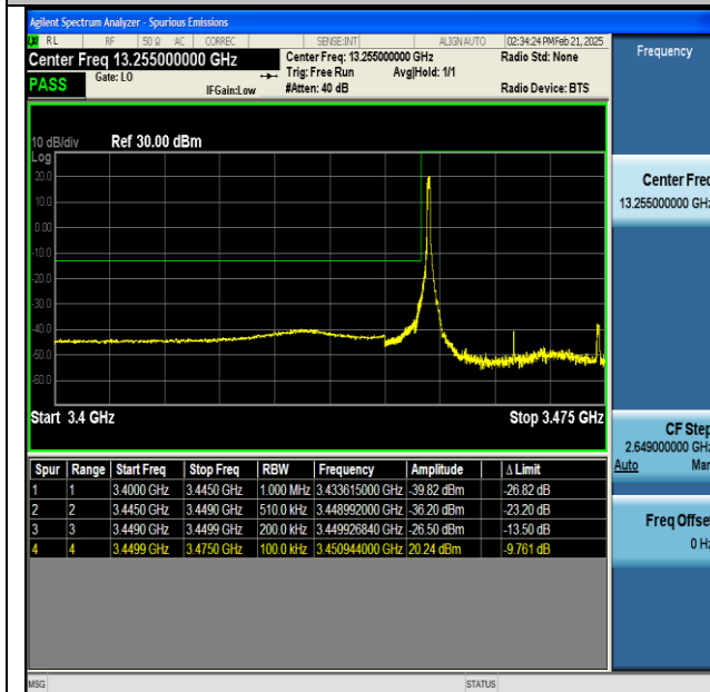
NTNV-n77(3450-3550)-PC2-30-25-L-CP-QPSK- Edge_1RB_Left-PASS
