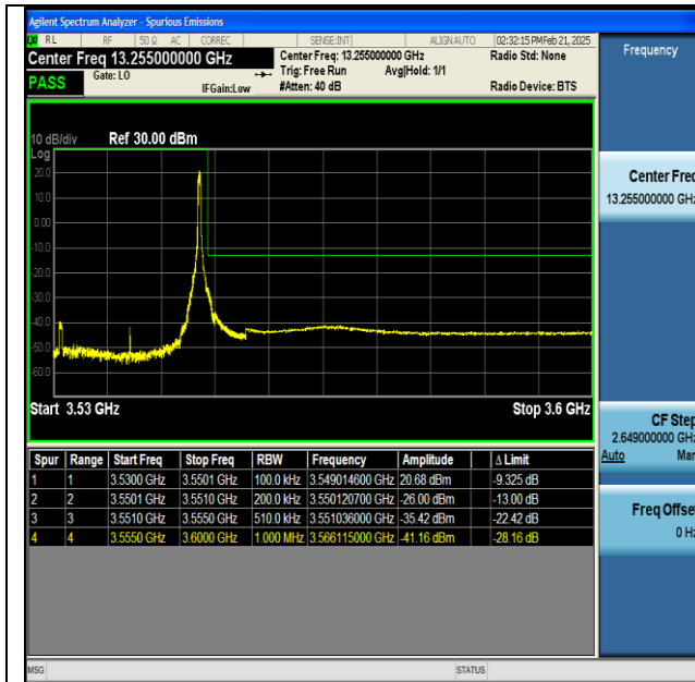
NTNV-n77(3450-3550)-PC2-30-20-H-DFT-BPSK- Edge_1RB_Right-PASS
