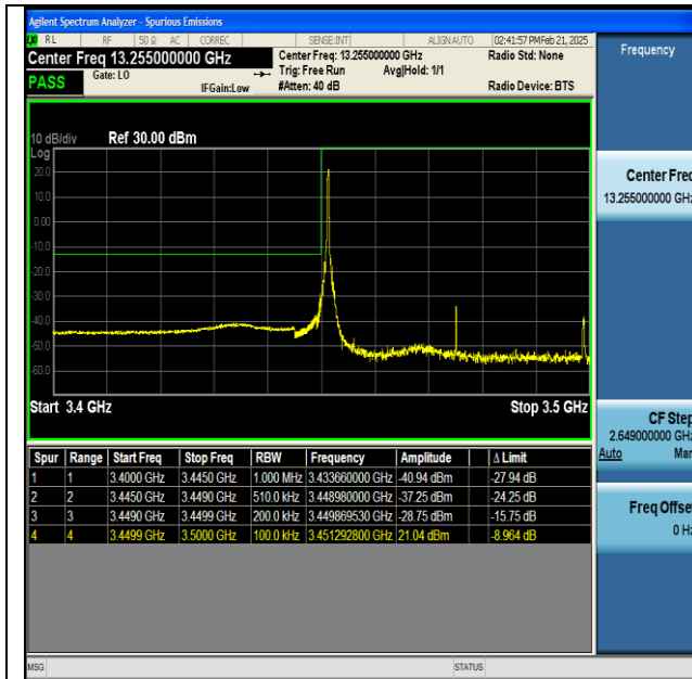
NTNV-n77(3450-3550)-PC2-30-50-L-DFT-BPSK- Edge_1RB_Left-PASS
