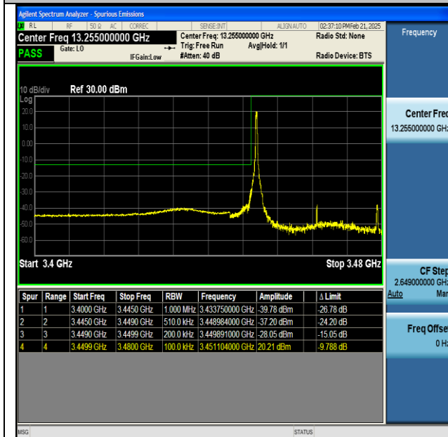
NTNV-n77(3450-3550)-PC2-30-30-L-CP-QPSK- Edge_1RB_Left-PASS
