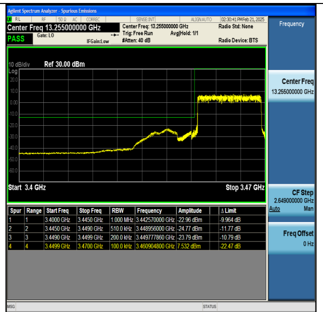
NTNV-n77(3450-3550)-PC2-30-20-L-DFT-BPSK- Outer_Full-PASS
