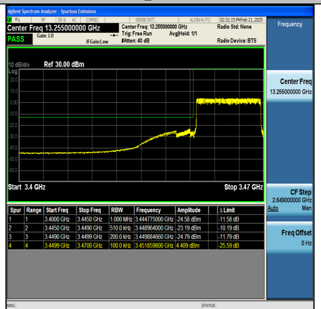
NTNV-n77(3450-3550)-PC2-30-20-L-CP-QPSK- Outer_Full-PASS
