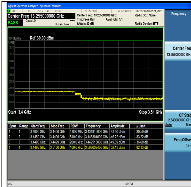
NTNV-n77(3450-3550)-PC2-30-60-L-DFT-BPSK- Edge_1RB_Left-PASS
