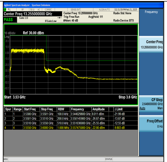
NTNV-n77(3450-3550)-PC2-30-20-H-DFT-BPSK- Outer_Full-PASS
