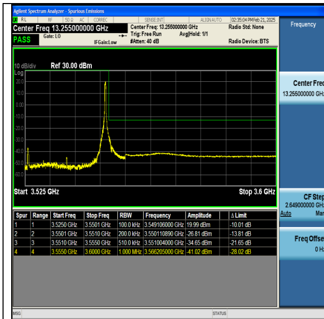
NTNV-n77(3450-3550)-PC2-30-25-H-DFT-BPSK- Edge_1RB_Right-PASS
