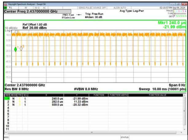
802.11g
