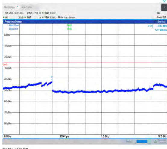
1-N41-PC1-30-100-H-1-DFT-QPSK-Edge_1RB_Left -1@0-3000-18000-Ant1-7471.50--41.64--25-PASS
