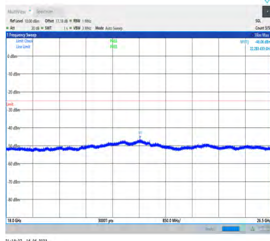
1-N41-PC1-30-100-H-1-DFT-QPSK-Edge_1RB_Left- 1@0-18000-26500-Ant1-22283.43--46.06--25-PASS
