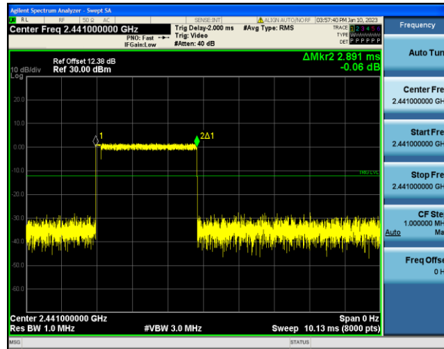
3DH1-Ant1-Hop-0.390-320
