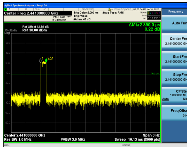
3DH3-Ant1-Hop-1.643-160
