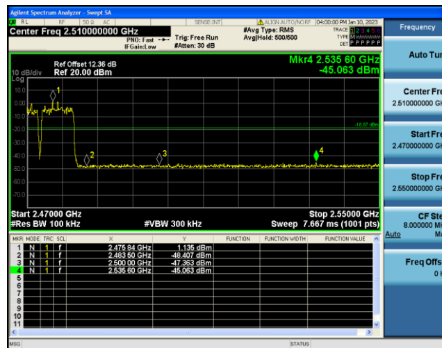
3DH5-Ant1-High-Hop_2480-1.14
