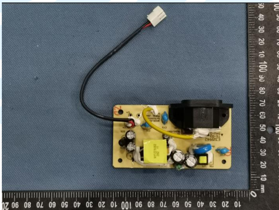
EUT Photo _ Build-in Power 3
