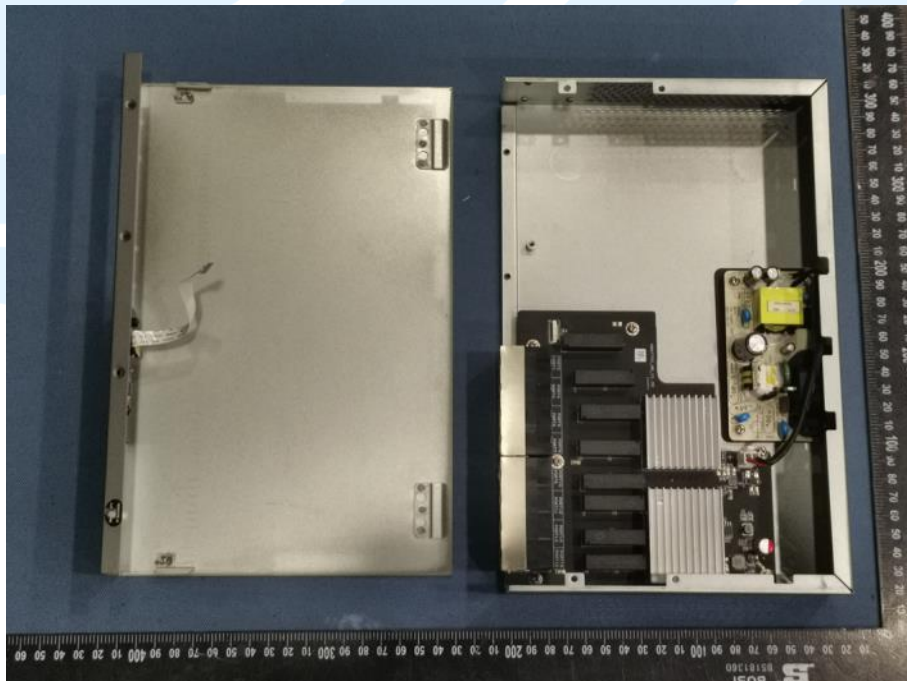
EUT Photo _ Configuring the Build-in Power 2
