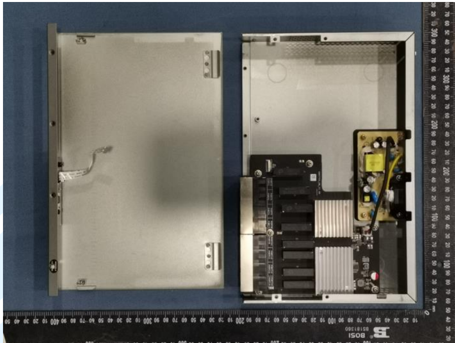
EUT Photo _ Configuring the Build-in Power 3
