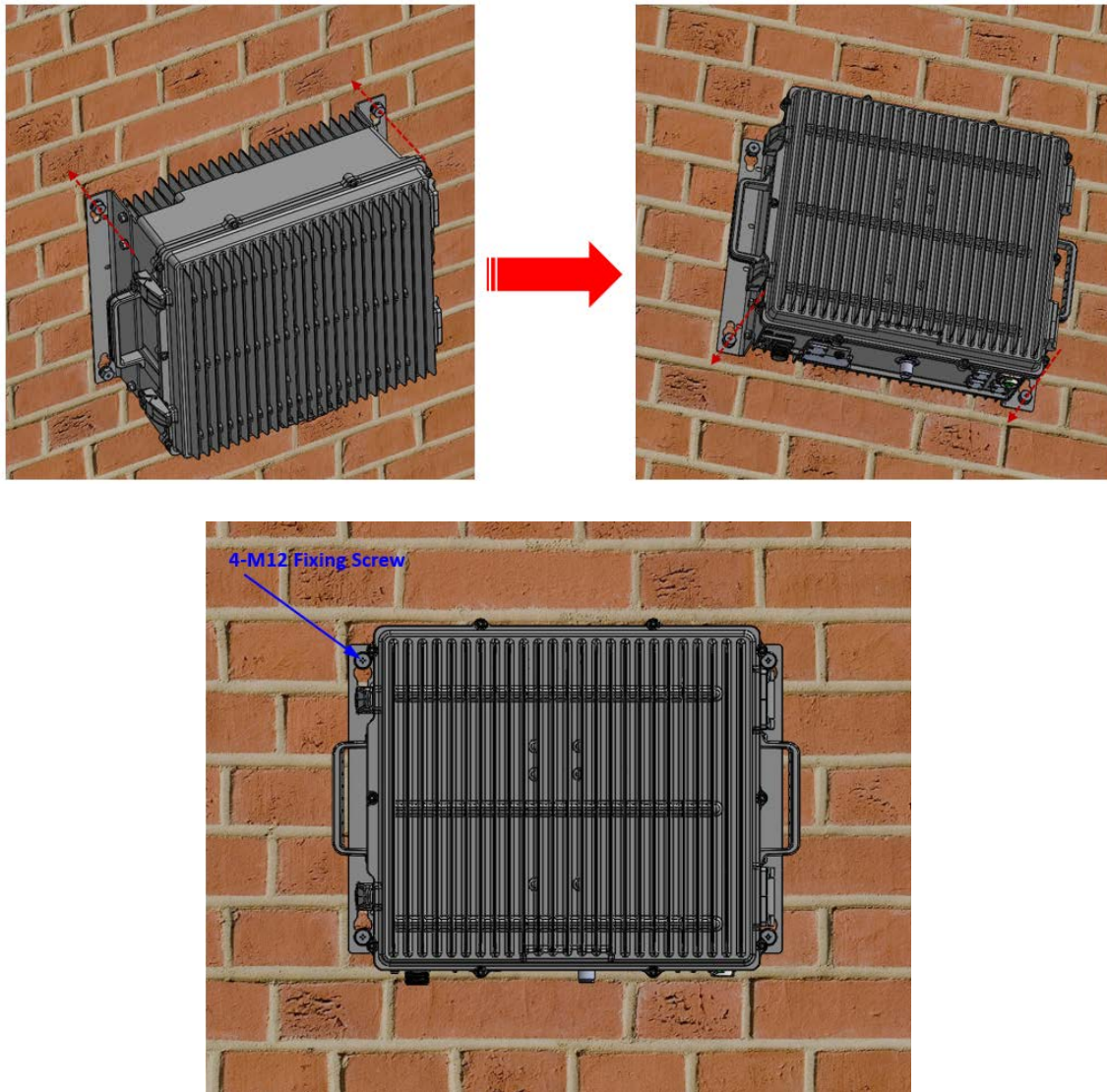
Figure 4.4 – Installation Procedure
