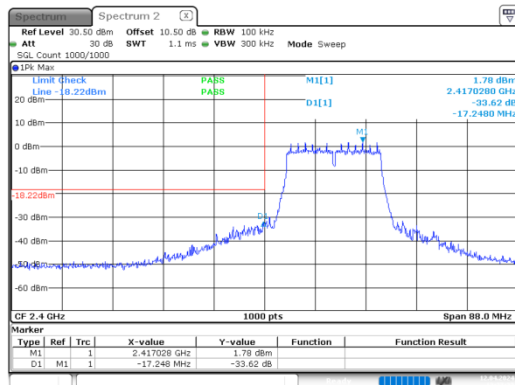
g_2412MHz
