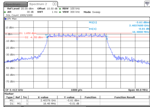
g_2412MHz
