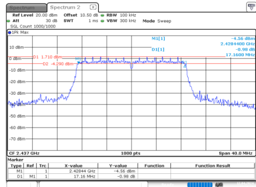
n20_2437MHz
