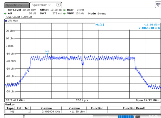
g_2412MHz
