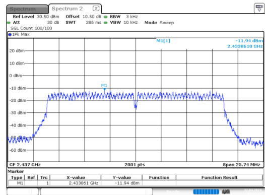
n20_2437MHz
