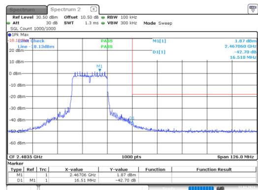
n20_2462MHz_
