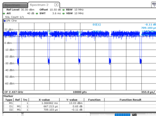
n20_2437MHz
