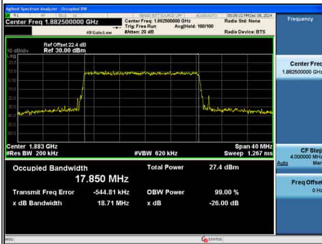
OCC_5G_n25_15KHz_256QAM_20M CH376500
