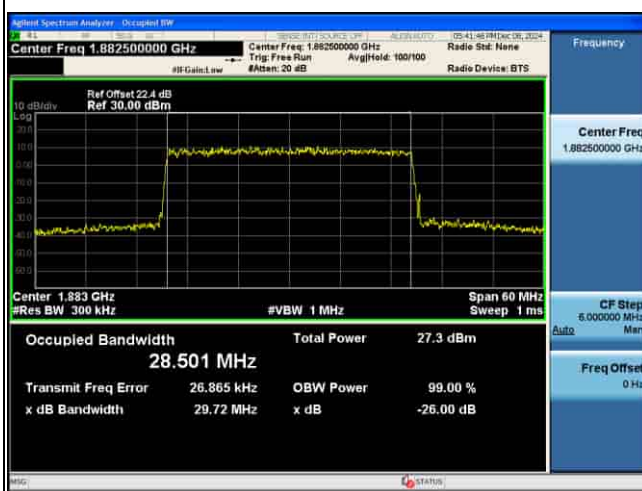
OCC_5G_n25_15KHz_256QAM_30M CH376500
