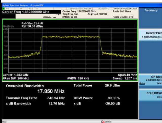
OCC_5G_n25_15KHz_16QAM_20M CH376500
