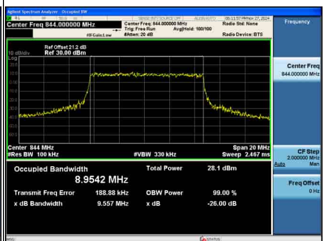
OCC_5G_n26_15KHz_64QAM_10M CH168800
