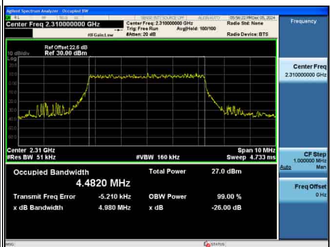
OCC_5G_n30_15KHz_256QAM_5M CH462000
