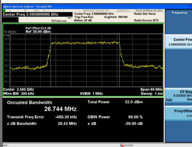
OCC_5G_n41_30KHz_..PI2-BPSK_30M CH519000
