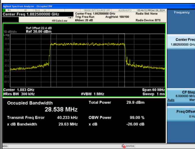
OCC_5G_n25_15KHz_16QAM_30M CH376500
