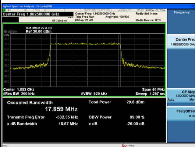
OCC_5G_n25_15KHz_64QAM_20M CH376500
