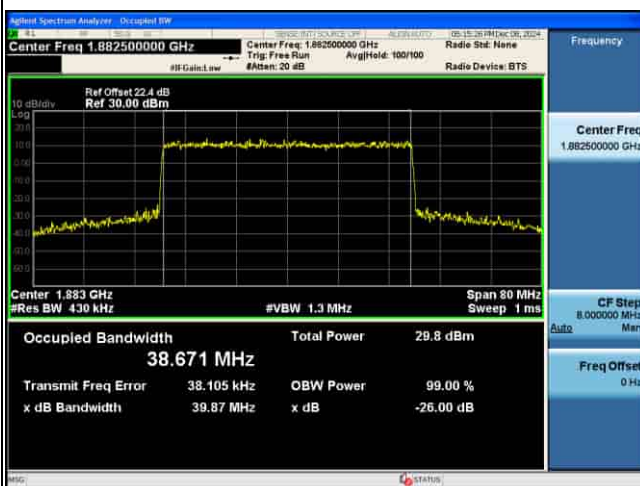
OCC_5G_n25_15KHz_16QAM_40M CH376500
