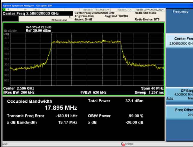
OCC_5G_n41_30KHz_..PI2-BPSK_20M CH535998
