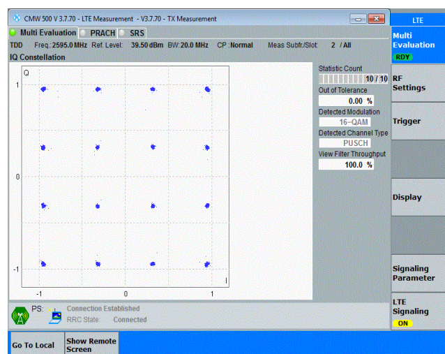
Band41-20MHz-16QAM-40640-100RB#0
