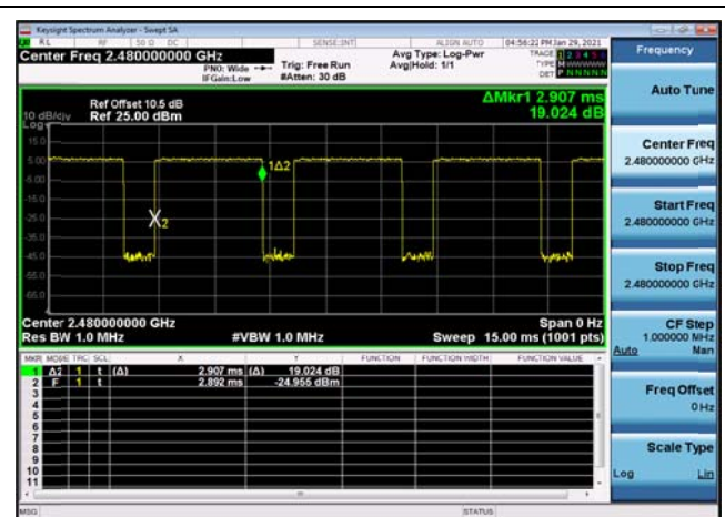
8DPSK,2480,3DH5,Transmission Time
