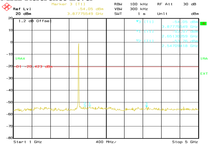
Conducted Emissions. 802.11n, Frequency 2412 MHz Emission Level, 1 GHz -> 5 GHz
