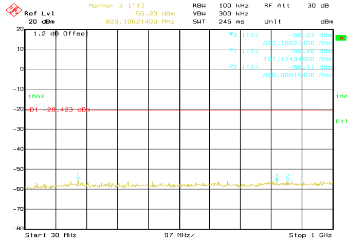
Conducted Emissions. 802.11n, Frequency 2412 MHz Emission Level, 30 MHz -> 1 GHz
