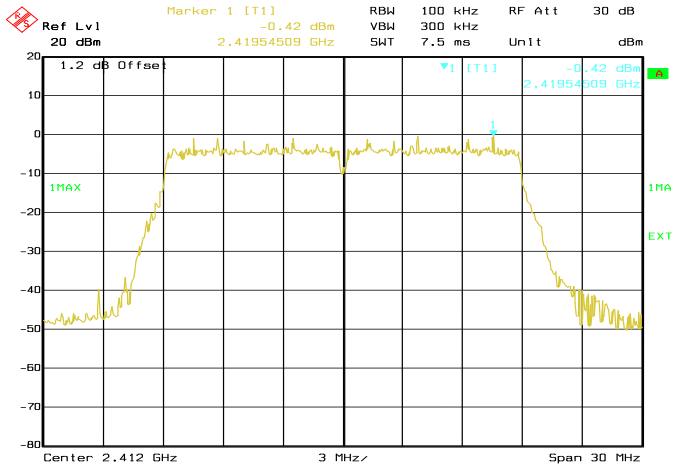
Conducted Emissions. 802.11n, Frequency 2412 MHz Reference Level
