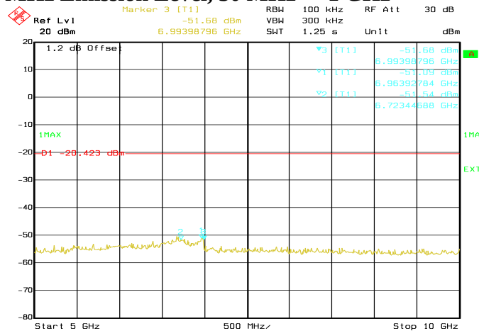
Conducted Emissions. 802.11n, Frequency 2412 MHz Emission Level, 5 GHz -> 10 GHz
