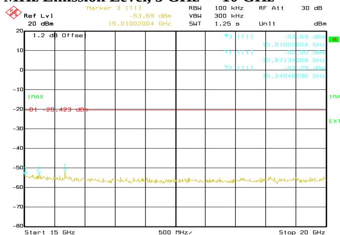
Conducted Emissions. 802.11n, Frequency 2412 MHz Emission Level, 15 GHz -> 20 GHz
