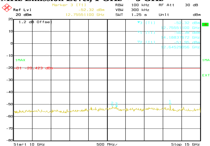
Conducted Emissions. 802.11n, Frequency 2412 MHz Emission Level, 10 GHz -> 15 GHz
