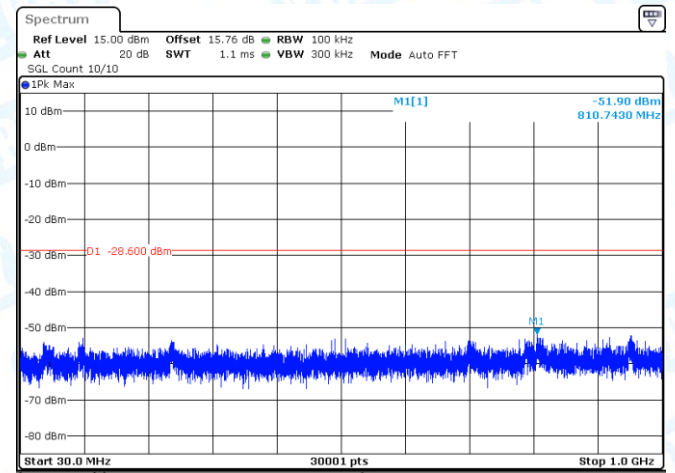
11AX20-CDD-Ant2-2412-0~Reference-PASS
