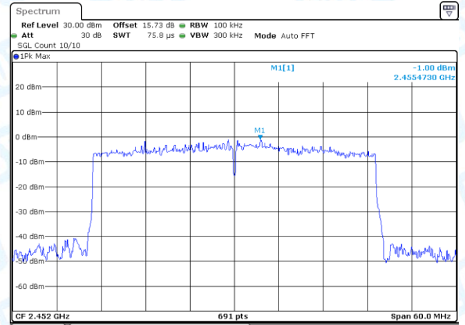
11AX40-CDD-Ant2-2452-0~Reference-PASS
