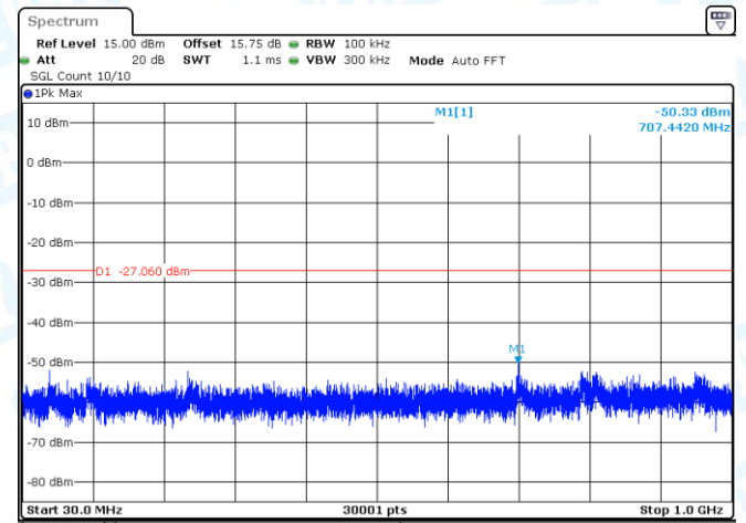
11AX40-CDD-Ant2-2437-0~Reference-PASS
