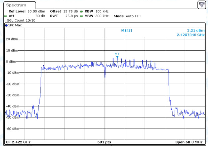
11AX40-CDD-Ant2-2422-0~Reference-PASS
