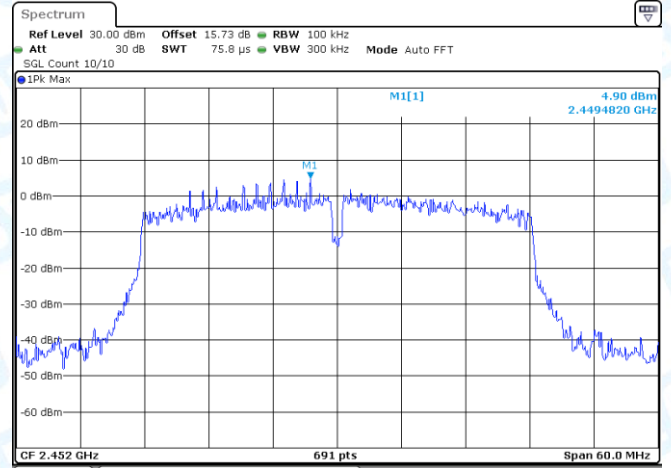
11N40-CDD-Ant2-2452-0~Reference-PASS
