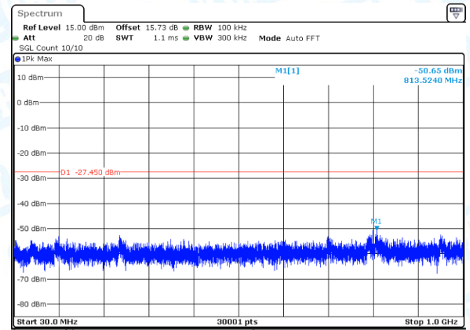
11AX20-CDD-Ant2-2462-0~Reference-PASS
