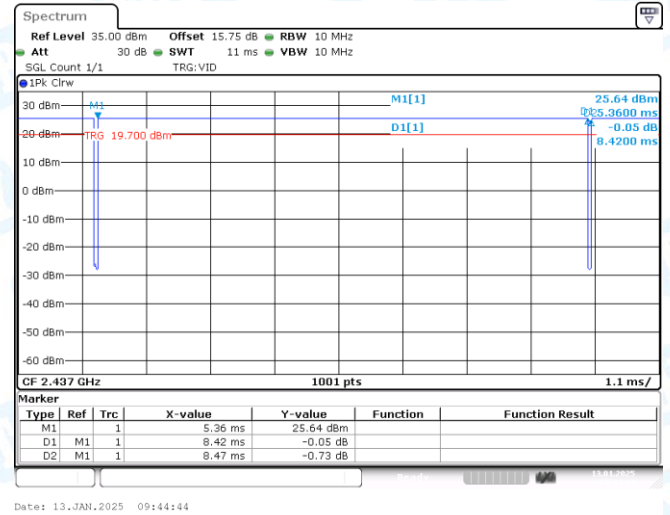
NTNV-11B-Ant2-2437
