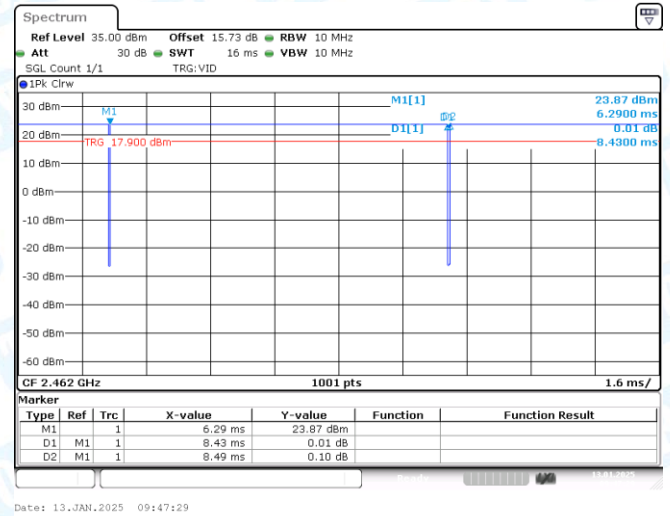
NTNV-11B-Ant2-2462
