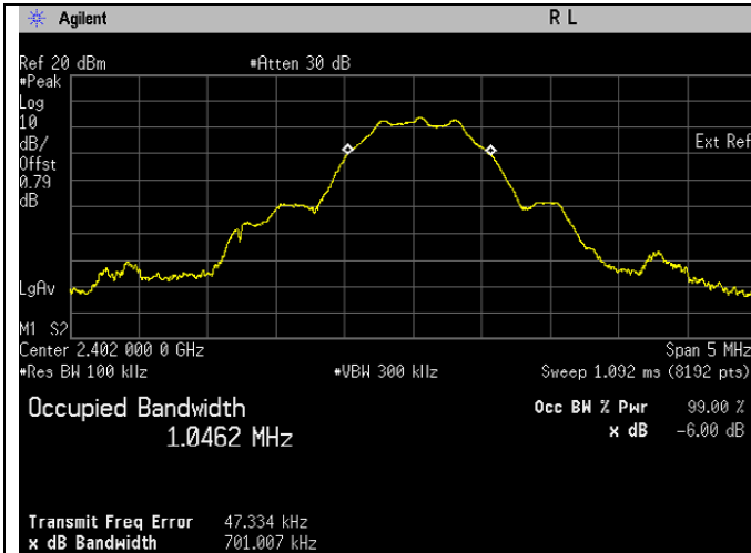
6dB Bandwidth. Bluetooth LE Frequency 2402 MHz
