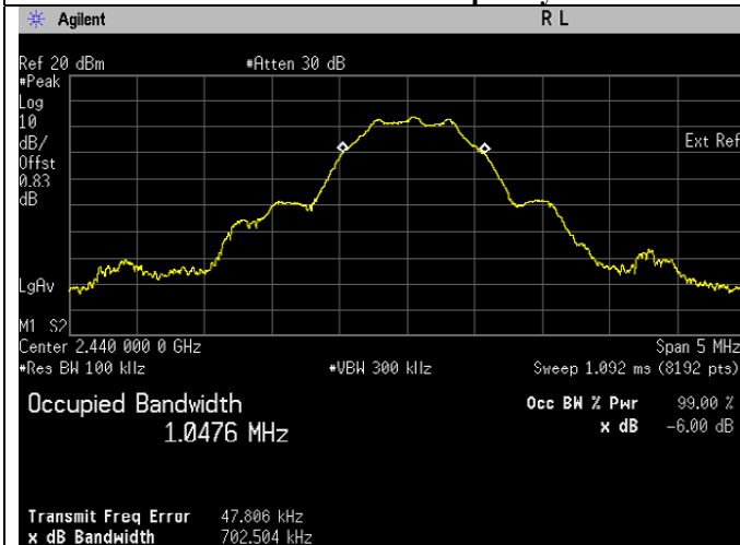
6dB Bandwidth. Bluetooth LE Frequency 2440 MHz
