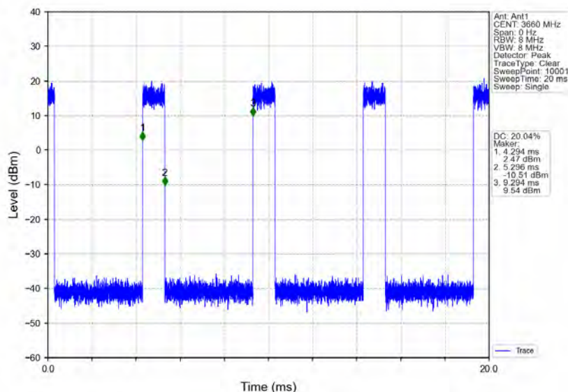
n78d_30kHz_MIMO_NTNV_80MHz_CP-OFDM_16_QAM_3660MHz_Inner_Full
