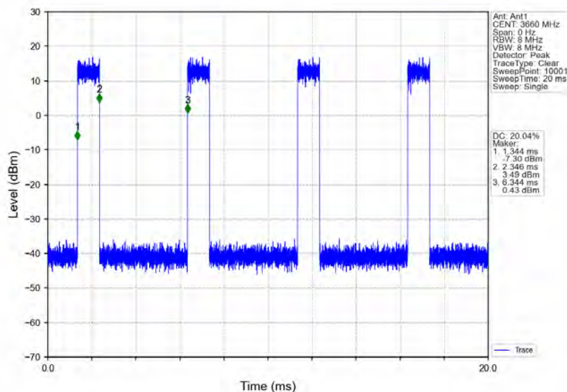
n78d_30kHz_MIMO_NTNV_80MHz_CP-OFDM_QPSK_3660MHz_Inner_Full
